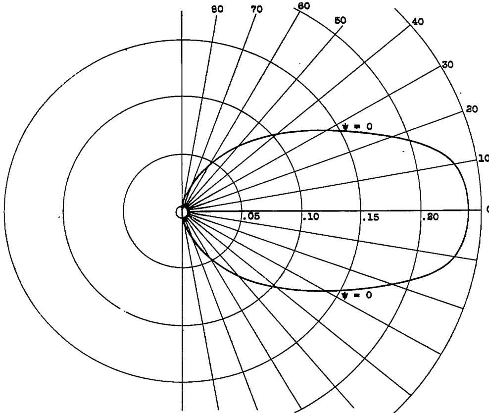
Figure 14.- The compressible flow in \tau , \theta -plane. \epsilon = 1/2 ; M_1 = 0.6 .
