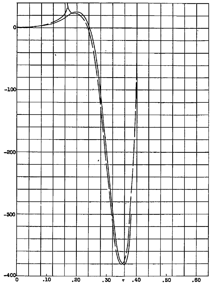
Figure 8.- F - \frac{21}{2}(\tau) ; \gamma = 1.405 .
