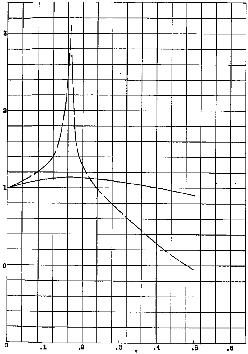
Figure 7.- F - \frac{3}{2}(\tau) ; \gamma = 1.405 .
