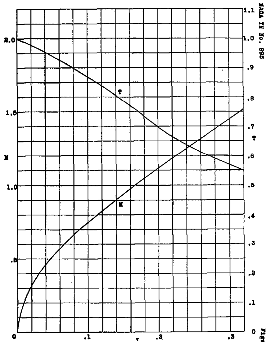
Figure 4.- T(\tau) ; X(\tau) ; \gamma = 1.405 .
