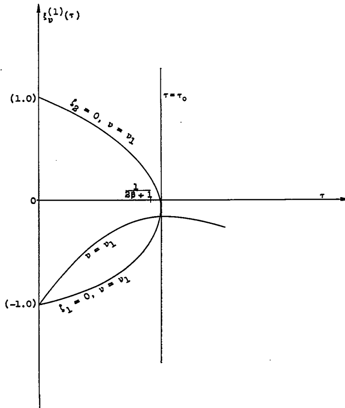
Figure 16.- The behavior of the integral-curve; i_p^{(1)}(\tau) .
