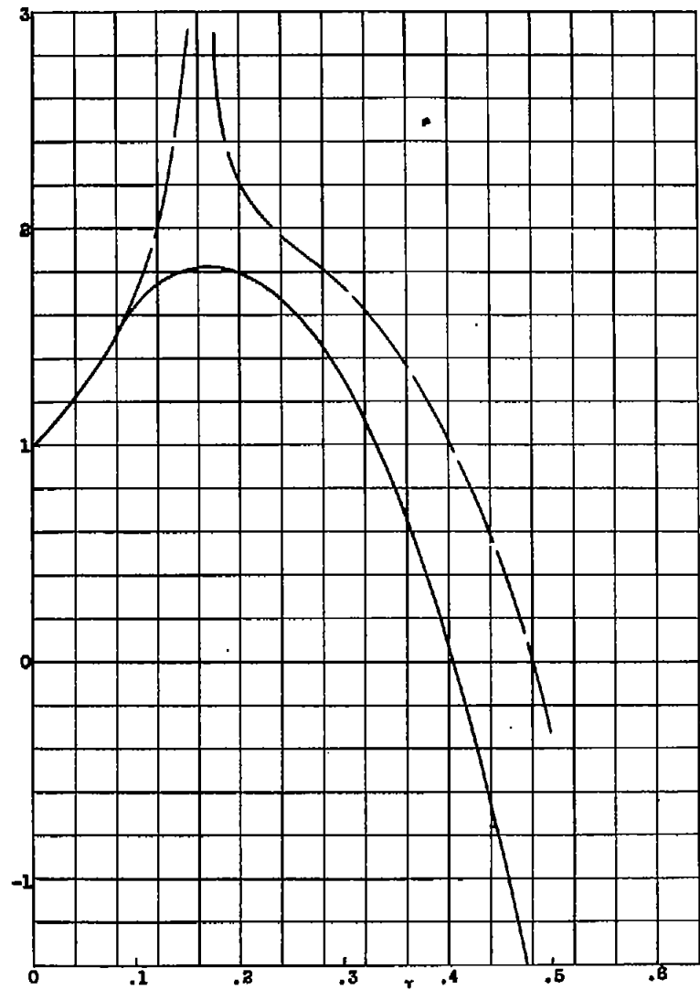
Figure 10.- \bar{F} - 3/2(\tau) ; \gamma = 1.405 .
