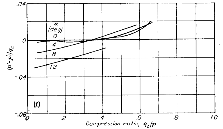
(b) Collar at distance x_C behind static orifices. D_c=1.43D ; x_N=13.6D . (d) Angle of attack for hemispherical nose. Prandtl-type tube. x_N=3D ; r_S=10D_S ; reference 22. (f) Angle of attack for semiellipsoidal nose. x_N=3.5D ; D_S=0.25D ; r_S=20D_S ; reference 23.
