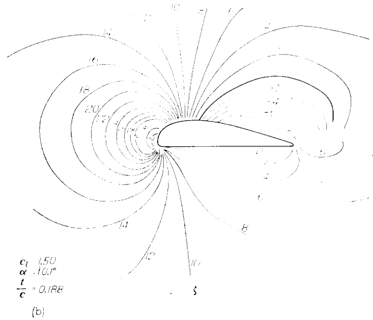
(a) RAF 30 symmetrical airfoil (reference 27). (b) Nonsymmetrical airfoil (reference 26). FIGURE 6.—Contours of equal static-pressure defect \Delta p/q and angle of flow relative to airfoil chord \zeta from measurements.
