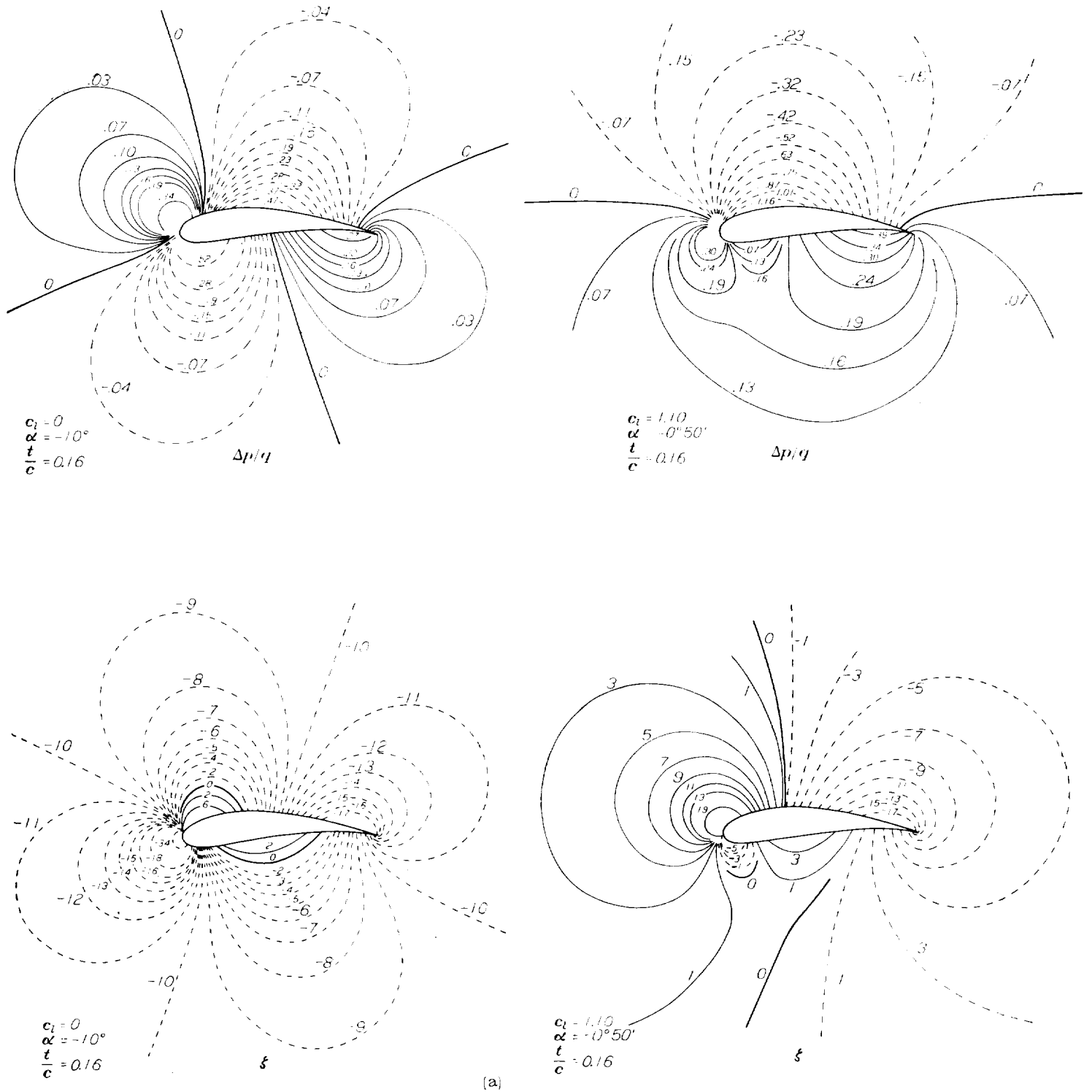
(a) Contours of equal static-pressure defect \Delta p/q and equal angle of flow relative to airfoil chord \xi . Data from reference 28. FIGURE 5.—The field of flow about a Joukowski airfoil from calculations. Variation with c_l .
