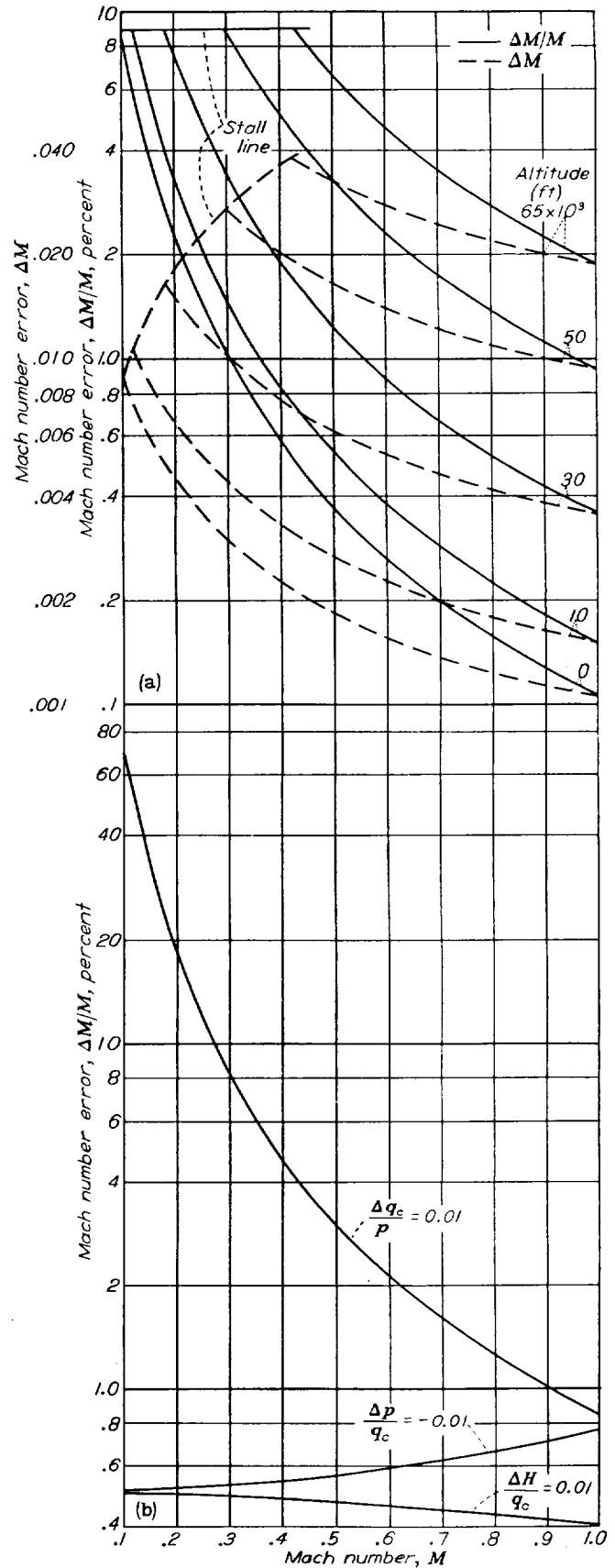
(a) Error in q_c and p of 0.5 inch of water. (b) Error in H , q_c , and p of 1 percent.
