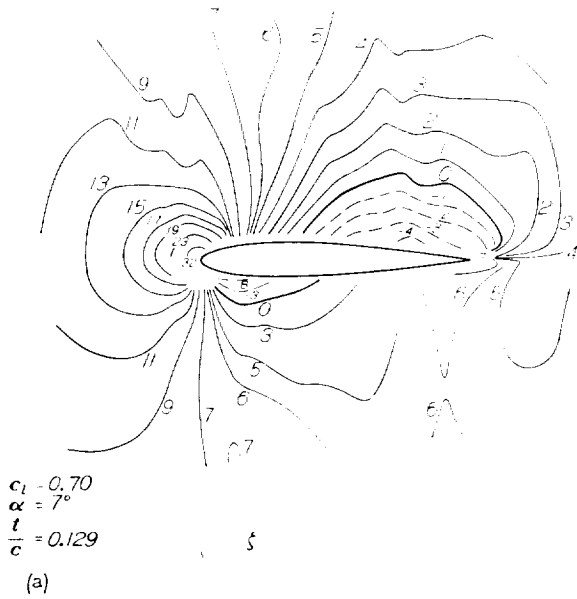
(a) RAF 30 symmetrical airfoil (reference 27). (b) Nonsymmetrical airfoil (reference 26). FIGURE 6.—Contours of equal static-pressure defect \Delta p/q and angle of flow relative to airfoil chord \zeta from measurements.
