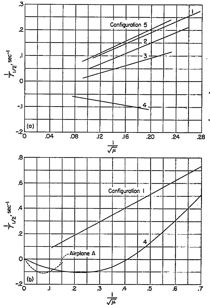
(a) Basic configurations. Data taken from table II for altitudes of 0 and 50,000 feet.
