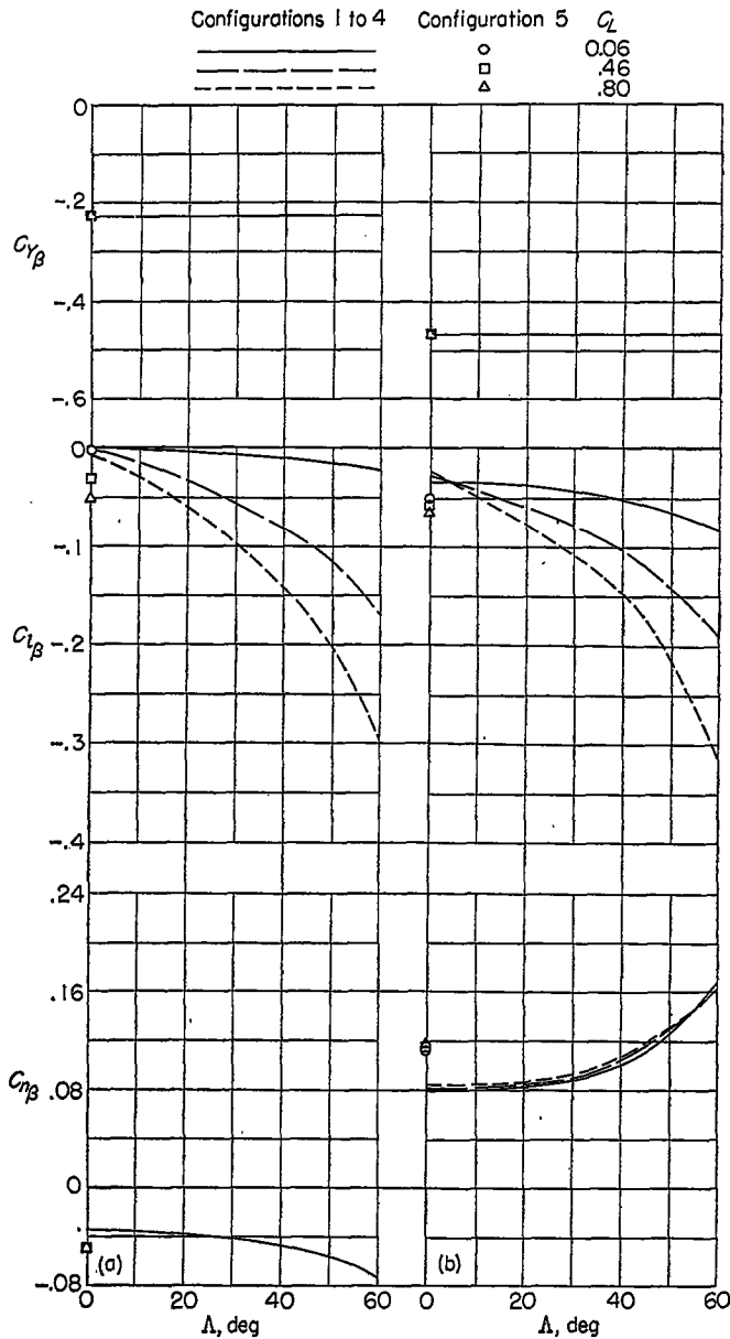
(a) Vertical tail off. (b) Complete airplane.
