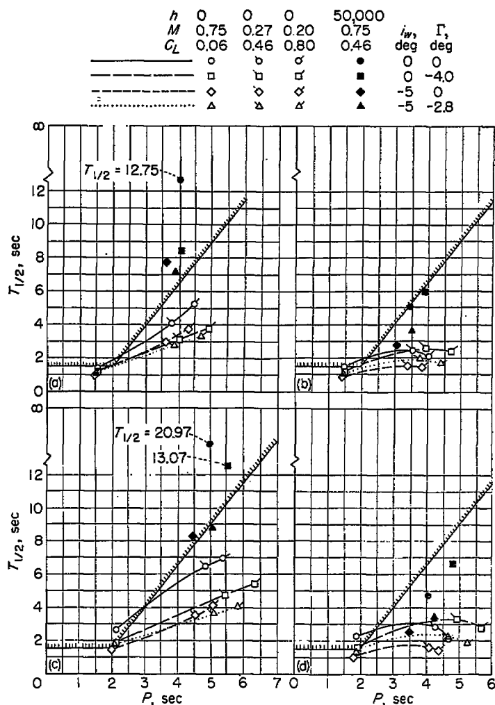
(a) Basic mass characteristics. (b) Reduced K_{x_0} . (c) Increased K_{z_0} . (d) Reduced K_{x_0} and increased K_{z_0} . FIGURE 11.—Stability of modified configuration derived from configuration 5.
