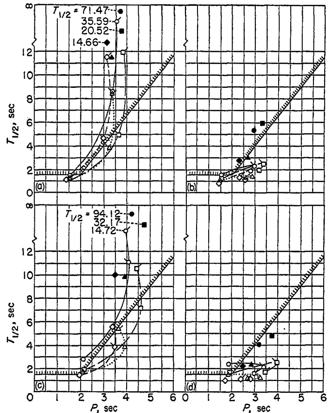
(a) Basic mass characteristics. (b) Reduced K_{x_0} . (c) Increased K_{z_0} . (d) Reduced K_{x_0} and increased K_{z_0} .
