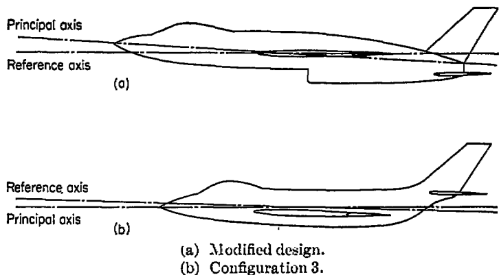
(a) Modified design. (b) Configuration 3. FIGURE 12.—Illustration of profile of an airplane designed to have positive inclination of the principal longitudinal axis of inertia and comparison with profile of configuration 3 which is representative of many designs.
