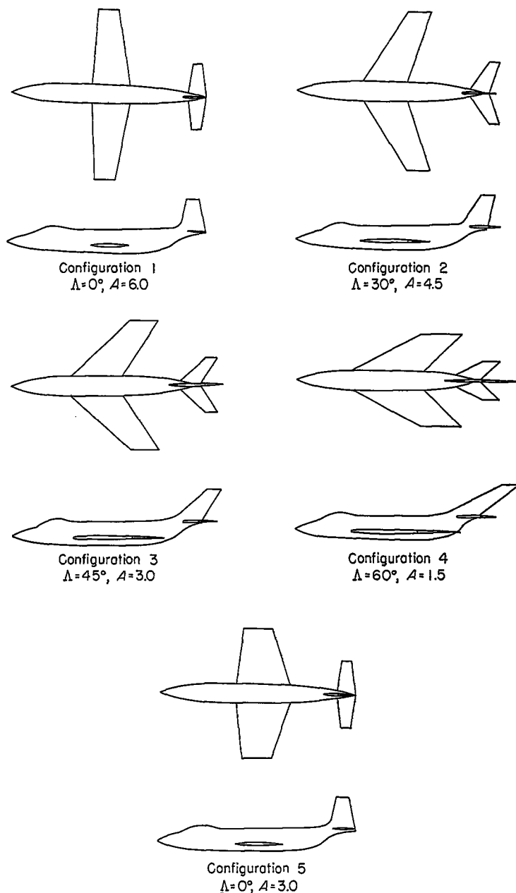
FIGURE 2.—Basic configurations for which calculations were made.
