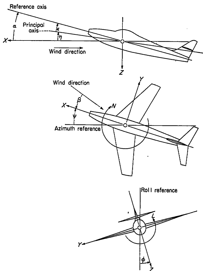
FIGURE 1.—The stability system of axes. Arrows indicate positive directions of moments, forces, and angles. This system of axes is defined as an orthogonal system having the origin at the center of gravity and in which the Z -axis is in the plane of symmetry and perpendicular to the relative wind, the X -axis is in the plane of symmetry and perpendicular to the Z -axis, and the Y -axis is perpendicular to the plane of symmetry. At a constant angle of attack, these axes are fixed in the airplane.
