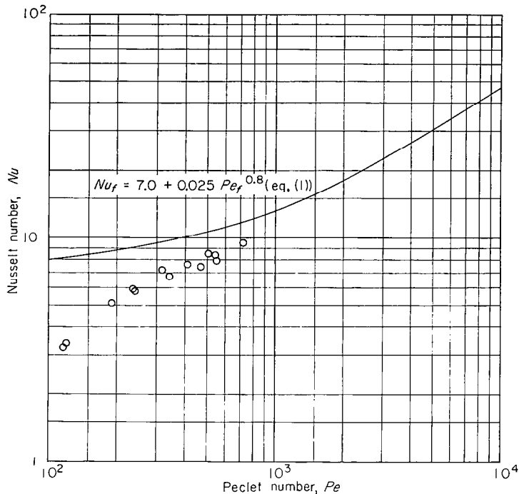
FIGURE 17.—Data of English and Barrett (refs. 9 and 10) for fully developed heat transfer to mercury in round tubes.
