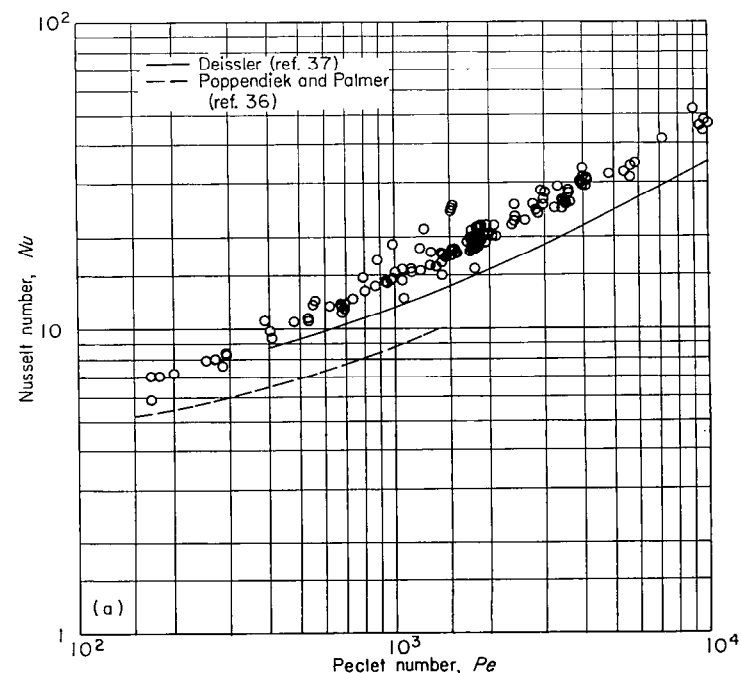
(a) Length-diameter ratio x/D , 4.6.
