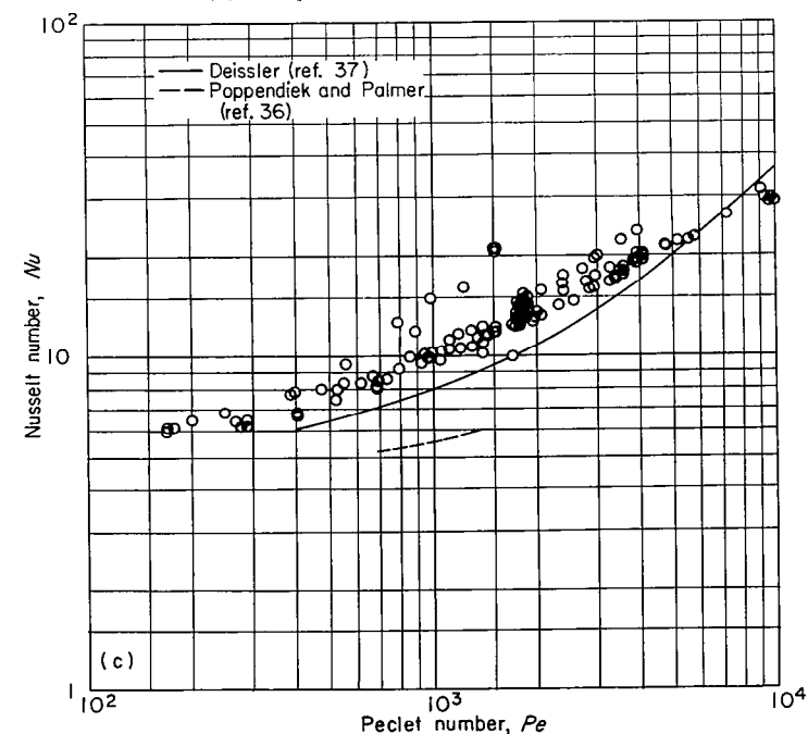
(c) Length-diameter ratio x/D , 23.
