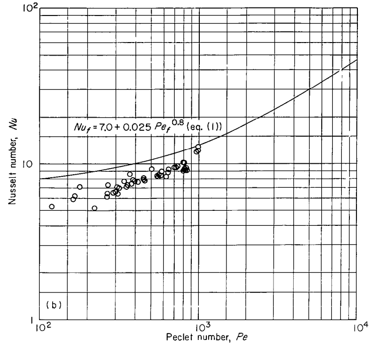
(b) Test section B (length-diameter ratio l/D , 98).
