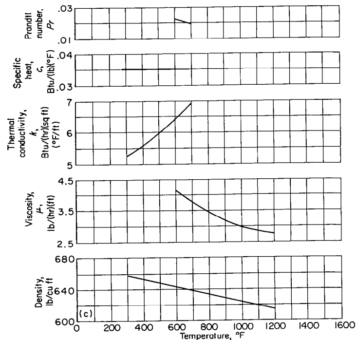
(c) Lead-bismuth eutectic.
