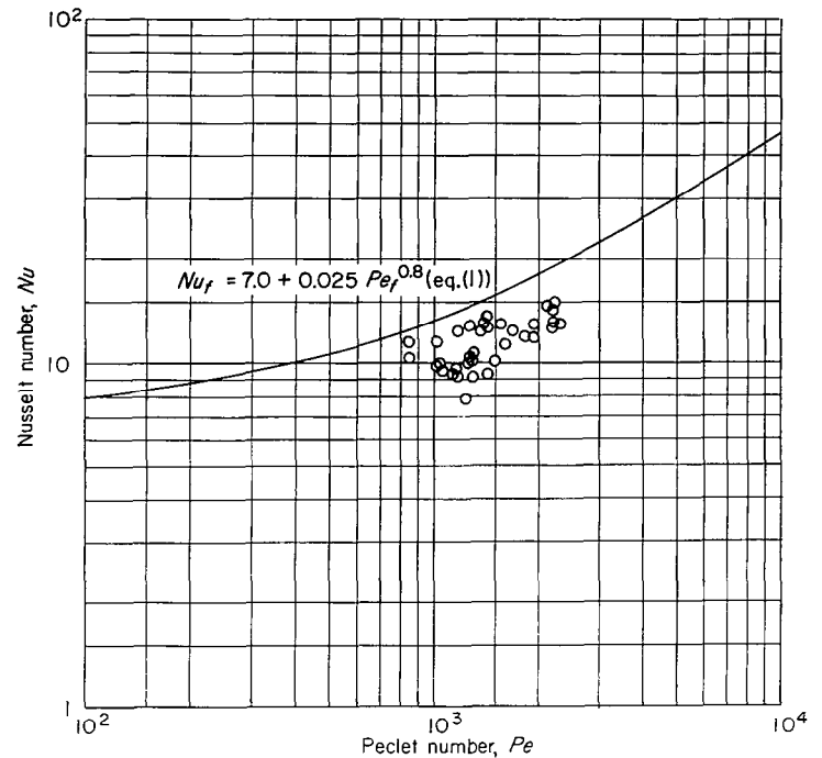
FIGURE 8.—Reevaluated data of Styrikovich and Semenovker (ref. 1) for fully developed heat transfer to mercury in round tubes.
