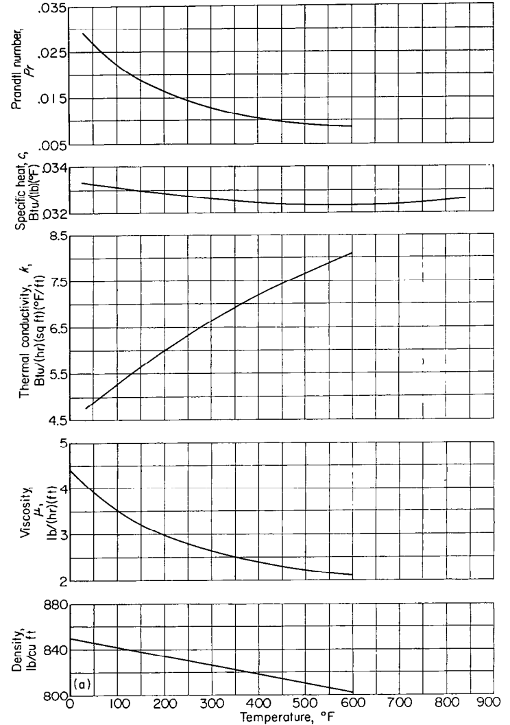
(a) Mercury.
