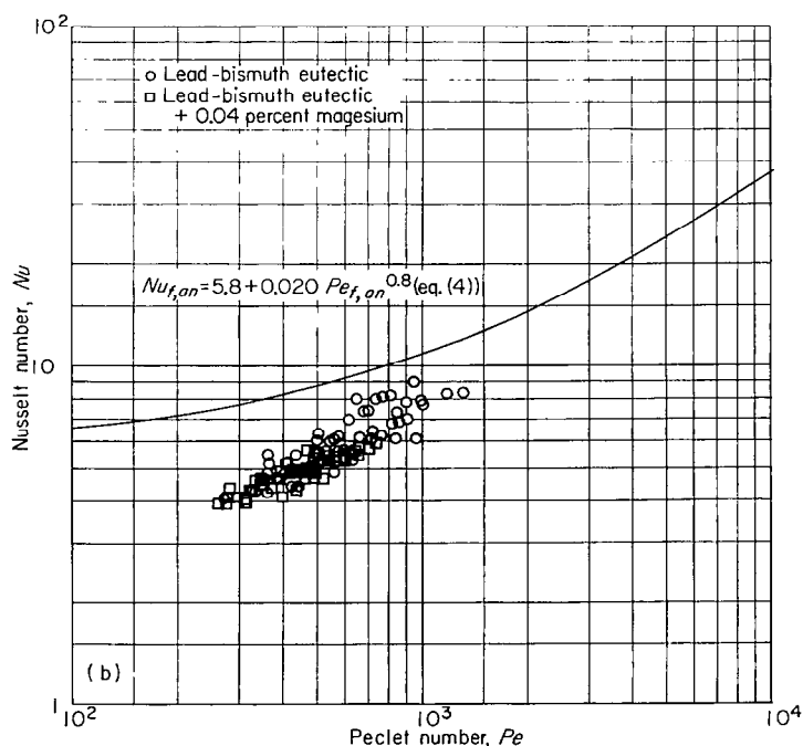
(b) In annuli; length-diameter ratio l/D , 322.
