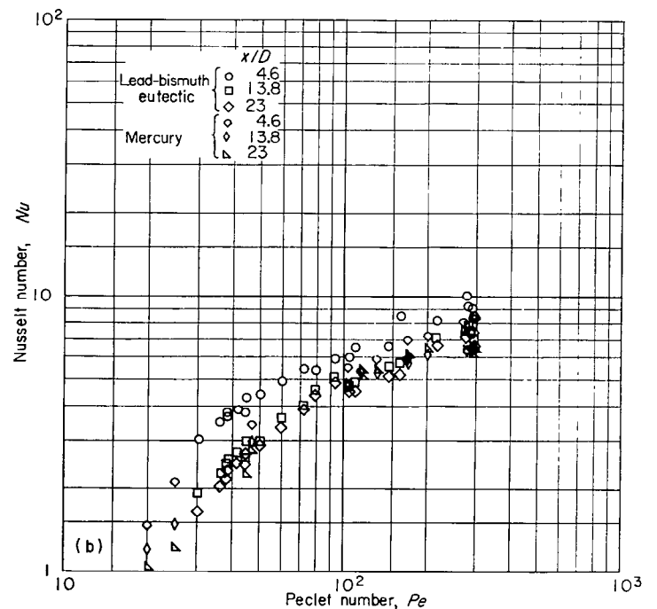
(b) Entrance-region heat transfer.
