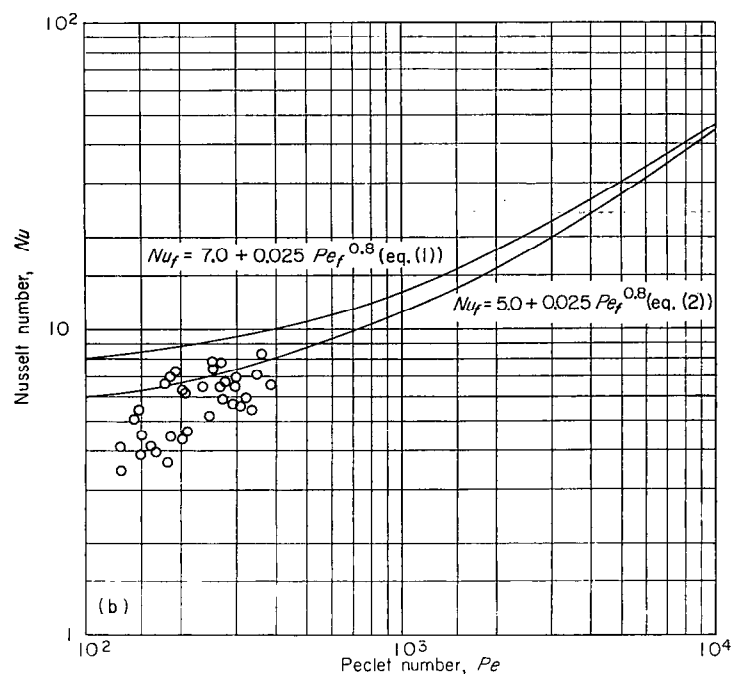
(b) With small sodium additions.
