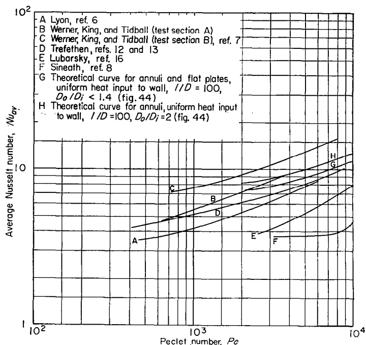
FIGURE 47.—Comparison of measured and predicted average Nusselt numbers in annuli and between flat plates with uniform heat input to wall.
