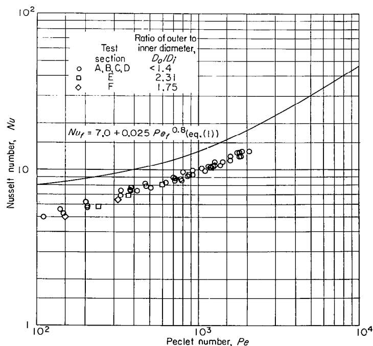
FIGURE 21.—Reevaluated data of Trefethen (refs. 12 and 13) for fully developed heat transfer to mercury in round tubes.
