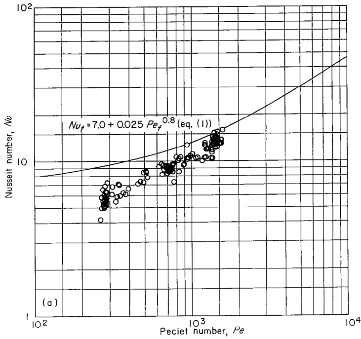
(a) Test section A (length-diameter ratio l/D , 111).
