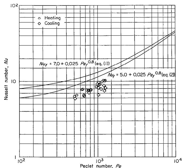
FIGURE 9.—Data of Gilliland, Musser, and Page (refs. 2 and 3) for average heat transfer to mercury in round tubes. Length-diameter ratio l/D : heating section, 45; cooling section, 160.
