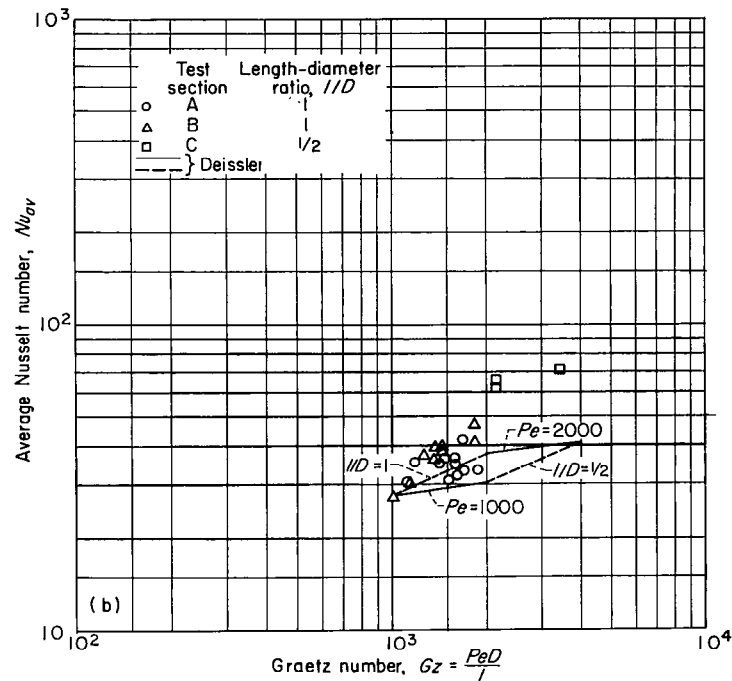
(b) 1000 < \text{Peclet number} < 2000 .
