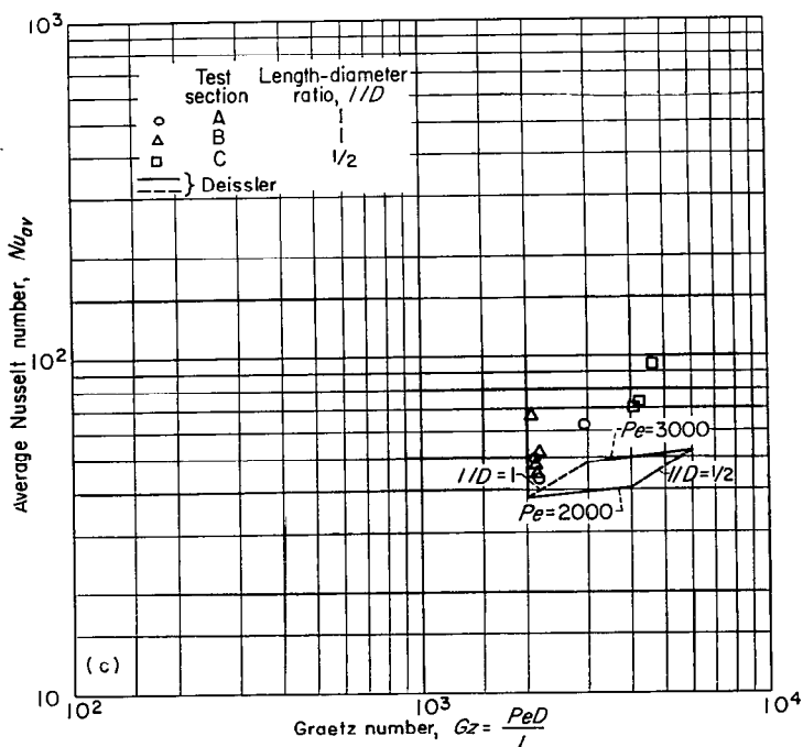
(c) 2000 < \text{Peclet number} < 3000 .
