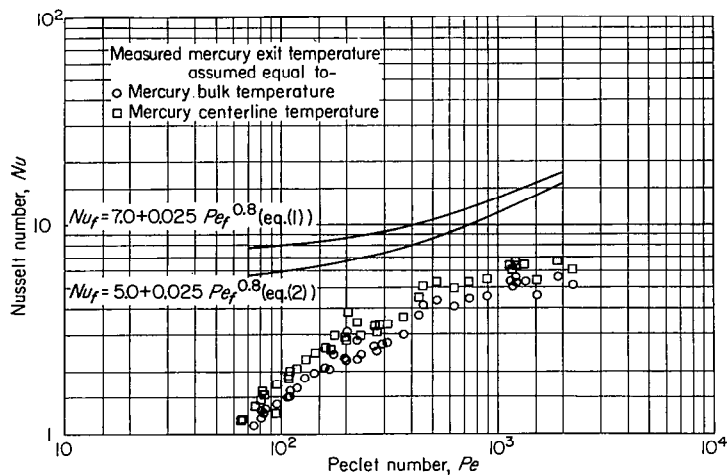
FIGURE 11.—Reevaluated data of Bailey, Cope, and Watson (ref. 5) for fully developed heat transfer to mercury in round tubes.
