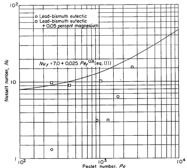
FIGURE 14.—Reevaluated data of Untermeyer for fully developed heat transfer to lead-bismuth eutectic, with and without magnesium addition, in round tubes.
