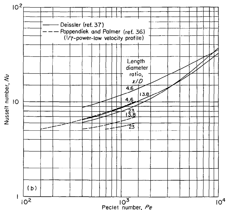
(b) Nusselt number against Peclet number.
