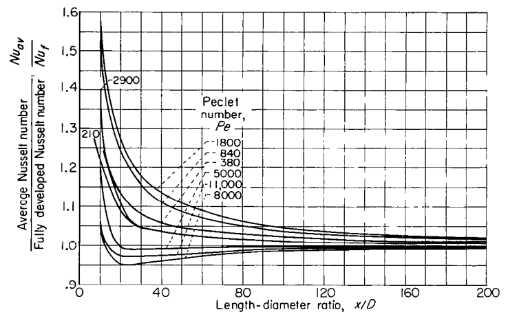
FIGURE 43.—Predictions of Deissler (ref. 37) for variation of ratio of average Nusselt number to fully developed Nusselt number with length-diameter ratio for various Peclet numbers (Prandtl number, 0.01).
