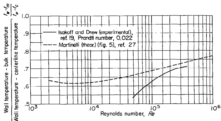
FIGURE 48.—Comparison of measured and predicted values of ratio (t_w - t_m)/(t_w - t_c) in round tubes with uniform heat input to wall.
