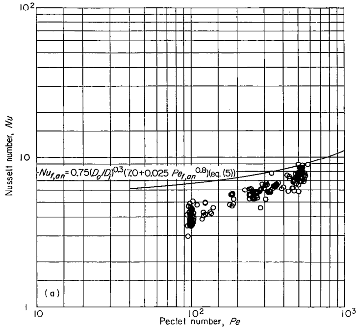
(a) Test section A (ratio of outer to inner diameter, 1.43; length-diameter ratio l/D , 223).
