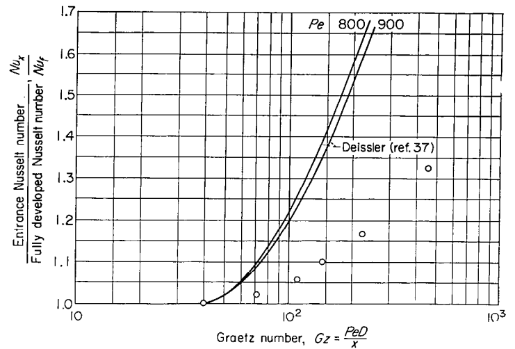
FIGURE 18.—Data of English and Barrett (ref. 9) for entrance-region heat transfer to mercury in round tubes. Peclet number, 800 to 900.
