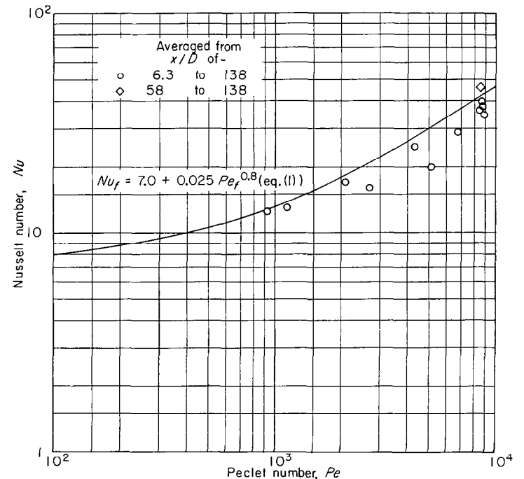
FIGURE 31.—Data of Isakoff and Drew (refs. 19 and 20) for average heat transfer to mercury in round tubes (inside wall temperatures calculated from outside wall temperatures).
