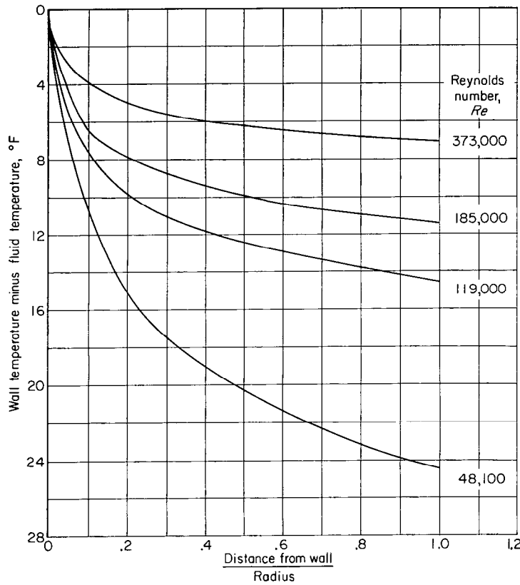
FIGURE 4.—Theoretical predictions of Martinelli (ref. 27) for fully developed temperature profiles for heat transfer to liquid metals in round tubes. Prandtl number, 0.022.
