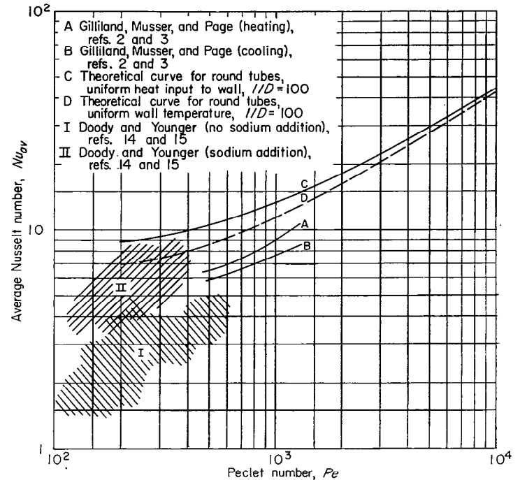
FIGURE 46.—Comparison of measured and predicted average Nusselt numbers in round tubes with uniform wall temperature or with a wall condition somewhere between uniform wall temperature and uniform heat input.
