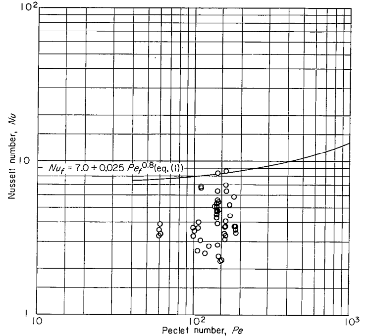
FIGURE 35.—Data of MacDonald and Quittenton (refs. 22 and 23) for fully developed heat transfer to sodium in round tubes.
