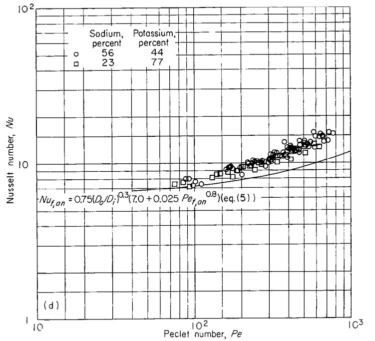
(d) In annuli; test section B (length-diameter ratio l/D , 54; ratio of outer to inner diameter, 1.83).
