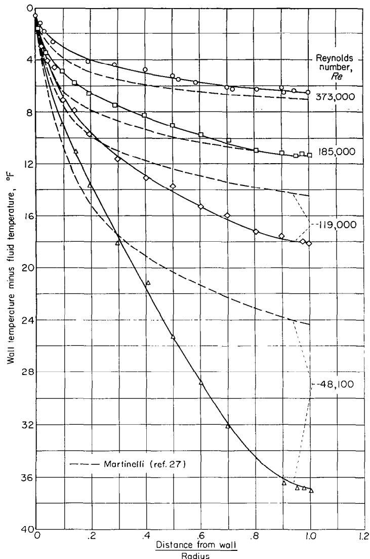
FIGURE 32.—Data of Isakoff and Drew (refs. 19 and 20) for fully developed temperature distribution for heat transfer to mercury in round tubes. Length-diameter ratio x/D , 138.
