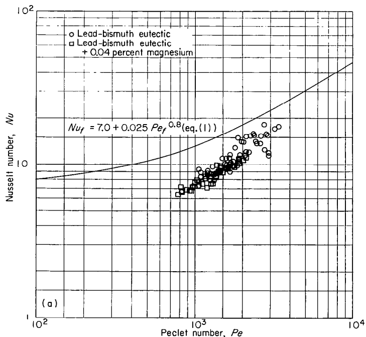
(a) In round tubes; length-diameter ratio l/D , 100.
