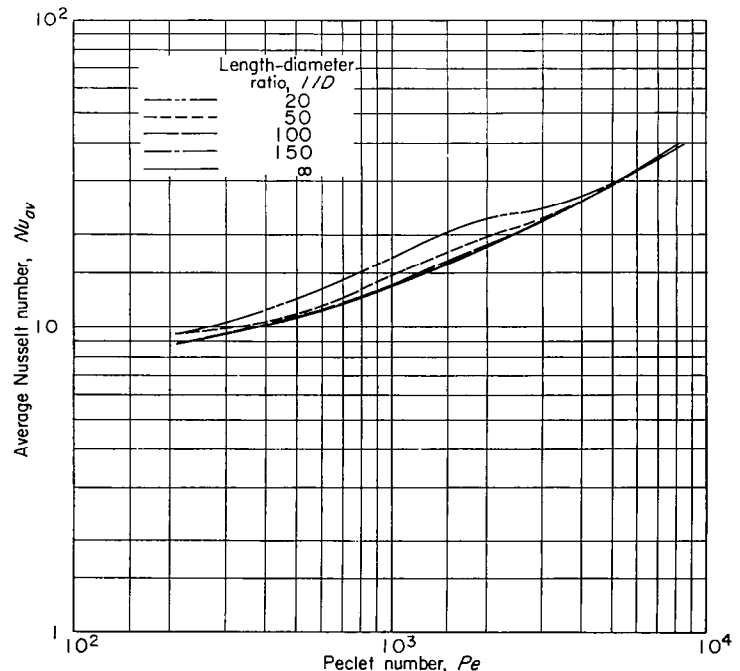
FIGURE 44.—Variation of average Nusselt number with Peclet number for several length-diameter ratios as determined from figure 43 and equation (1).
