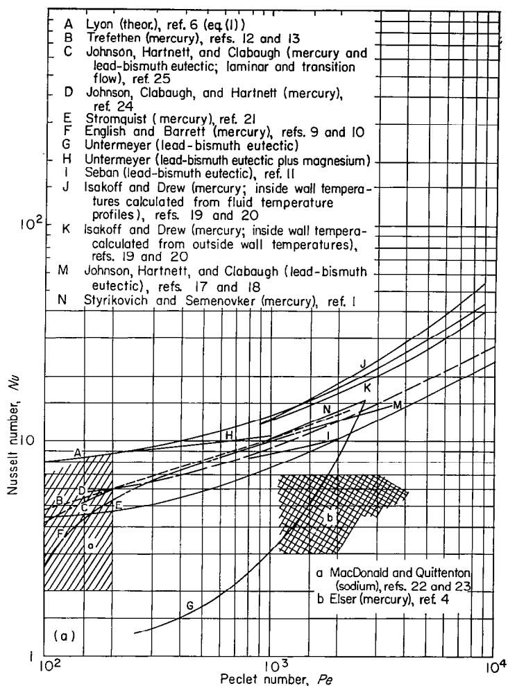
(a) Faired curves of experiments.
