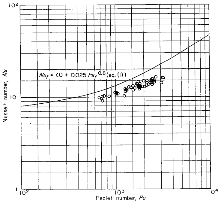
FIGURE 27.—Data of Johnson, Hartnett, and Clabaugh (refs. 17 and 18) for average heat transfer to lead-bismuth eutectic in round tubes. Length-diameter ratio l/D , 74.
