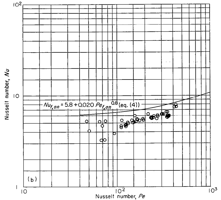
(b) Test section B (ratio of outer to inner diameter, 1.23; length-diameter ratio l/D , 397).
