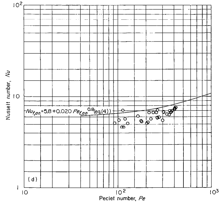
(d) Test section D (ratio of outer to inner diameter, 1.37; length-diameter ratio l/D , 375).
