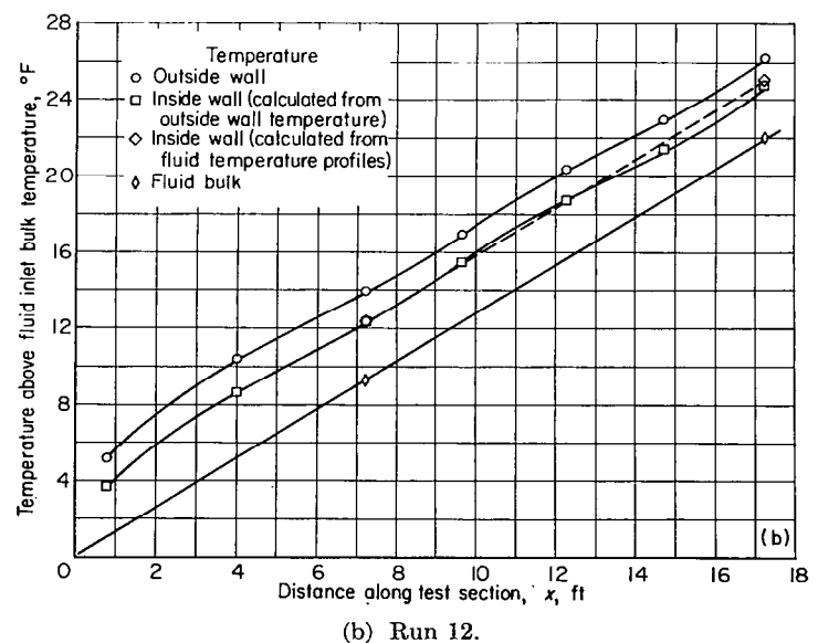
FIGURE 28.—Test-section temperatures from two typical runs of Isakoff and Drew (refs. 19 and 20).
