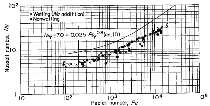
FIGURE 33.—Data of Stromquist (ref. 21) for fully developed heat transfer to mercury, with and without sodium additions, in round tubes.
