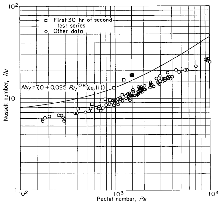
FIGURE 36.—Data of Johnson, Clabaugh, and Hartnett (ref. 24) for fully developed heat transfer to mercury in round tubes.
