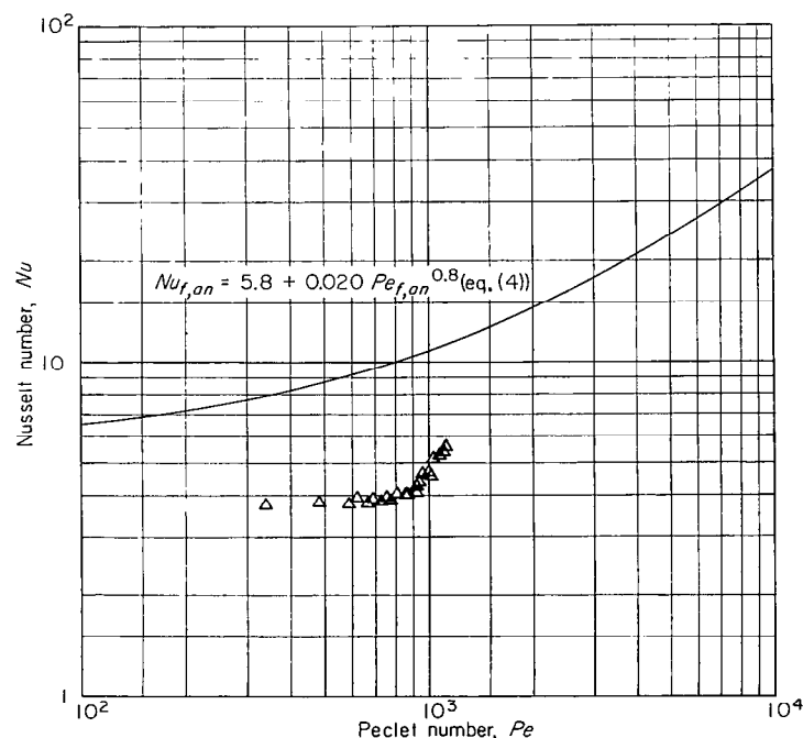
FIGURE 16.—Data of Sineath (ref. 8) for average heat transfer to mercury in rectangular ducts. Length-diameter ratio l/D , 50.
