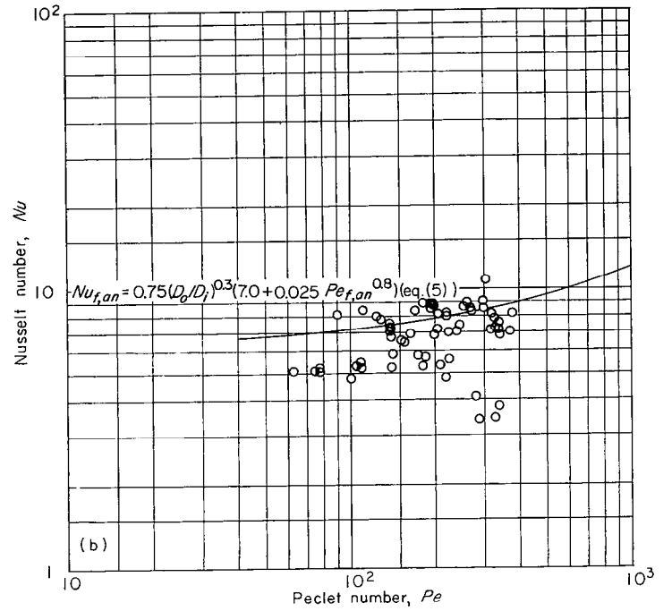
(b) In annuli; test section A (length-diameter ratio l/D , 54; ratio of outer to inner diameter, 1.83).
