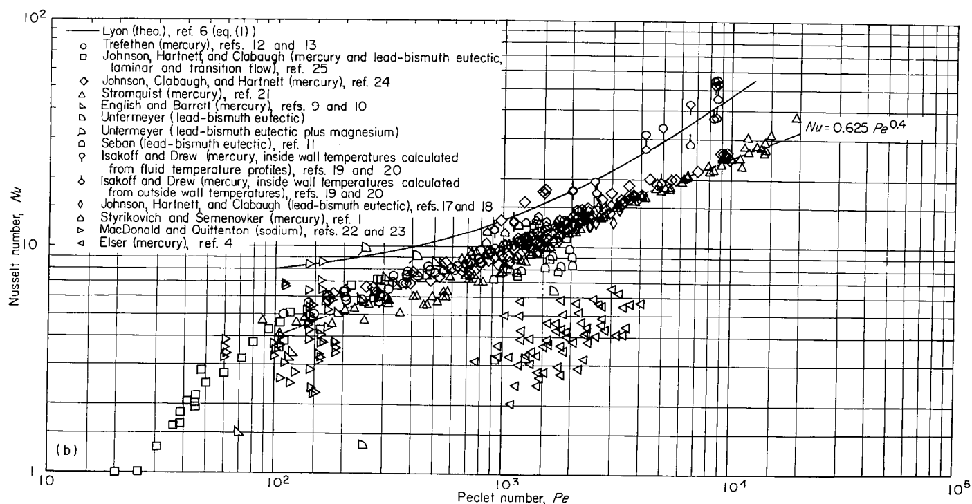
(b) Reevaluated data points.
