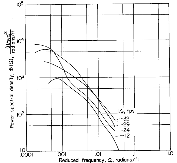
FIGURE 2.—Measurements of the power spectrum of atmospheric turbulence obtained at 300 feet from a meteorological tower (ref. 19).
