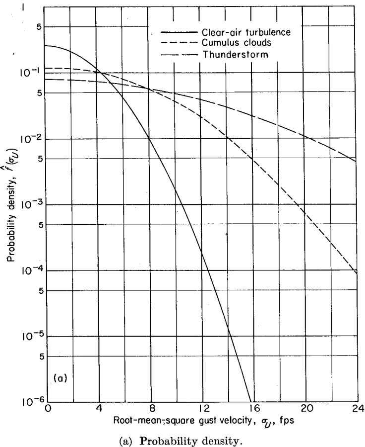
FIGURE 12.—Distribution of root-mean-square gust velocity with weather condition.
