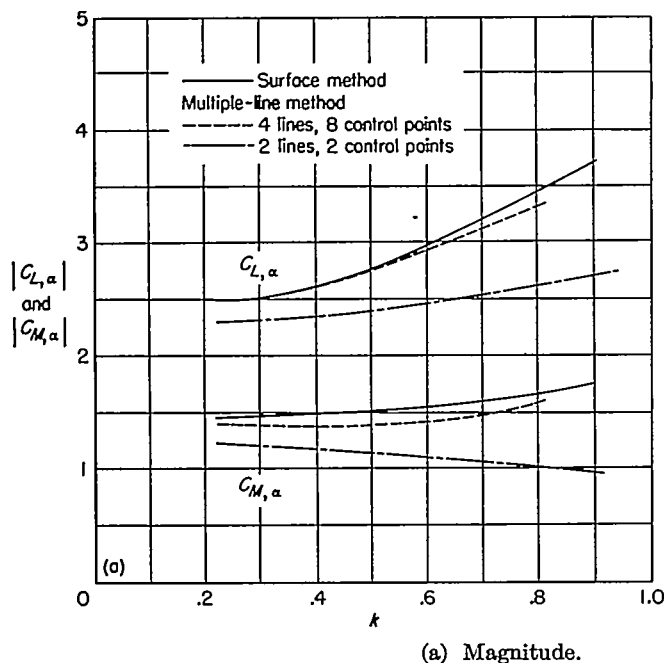
FIGURE 6.—Variation of lift and moment with reduced frequency k for a rectangular wing oscillating in pitch about its midchord. Comparison of results of multiple-line method with results of surface-loading method. A=2 ; M=0 .
