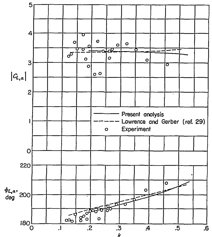
FIGURE 4.—Variation of lift with reduced frequency k for a delta wing oscillating in pitch about its midchord. A=4 ; M=0 .
