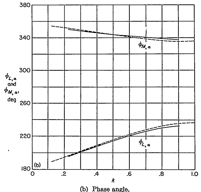
FIGURE 2.—Variation of lift and moment with reduced frequency k for a rectangular wing oscillating in pitch about its midchord. A=2 ; M=0 .
