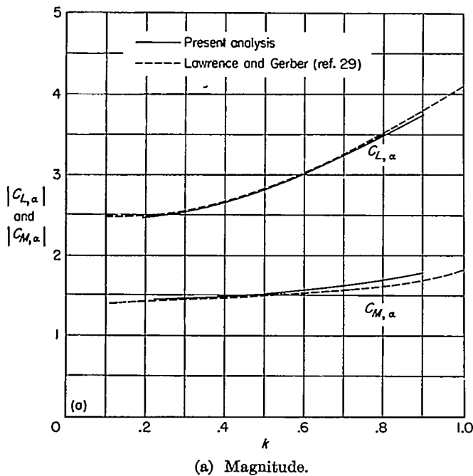
FIGURE 2.—Variation of lift and moment with reduced frequency k for a rectangular wing oscillating in pitch about its midchord. A=2 ; M=0 .
