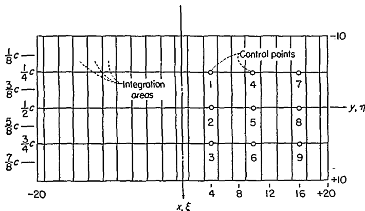
FIGURE 1.—Typical layout for lifting-surface method applied to a rectangular wing.
