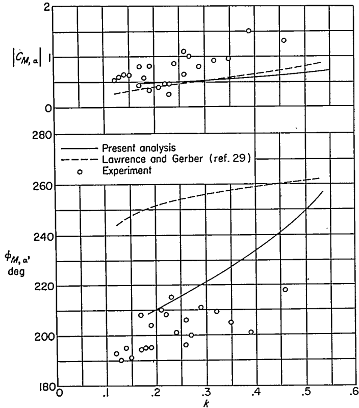
FIGURE 5.—Variation of moment with reduced frequency k for a delta wing oscillating in pitch about its midchord. A=4 ; M=0 .
