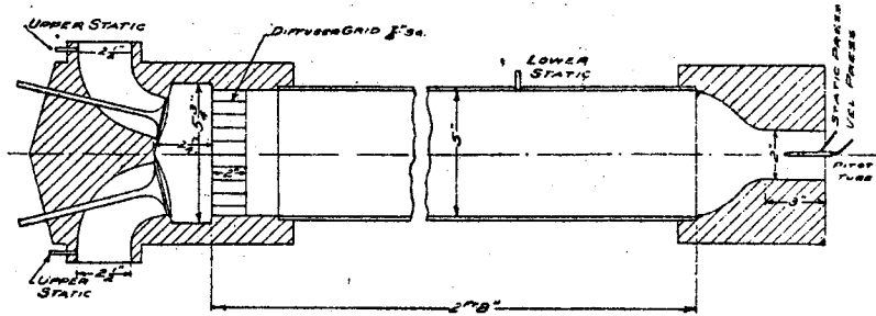
PLATE 1.—Cross through cylinder model.
