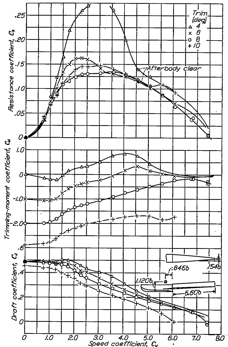
FIGURE 9.—Resistance, trimming-moment, and draft characteristics of model 163J-11 at fixed trim.
