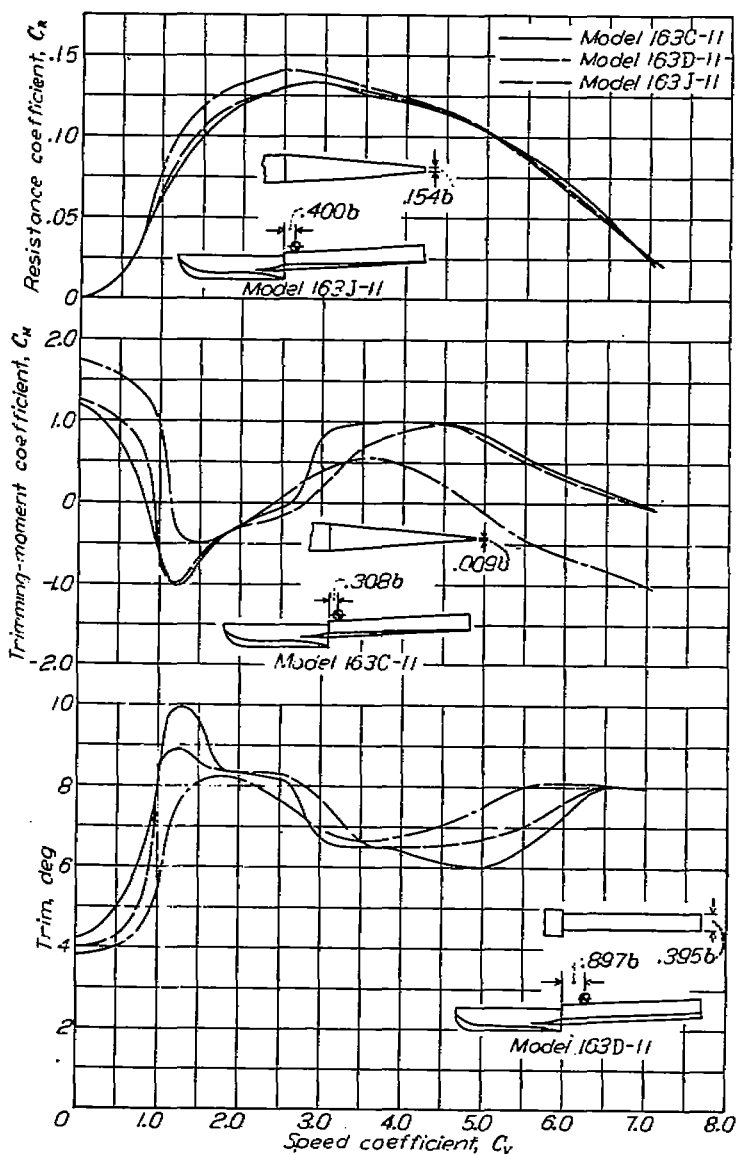
FIGURE 12.—Effect on best-trim characteristics of tapering afterbody.
