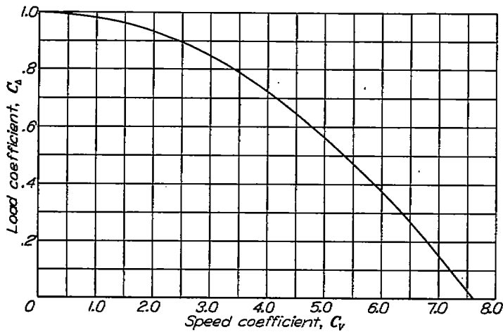
FIGURE 4.—Load curve based on constant lift coefficient.
