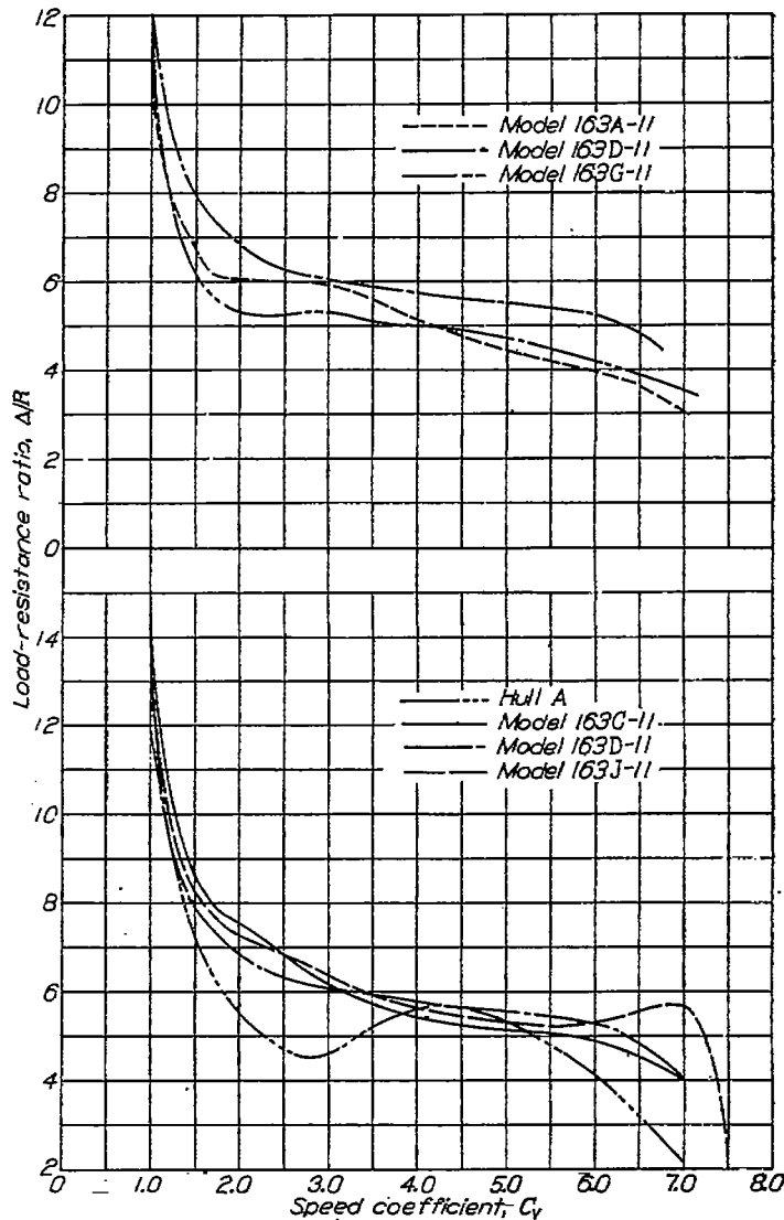
FIGURE 15.—Comparison of load-resistance ratios of planing-tail hulls and a conventional hull.
