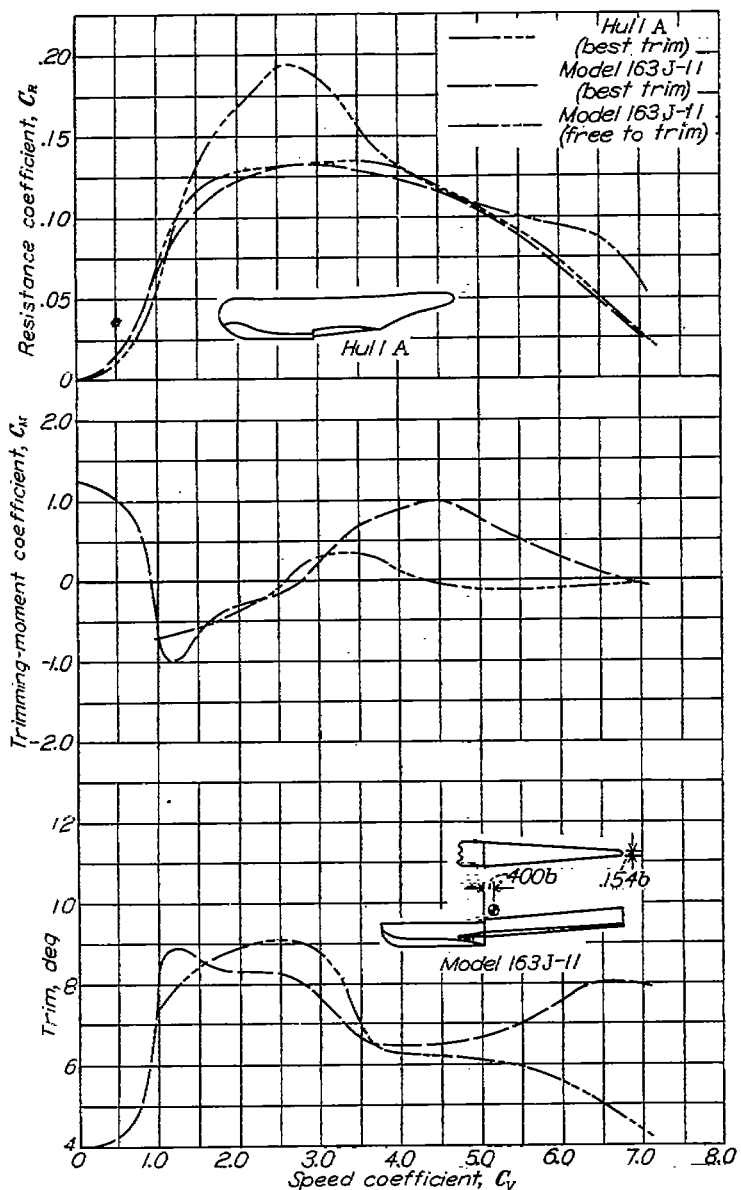
FIGURE 14.—Comparison of the resistance characteristics of a planing-tail hull with those of a conventional hull.
