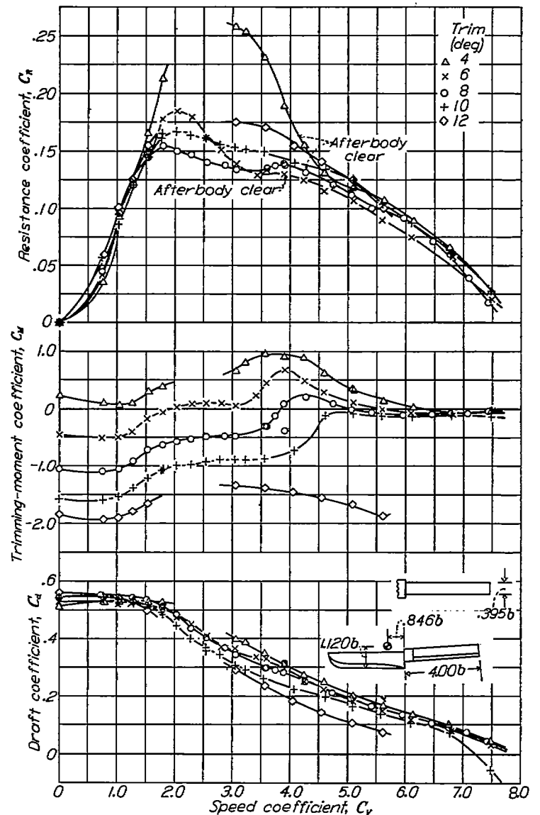
FIGURE 5.—Resistance, trimming-moment, and draft characteristics of model 163A-11 at fixed trim.
