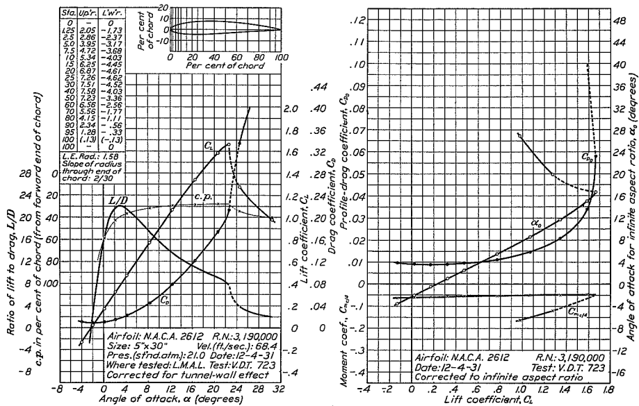
FIGURE 28.—N.A.C.A. 2612 airfoil.
