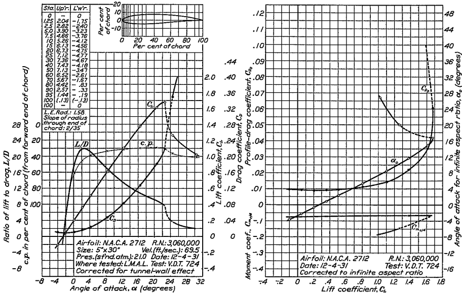
FIGURE 29.—N.A.C.A. 2712 airfoil.
