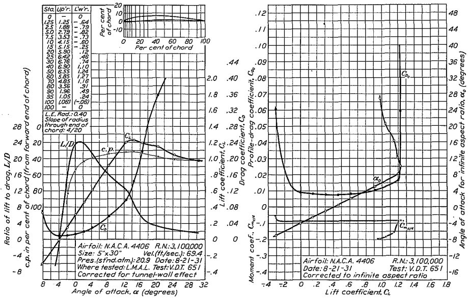
FIGURE 37.—N.A.C.A. 4406 airfoil.
