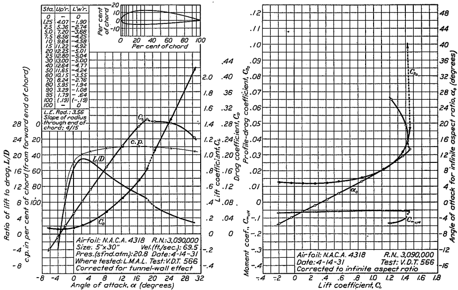
FIGURE 35.—N.A.C.A. 4318 airfoil.
