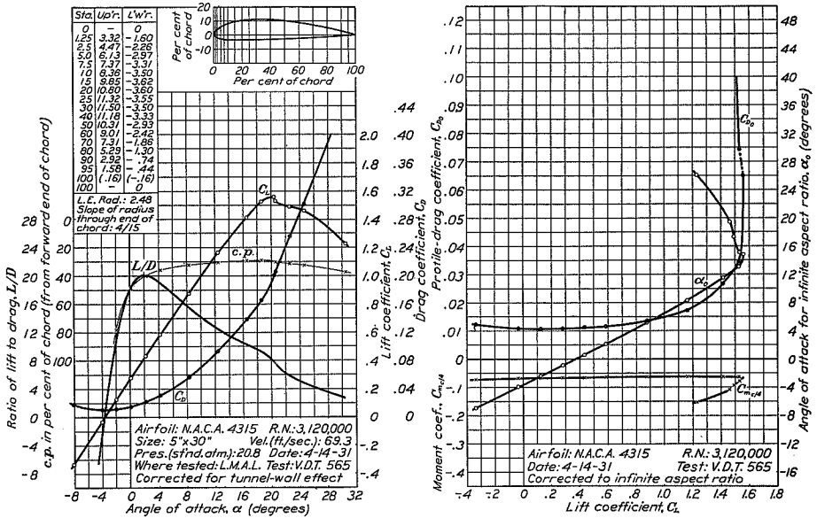
FIGURE 34.—N.A.C.A. 4315 airfoil.
