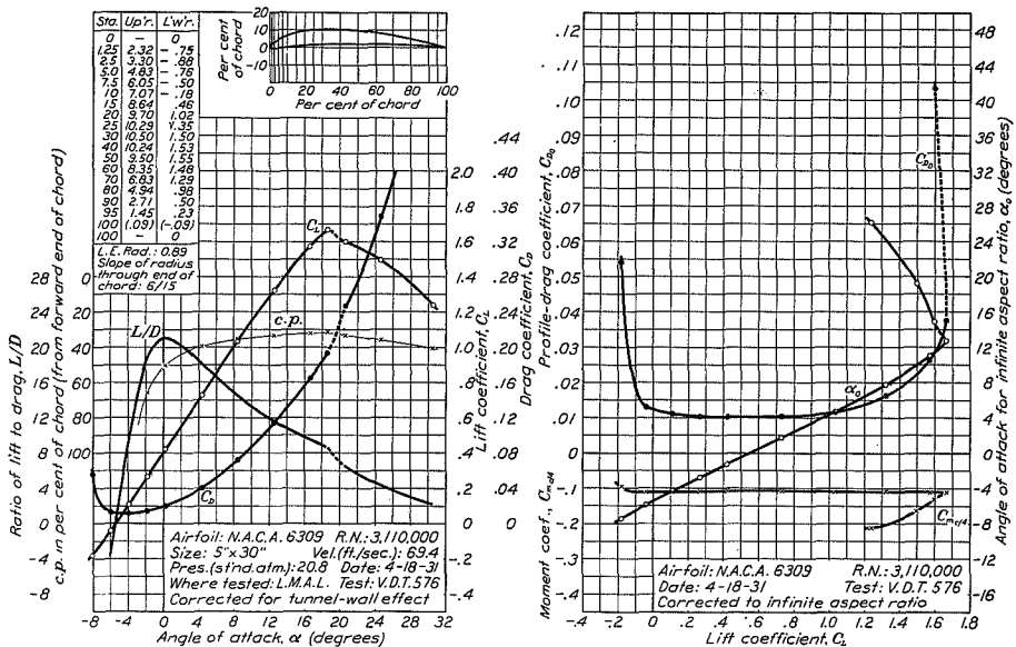
FIGURE 63.—N.A.C.A. 6309 airfoil.
