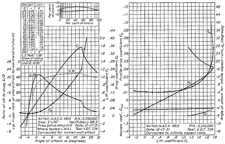
FIGURE 49.—N.A.C.A. 4612 airfoil.
