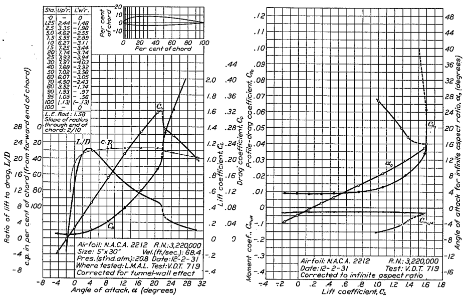
FIGURE 11.—N.A.C.A. 2212 airfoil.
