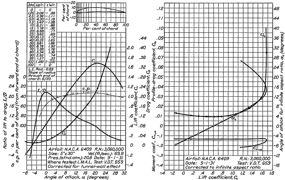
FIGURE 59.—N.A.C.A. 6409 airfoil.
