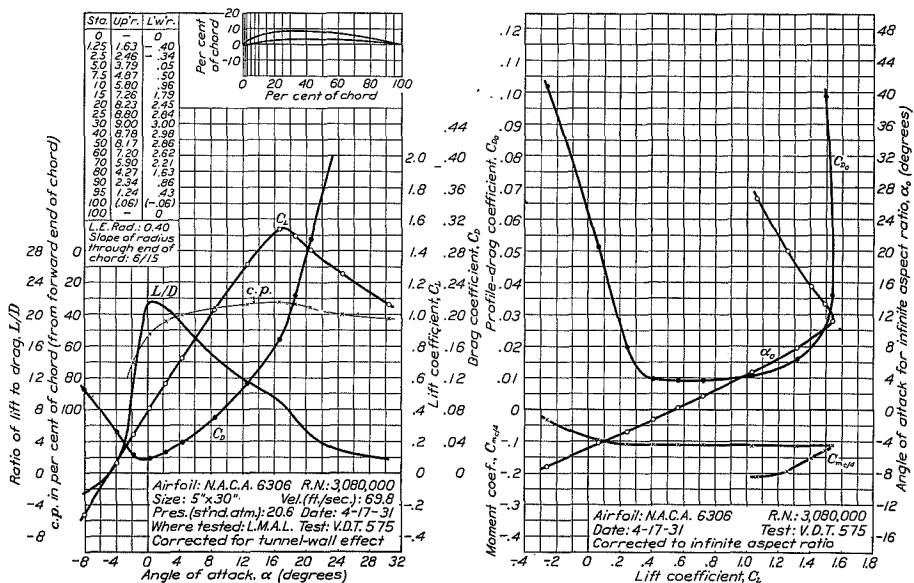
FIGURE 62.—N.A.C.A. 6306 airfoil.
