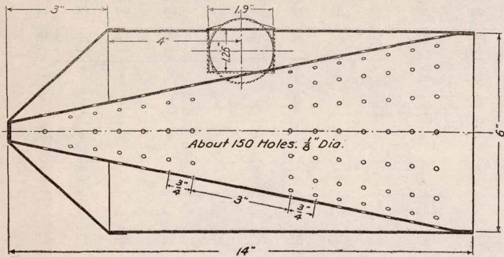
TENTATIVE SUGGESTION FOR MUFFLER No. 18 U.S. Gauge (0.05) Sheet Metal, Welded. For Airplane Engine, 6 or 12 Cylinder, 5" Bore, 7" Stroke.
