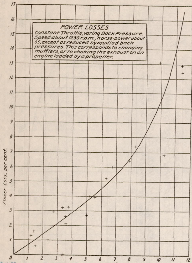
Plot No. 2 Applied Back Pressure, inches of mercury.
