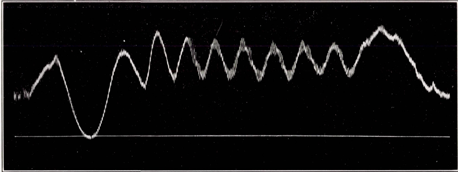
FIG. 24.—SPIN OF 9\frac{1}{2} TURNS, JN4H. QUICK PULL UP INTO STALL, MOTOR THROTTLED. DESCENDED 1,700 FEET. MAXIMUM ACCELERATION IN THE SPIN WAS 2.57 G. AND WHEN PULLING OUT 2.70 G.
