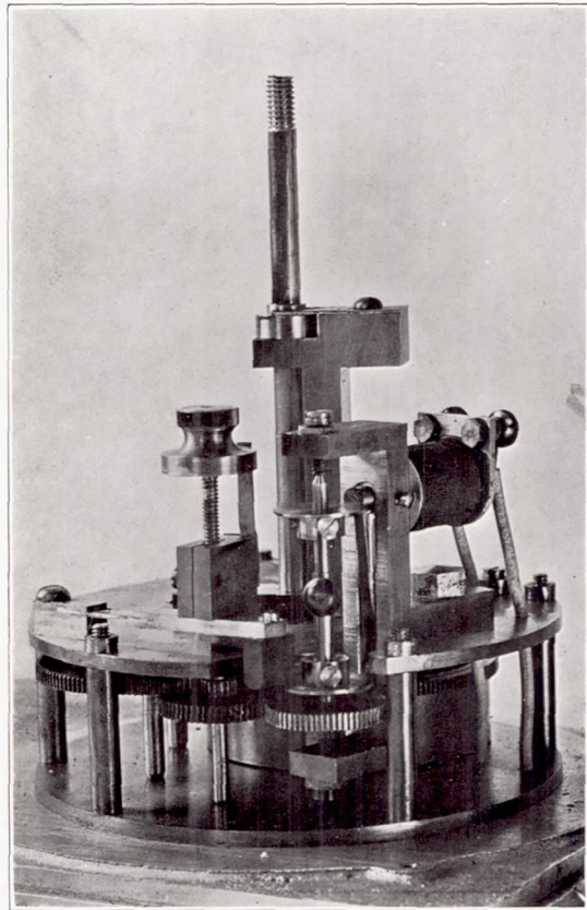
FIG. 5.—ACCELEROMETER CLOCK.
