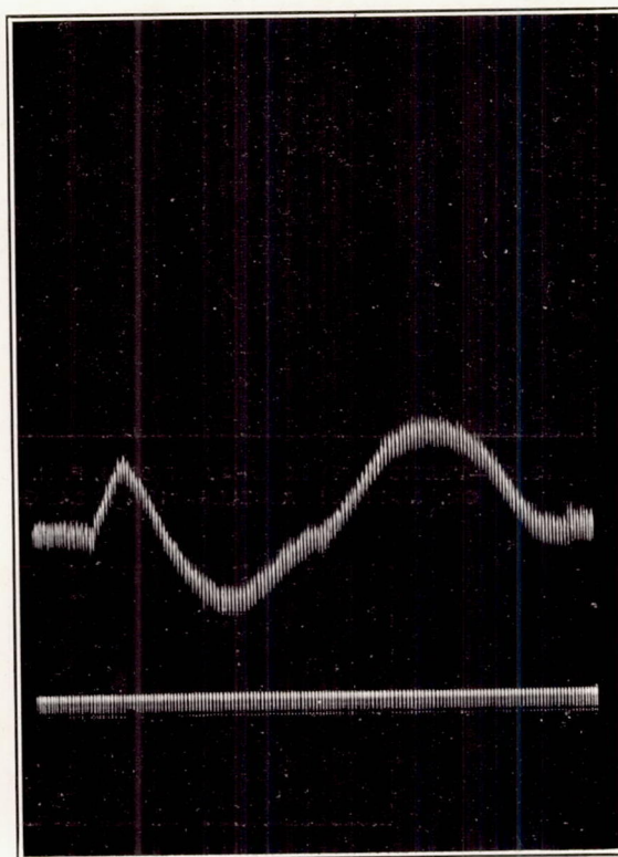
FIG. 33.—STICK PULLED BACK SUDDENLY AT 50 M. P. H. ON JN4H. MOTOR THROTTLED. MAXIMUM ACCELERATION IS 1.46 G.
