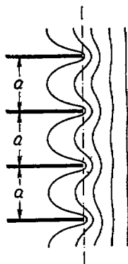
FIG. 60.—Conformal transformation
