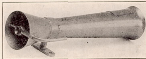
FIG. 8.—Venturi tube for Pioneer turn indicator.
