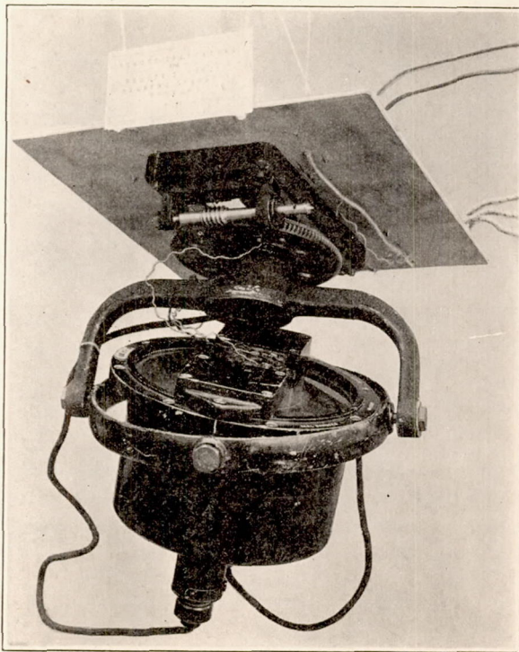
FIG. 28.—Remote indicating and remote control compass. (Magnetic compass removed from housing.)
