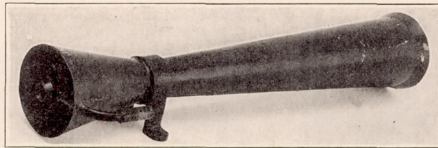
FIG. 7.—Venturi tube for Sperry turn indicator
