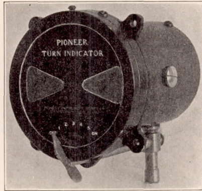
FIG. 2.—Pioneer turn indicator.
