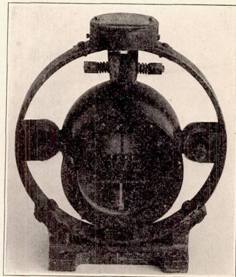
FIG. 7.—Creagh-Osborne aero compass, Type 259.
