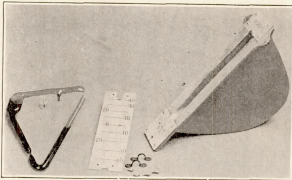
FIG. 10.—Liquid fore-and-aft inclinometer.
