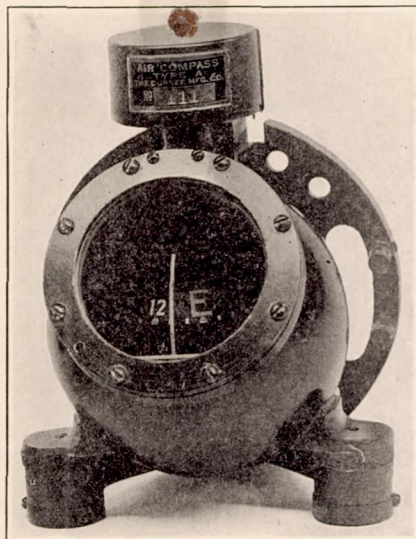
FIG. 2.—Air compass, Type A.
