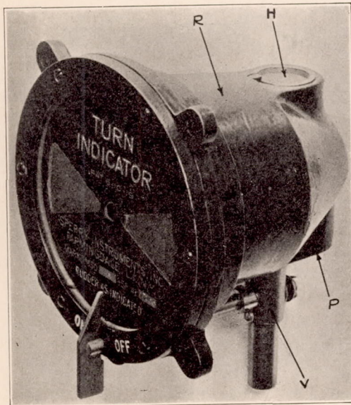
FIG. 4.—Sperry turn indicator.
