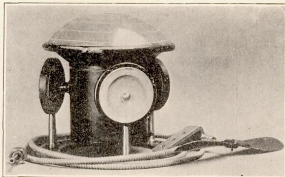
FIG. 8.—Hebrard spinning top.
