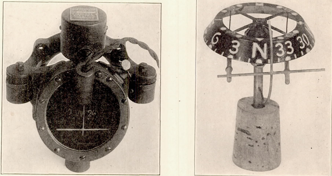
FIG. 1.—General Electric air compass, Type B.
