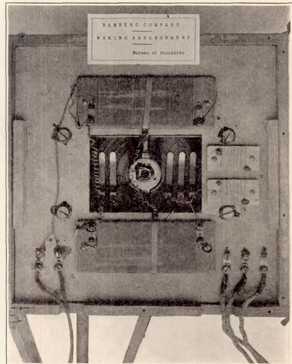
FIG. 29.—Remote indicating and remote control compass. (Wiring arrangement.)
