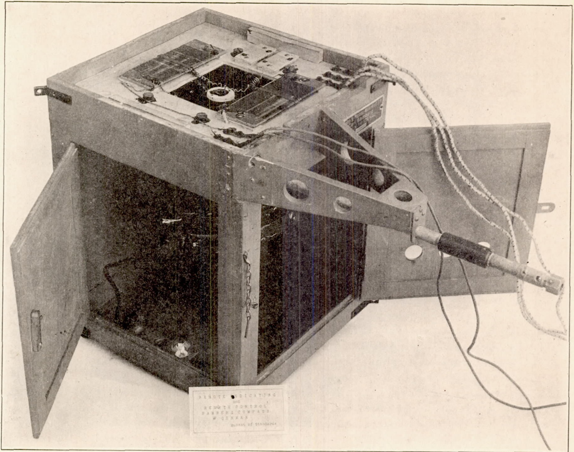
FIG. 27.—Remote indicating and remote control compass. (Magnetic compass in housing.)
