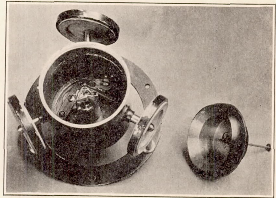
FIG. 8.—Hebrard spinning top.
