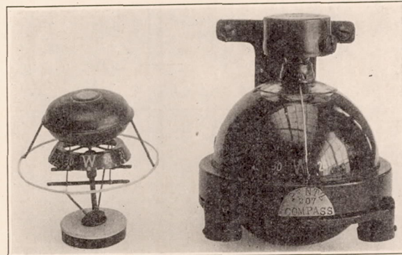
FIG. 5.—Pentz compass.
