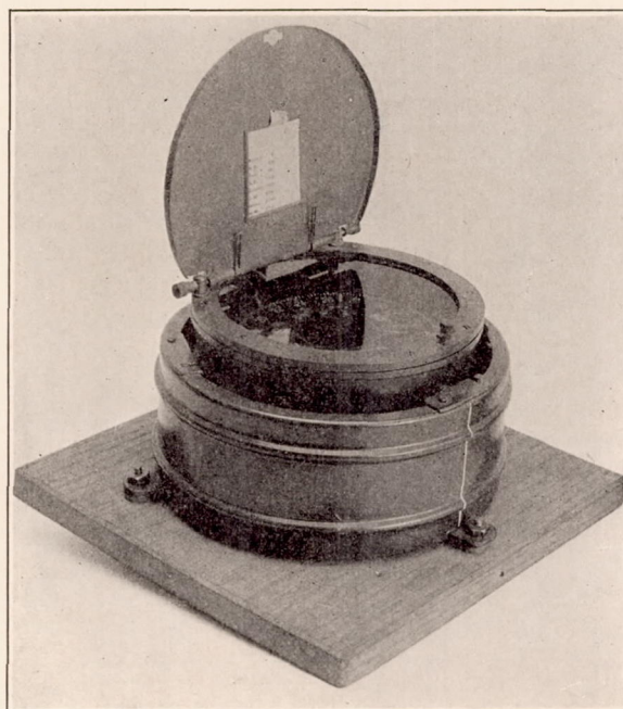
FIG. 8.—Creagh-Osborne aero compass, Type 253.
