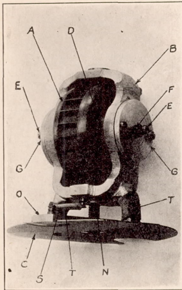
FIG. 6.—Sperry mechanism
