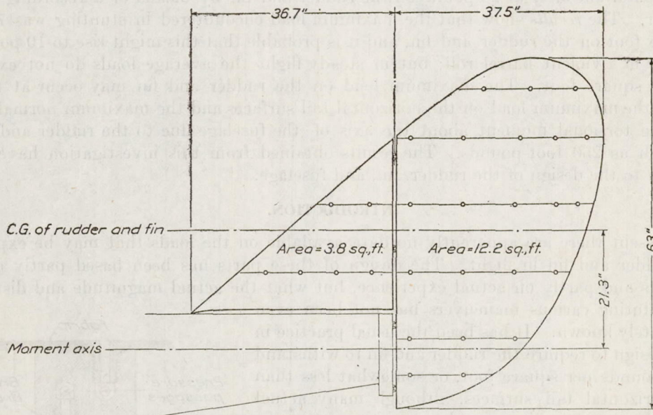
FIG. 3.—Elevation of fin and rudder showing location of ho es.
