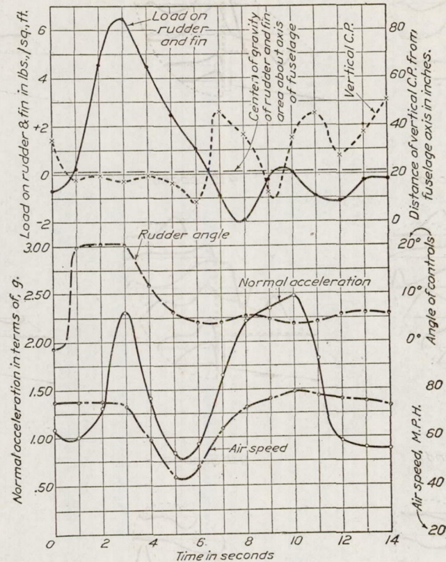
FIG. 7.—Roll to right.
