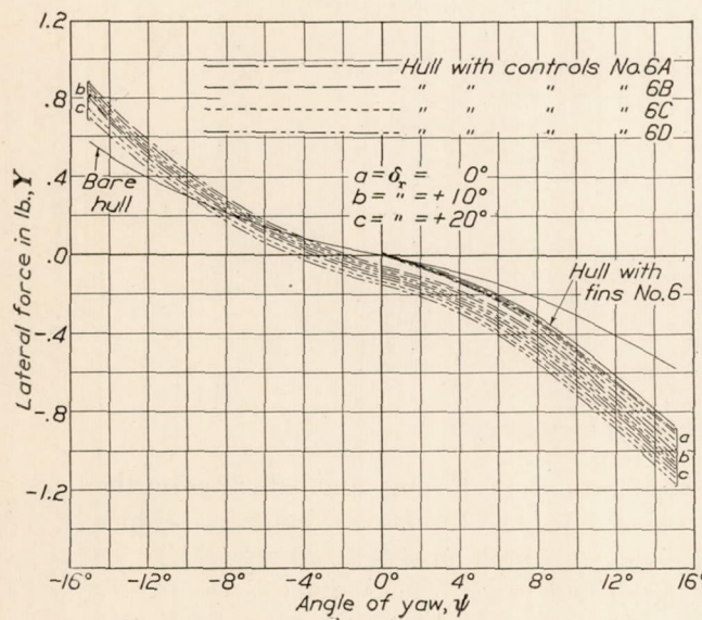
FIG. 13.—Y force for short model with controls No. 6. Model at 0° pitch and elevators neutral. Airspeed 40 M. P. H.
