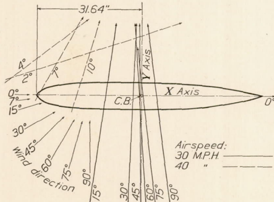
FIG. 28.—Line of resultant air force on long hull with No. 5 controls. Model at 0° pitch. Elevators and rudders neutral. Scale of model 1/120 full size
