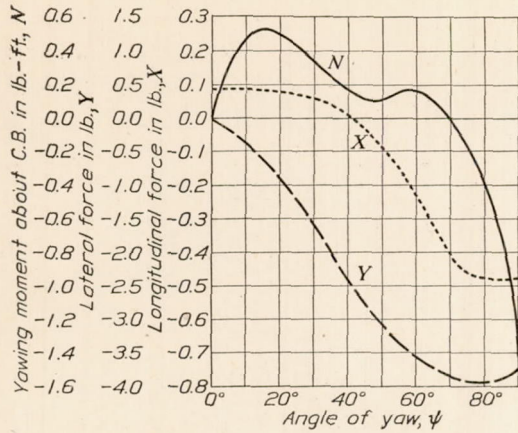
FIG. 27.—X and Y forces and yawing moments N for long model with No. 5 control surfaces. Model at 0° pitch. Elevators and rudders neutral. Airspeed 30 M. P. H.
