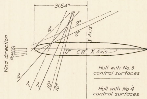
FIG. 30.—Line of resultant air force on long hull with Nos. 3 and 4 controls. Model at 0° pitch. Elevators and rudders neutral. Airspeed 40 M. P. H. Scale of model 1/120 full size
