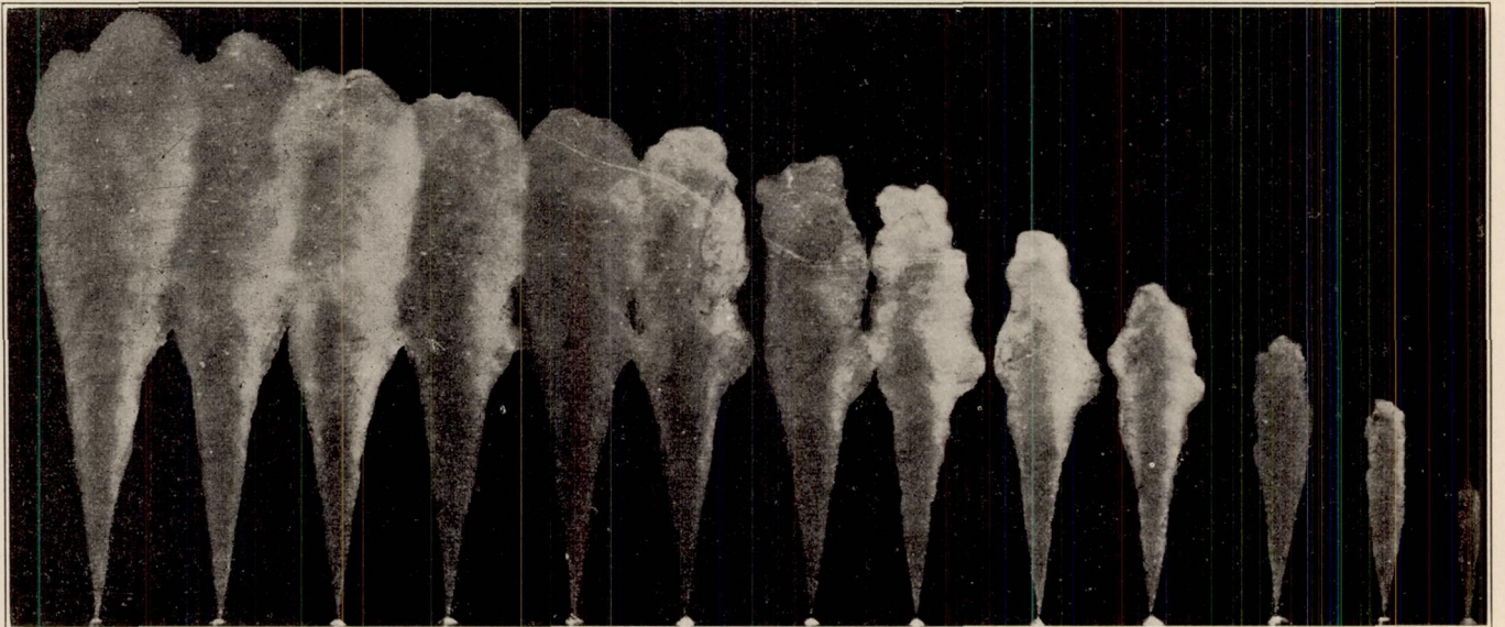
FIG. 8.—Injection pressure, 8,000 lb./sq. in. Chamber pressure, 300 lb./sq. in. The original photographs for Figures 3 to 8 inclusive were retouched for reproduction purposes
