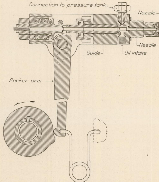
FIG. 2.—Fuel injection valve mechanism
