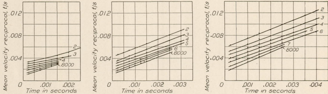
FIG. 18.—Chamber pressure, 100 lb./sq. in. FIG. 19.—Chamber pressure, 200 lb./sq. in. FIG. 20.—Chamber pressure 300 lb./sq. in. Fuel pressure, 2,000 to 8,000 lb./sq. in. Relation of mean velocity reciprocal ( t/s ) to time.
