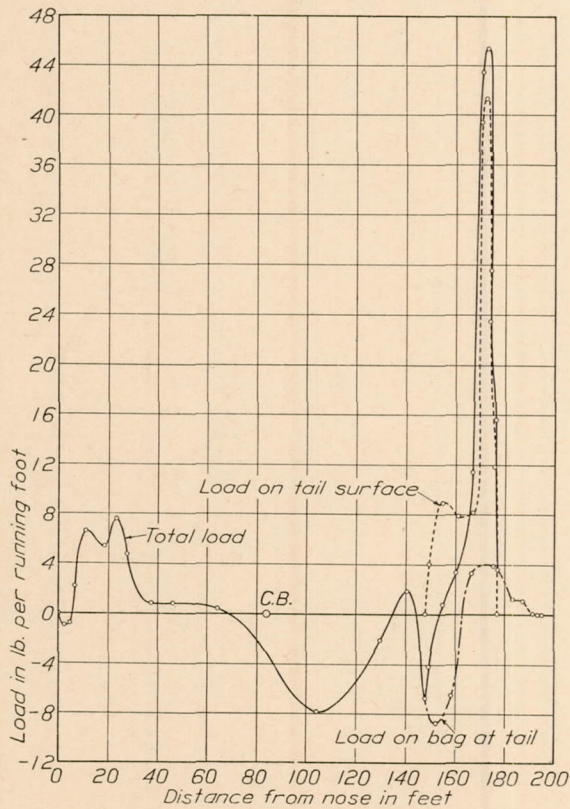
FIG. 25b.—Horizontal loads. Run 27b, reversal. Rudder angle 24° left to 18° right. 1,250 R. P. M. Positive loads acting to port. (NOTE.—The moment of the resultant aerodynamic forces on the vertical tail surfaces about the C. B. = 35,100 lb./ft. clockwise)
