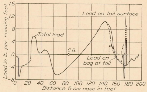
FIG. 26a.—Vertical loads. Run 4, steady circle. Rudder angle 8° right. 1,250 R. P. M. Positive loads acting upward. (NOTE.—The moment of the resultant aerodynamic forces on the horizontal tail surfaces about the C. B. = 3,735 lb./ft. counterclockwise)
