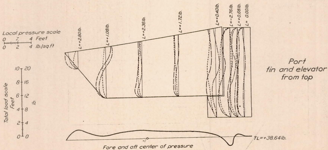
FIG. 12.—Tail surface load curves. Run No. 5, steady circle. Rudder angle 44^\circ right. 1,250 R. P. M Positive loads are those acting from lower side to upper
