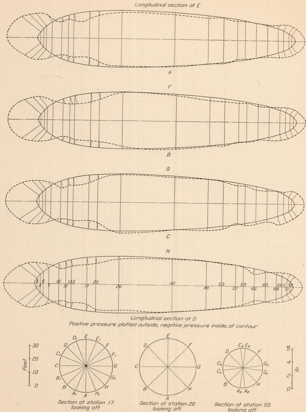
FIG. 21.—Pressure distribution on envelope. Run 9b, start circle. Rudder angle 44° right. 1,250 R. P. M.
