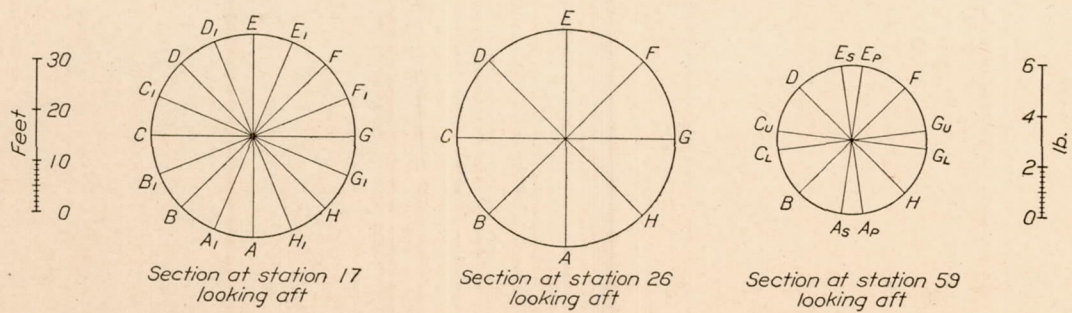
FIG. 17.—Pressure distribution on envelope. Run 27b, reversal. Rudder angle 24° left to 18° right. 1,250 R. P. M.
