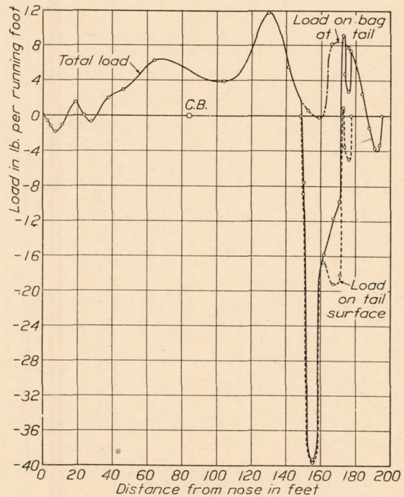
FIG. 26b.—Horizontal loads. Run 4, steady circle. Rudder angle 8° right. 1,250 R. P. M. Positive loads acting to port. (NOTE.—The moment of the resultant aerodynamic forces on the vertical tail surfaces about the C. B. = 37,200 lb./ft. counterclockwise)
