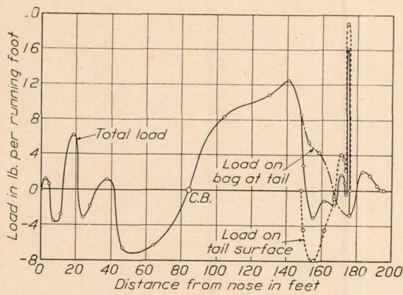
FIG. 25a.—Vertical loads. Run 27b, reversal. Rudder angle 24° left to 18° right. 1,250 R. P. M. Positive loads acting upward. (NOTE.—The moment of the resultant aerodynamic forces on the horizontal tail surfaces about the C. B. = 2,270 lb./ft. clockwise)
