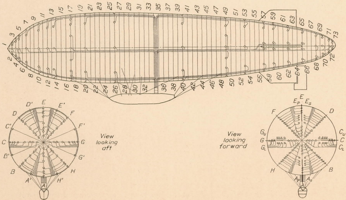
FIG. 4.—Location of pads and tubing on envelope
