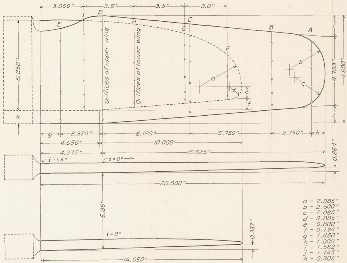
FIG. 2.—Plan and front elevation of PW-9 wing models
