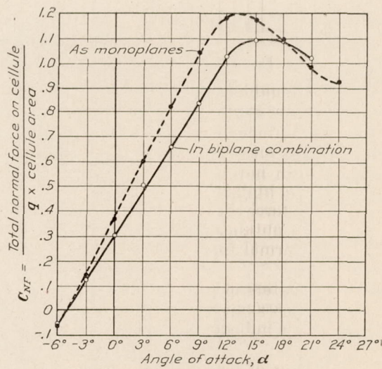
FIG. 13.—Cellule normal force coefficient
