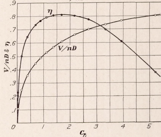
FIGURE 9.—Propeller D in free wind stream
