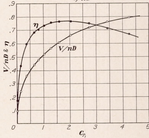
FIGURE 13.—Propeller B with model fuselage
