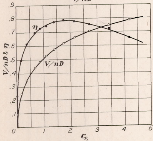
FIGURE 16.—Propeller E with model fuselage
