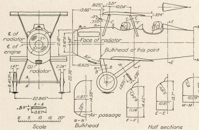
FIGURE 1.—Wind tunnel model of VE-7 airplane Chord, 20.36 inches; gap, 20.55 inches; stagger, 4.13 inches; angle of wing setting (upper wing) 1° 45'; lower, 2° 15'.
