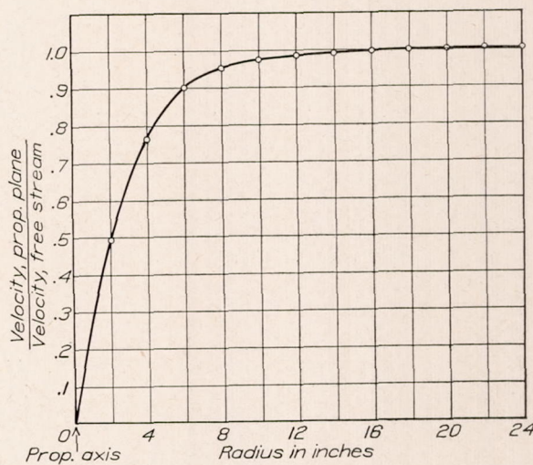
FIGURE 18.—Velocity in propeller plane, average. VE-7 model
