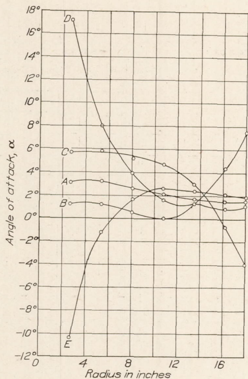
FIGURE 19.—Angles of attack of sections at V/nD for maximum efficiency. Free wind stream
