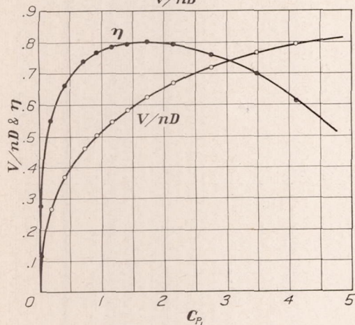
FIGURE 8.—Propeller C in free wind stream
