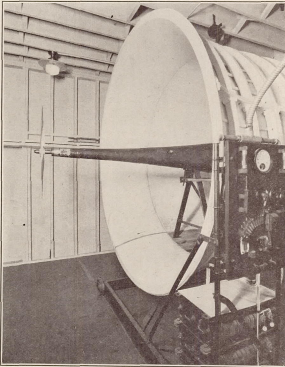
FIGURE 3.—Arrangement of apparatus for free stream tests
