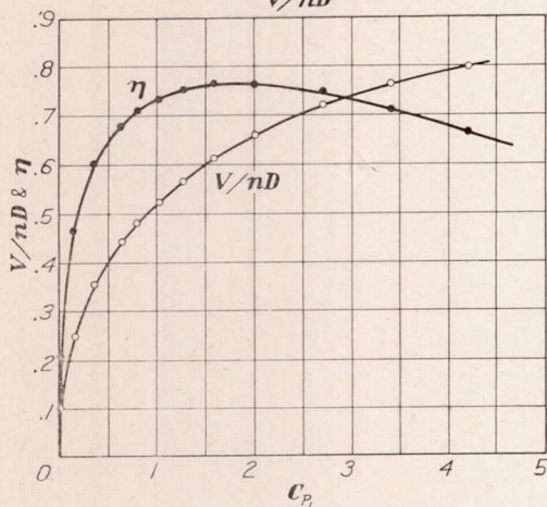
FIGURE 12.—Propeller A with model fuselage
