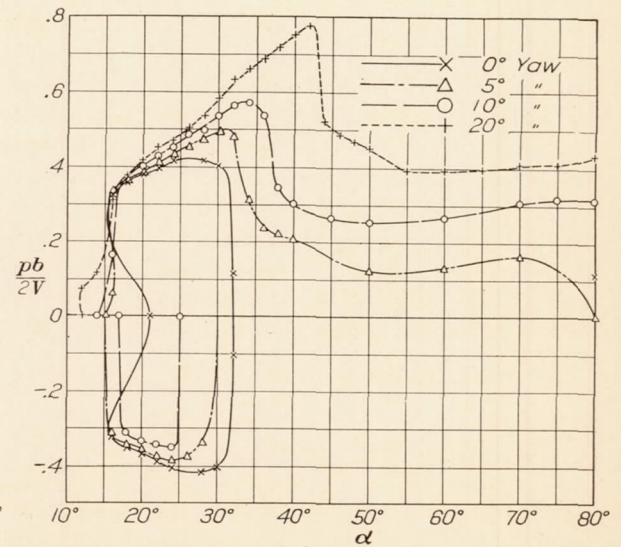
FIGURE 34.— -\frac{pb}{2V} vs. angle of attack for N. A. C. A. 84 monoplane wing model. Yaw=0°, 5°, 10°, 20°
