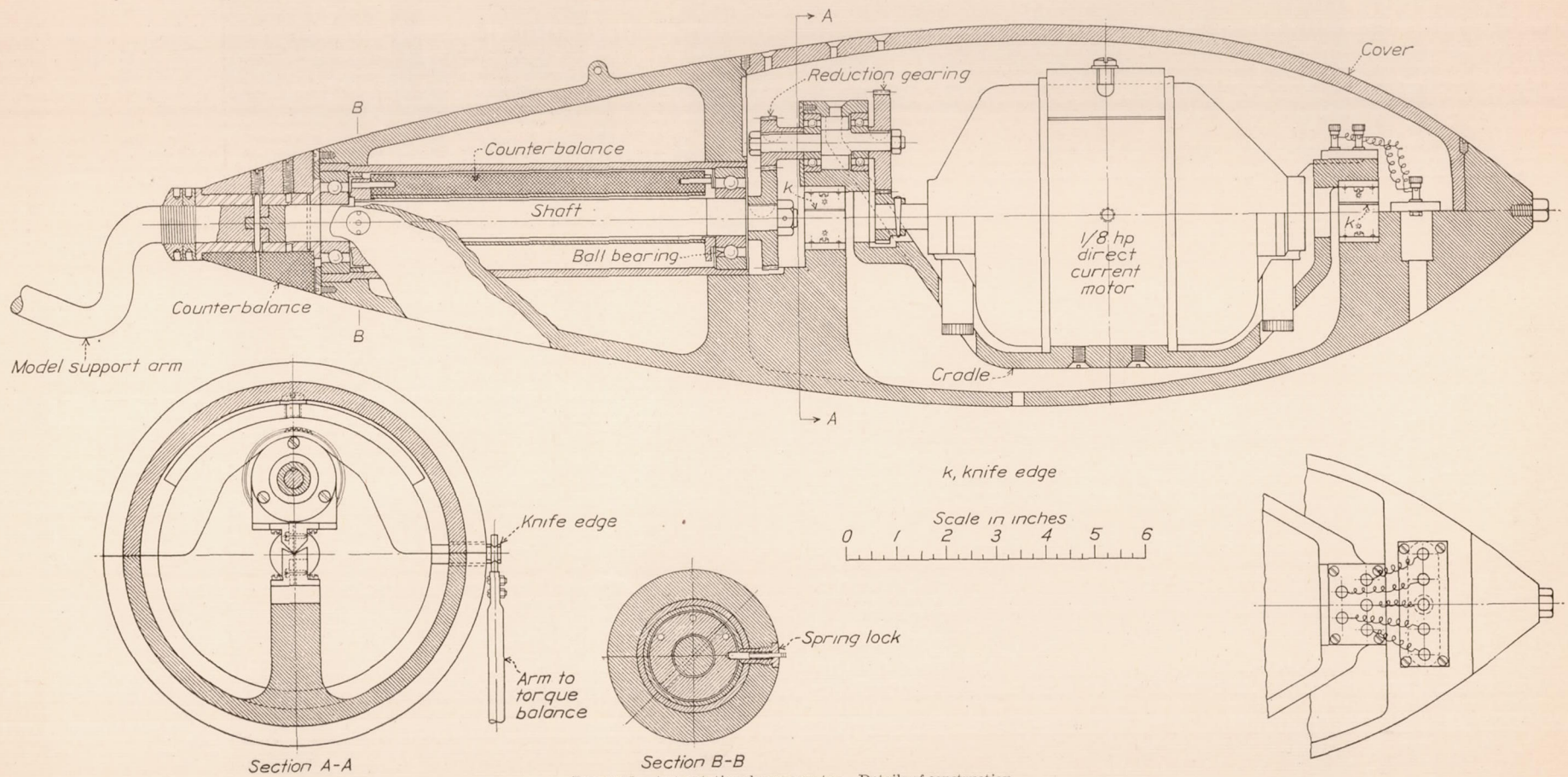
FIGURE 5.—Autorotation dynamometer. Details of construction
