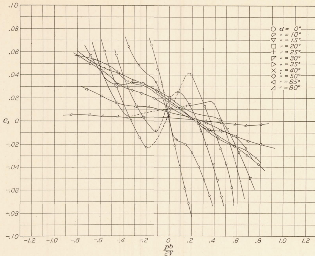
FIGURE 25.—Rolling moment coefficient vs. \frac{pb}{2V} for N. A. C. A. 86-M monoplane wing model. Yaw= 10^\circ
