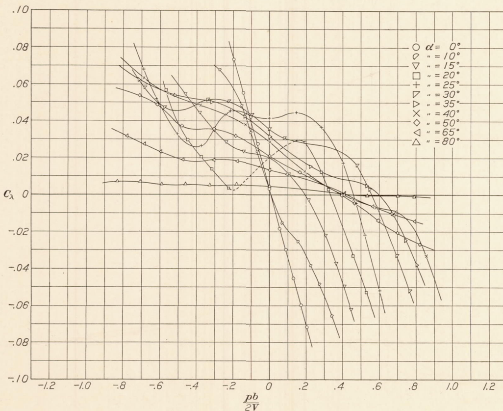
FIGURE 26.—Rolling moment coefficient vs. \frac{pb}{2V} for N. A. C. A. 86-M monoplane wing model. Yaw= 20^\circ
