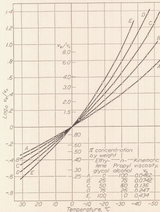
FIGURE 15.—Effect of temperature on the kinematic viscosity of solutions of ethylene glycol and n-propyl alcohol. \nu_\theta and \nu_0 are the kinematic viscosities of the liquid at a given temperature (designated by \theta ) and at 0° C.
