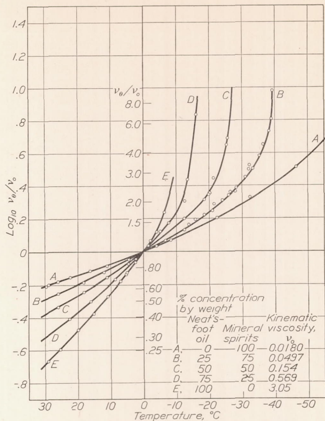
FIGURE 5.—Effect of temperature on the kinematic viscosity of solutions of neat's-foot oil (20° F.) and mineral spirits. v_\theta and v_0 are the kinematic viscosities of the liquid at a given temperature (designated by \theta ) and at 0° C.
