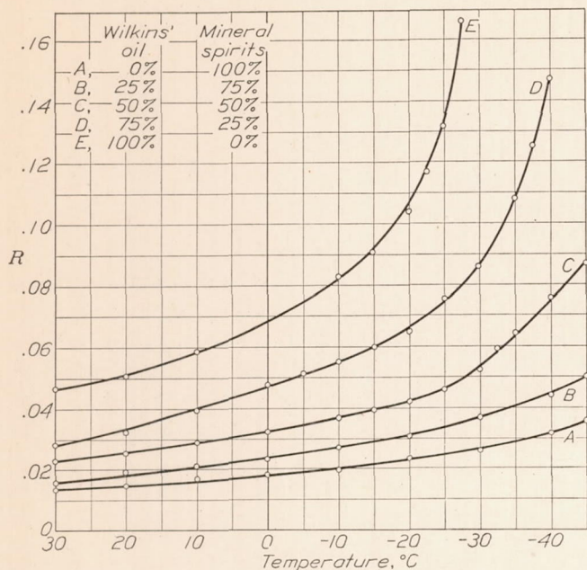
FIGURE 21.—Effect of temperature on the thermal coefficient R of kinematic viscosity of Wilkins' oil-mineral spirits solutions. R is the relative change in kinematic viscosity per degree centigrade. Similar curves are obtained for the other liquids of the mineral oil group
