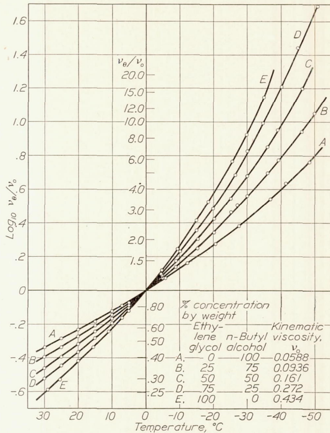
FIGURE 16.—Effect of temperature on the kinematic viscosity of solutions of ethylene glycol and n-butyl alcohol. v_\theta and v_0 are the kinematic viscosities of the liquid at a given temperature (designated by \theta ) and at 0° C.
