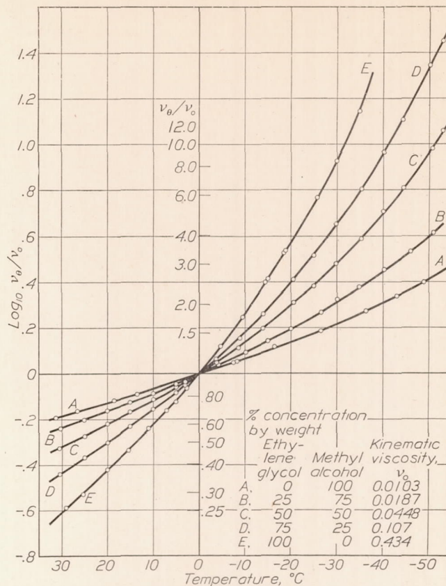
FIGURE 13.—Effect of temperature on the kinematic viscosity of solutions of ethylene glycol and methyl alcohol. \nu_\theta and \nu_0 are the kinematic viscosities of the liquid at a given temperature (designated by \theta ) and at 0° C.
