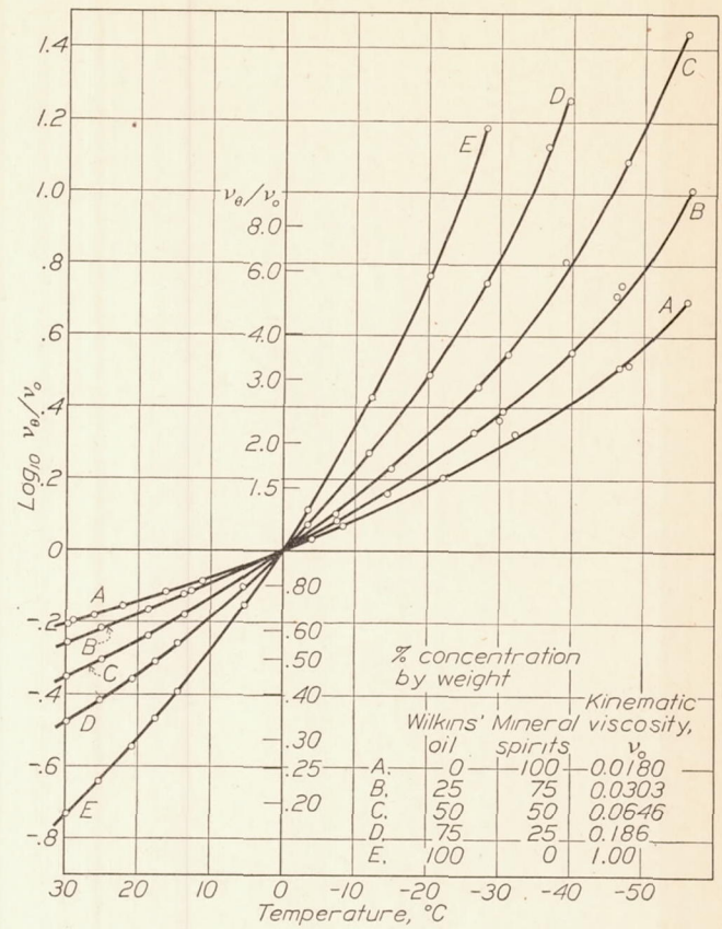
FIGURE 9.—Effect of temperature on the kinematic viscosity of solutions of Wilkins' oil and mineral spirits. v_\theta and v_0 are the kinematic viscosities of the liquid at a given temperature (designated by \theta ) and at 0° C.
