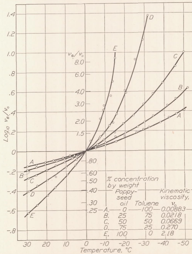
FIGURE 7.—Effect of temperature on the kinematic viscosity of solutions of poppy-seed oil and toluene. v_\theta and v_0 are the kinematic viscosities of the liquid at a given temperature (designated by \theta ) and at 0° C.
