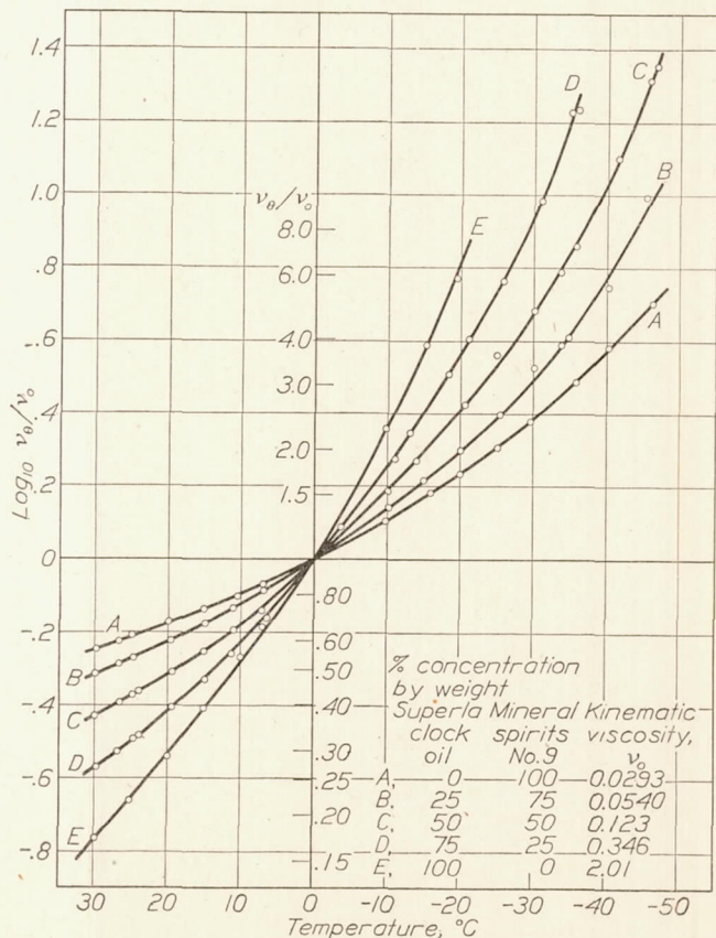
FIGURE 10.—Effect of temperature on the kinematic viscosity of solutions of Superla clock oil and mineral spirits No. 9. v_\theta and v_0 are the kinematic viscosities of the liquid at a given temperature (designated by \theta ) and at 0° C.
