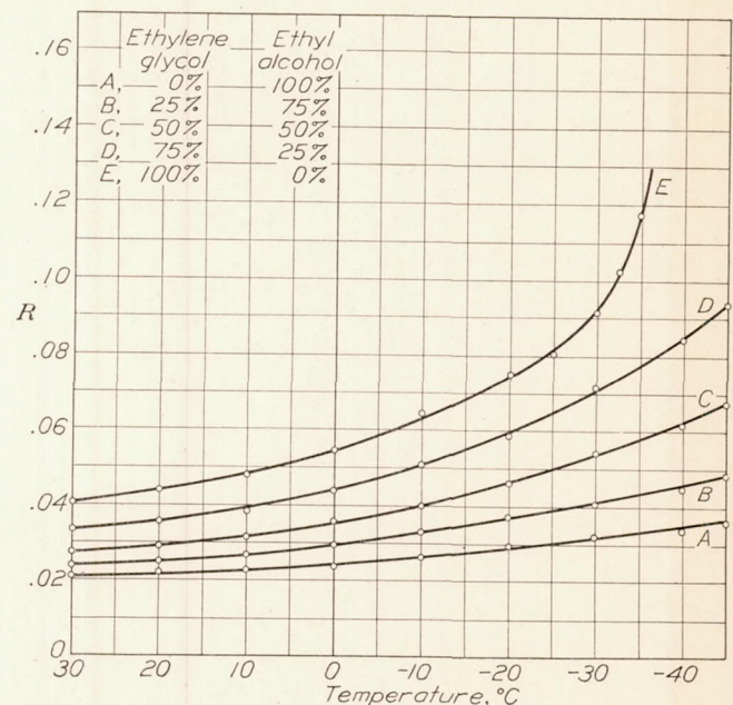
FIGURE 20.—Effect of temperature on the thermal coefficient R of kinematic viscosity of ethylene glycol-ethyl alcohol solutions. R is the relative change in kinematic viscosity per degree centigrade. Similar curves are obtained for the other liquids of the alcohol group
