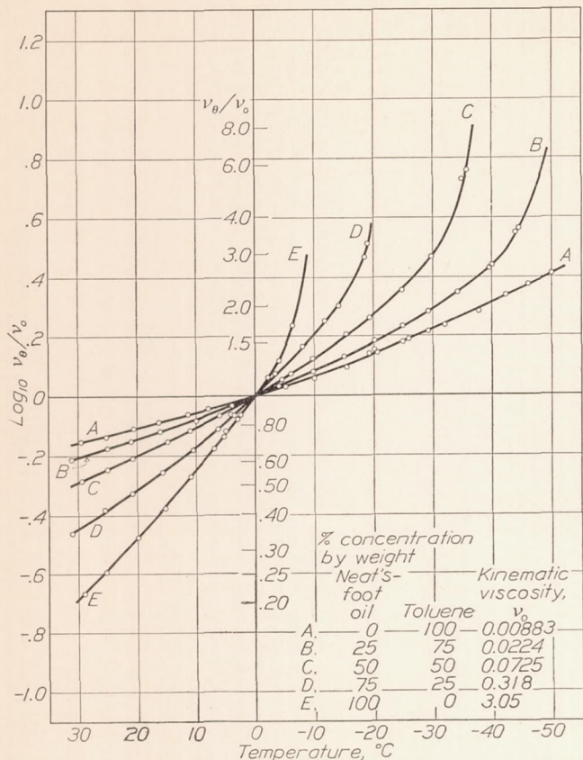
FIGURE 4.—Effect of temperature on the kinematic viscosity of solutions of neat's-foot oil (20° F.) and toluene. v_\theta and v_0 are the kinematic viscosities of the liquid at a given temperature (designated by \theta ) and at 0° C.
