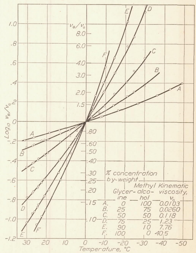
FIGURE 11.—Effect of temperature on the kinematic viscosity of solutions of glycerine and methyl alcohol. v_\theta and v_0 are the kinematic viscosities of the liquid at a given temperature (designated by \theta ) and at 0° C.
