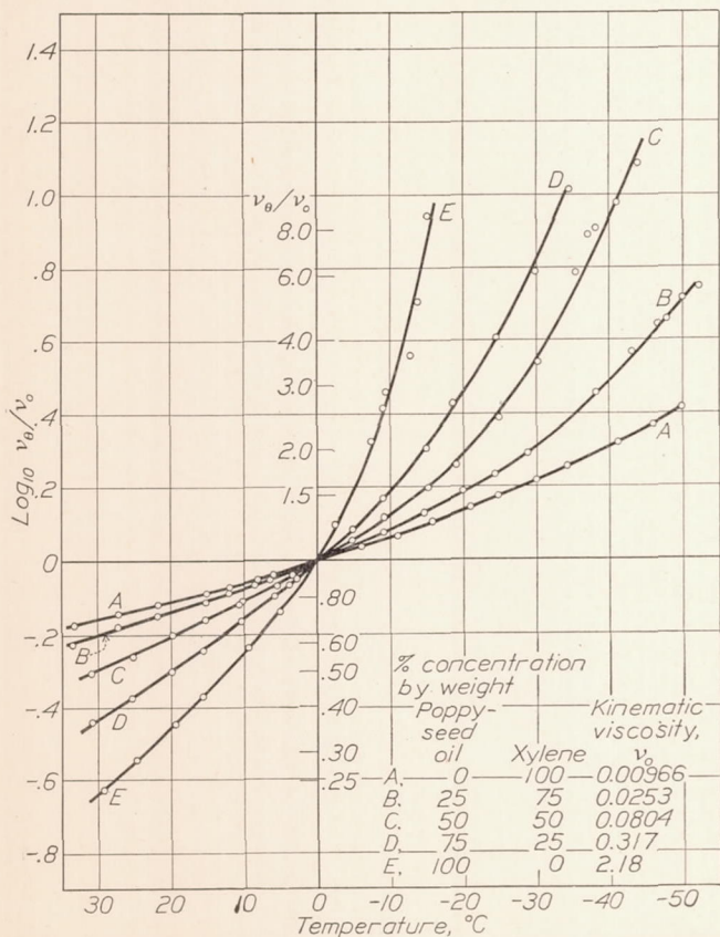
FIGURE 6.—Effect of temperature on the kinematic viscosity of solutions of poppy-seed oil and xylene. v_\theta and v_0 are the kinematic viscosities of the liquid at a given temperature (designated by \theta ) and at 0° C.
