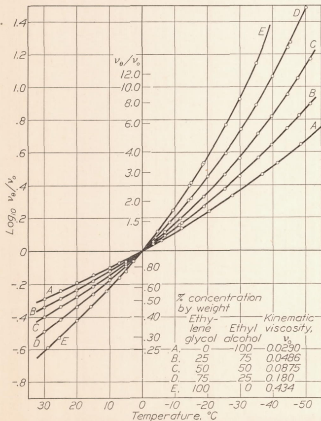
FIGURE 14.—Effect of temperature on the kinematic viscosity of solutions of ethylene glycol and ethyl alcohol. \nu_\theta and \nu_0 are the kinematic viscosities of the liquid at a given temperature (designated by \theta ) and at 0° C.
