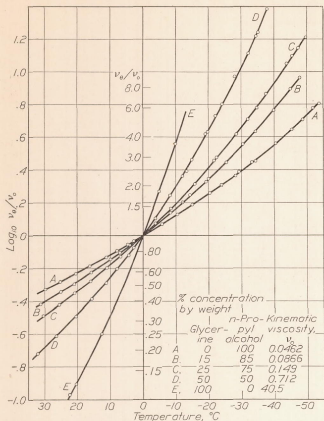
FIGURE 12.—Effect of temperature on the kinematic viscosity of solutions of glycerine and n-propyl alcohol. \nu_\theta and \nu_0 are the kinematic viscosities of the liquid at a given temperature (designated by \theta ) and at 0° C.
