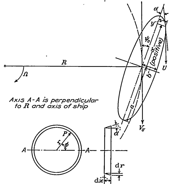
FIGURE 2.—Geometrical notation
