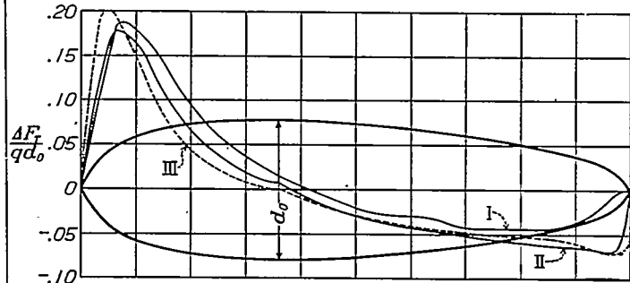
FIGURE 6.—Transverse force on model RS-1 ( \theta=9^\circ ). I. Transverse force from wind tunnel tests by Bureau of Standards (Technical Data Files, McCook Field, DE27/RS-1). II= \Delta F_T = q \times \frac{dS}{dX} \times \sin 2\theta \cos^2 \alpha (corrected for hydrodynamic balance.) III= \Delta F_T = q \times \frac{dS}{dX} (k_2 - k_1) \times \sin 2\theta Munk's formula ( k_2 - k_1 = 0.73 )
