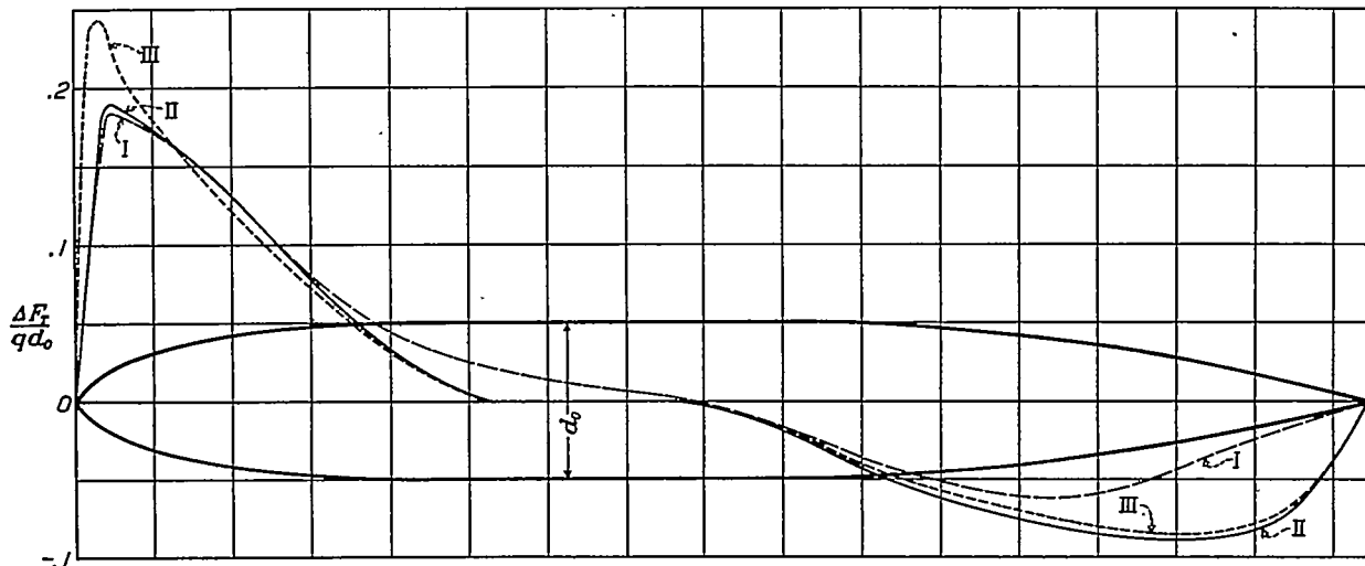
FIGURE 7.—Transverse force on model R-33 ( \theta=10^\circ ). I. Transverse force from wind tunnel tests (A. R. O.; R & M No. 801); II= \Delta F_T = q \times \frac{dS}{dX} \times \sin 2\theta \cos^2 \alpha ; III= \Delta F_T = q \times \frac{dS}{dX} (k_2 - k_1) \sin 2\theta Munk's formula ( k_2 - k_1 = .924 )
