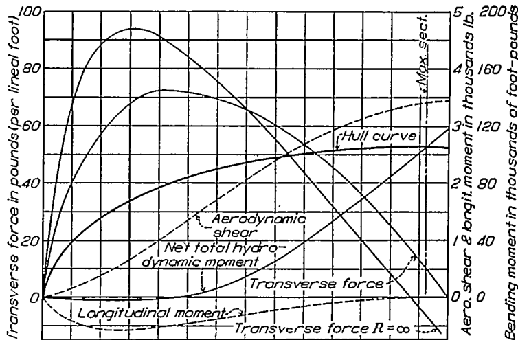
FIGURE 9.—Circular flight. Hydrodynamic loads, shears, and moments—Bow ZMC-8 ( \psi=10^\circ , v=50 m. p. h., R=600 feet)
