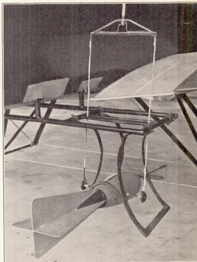
FIGURE 2.—Swivel suspension for flight-path-angle and air-speed recorder
