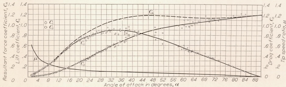
FIGURE 3.—Characteristic curves for PCA-2 autogiro
