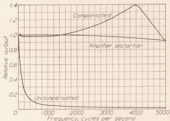
FIGURE 11.—Frequency characteristic of amplifier and hot wire
