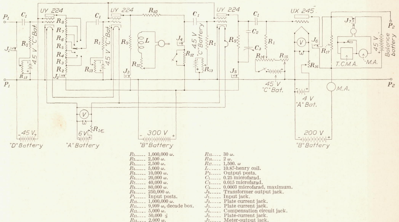
FIGURE 8.—Circuit of audio-frequency amplifier for turbulence measurement
