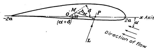
FIGURE 17.—Moment arm from M onto the lift vector
