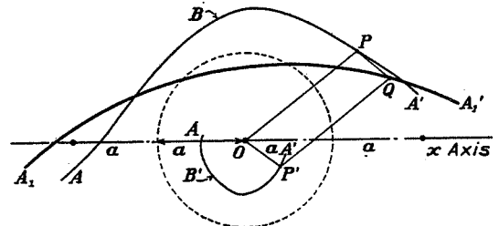
FIGURE 21.—Discontinuous B curve
