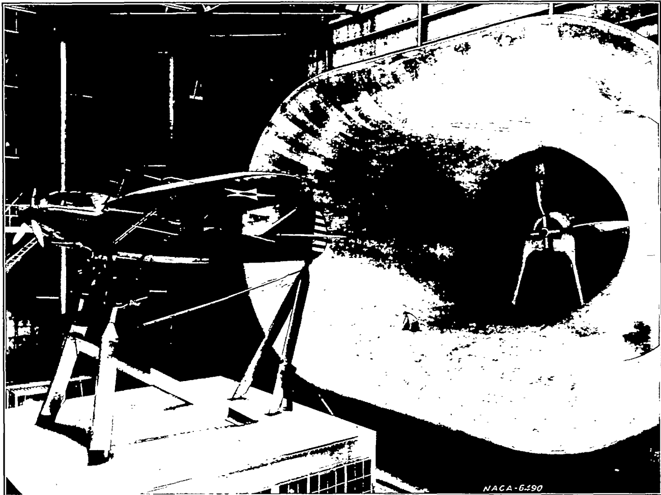
FIGURE 4.—The YO-31A airplanes ready for test in the tunnel.
