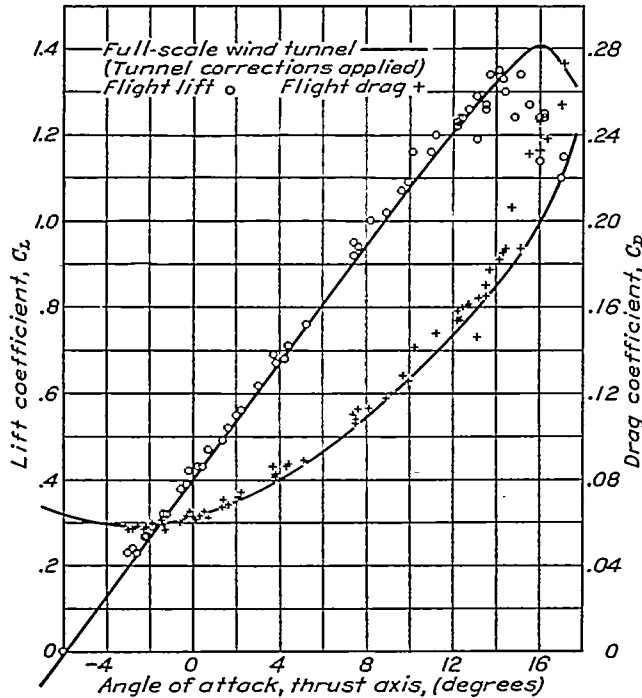
FIGURE 7.—Lift and drag characteristics of the F-23 airplane.
