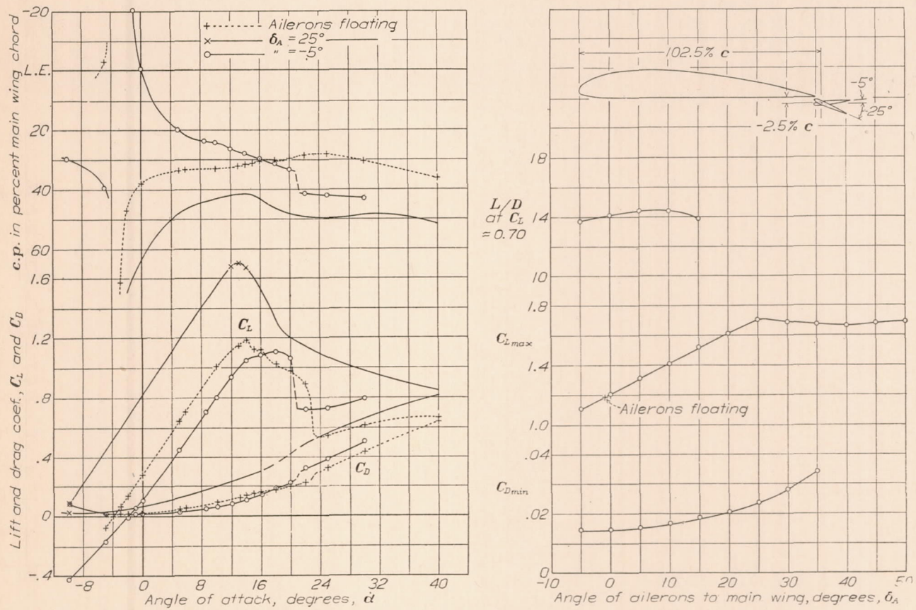
FIGURE 26.—Lift, drag, and center of pressure of Clark Y wing with external ailerons in position 37. The coordinates of all points on the curves for \delta_A = 25^\circ not marked (x) are interpolated from data obtained at \delta_A = 20^\circ and 30^\circ .
