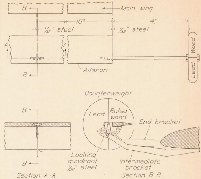
FIGURE 2.—External aileron mounting details.
