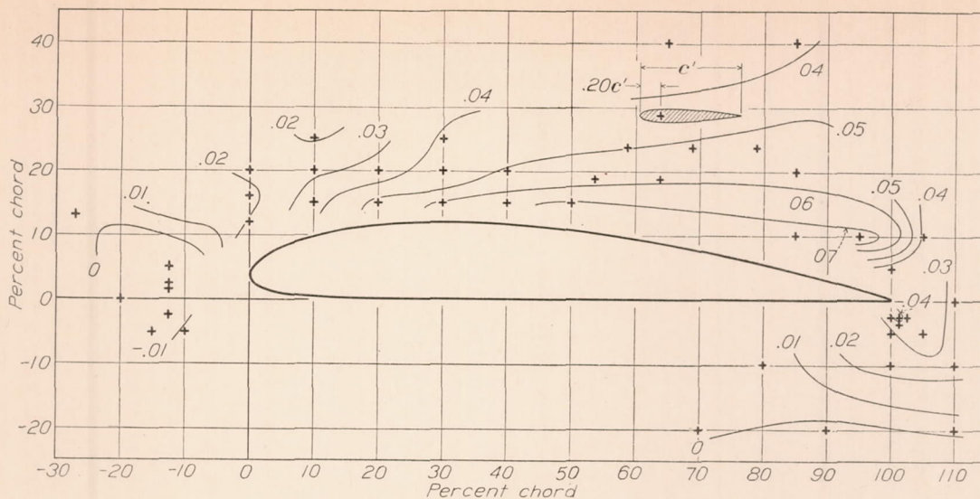
FIGURE 8.—Effect of location of external ailerons on C_l' . Right aileron deflected up-only. \alpha=0^\circ .
