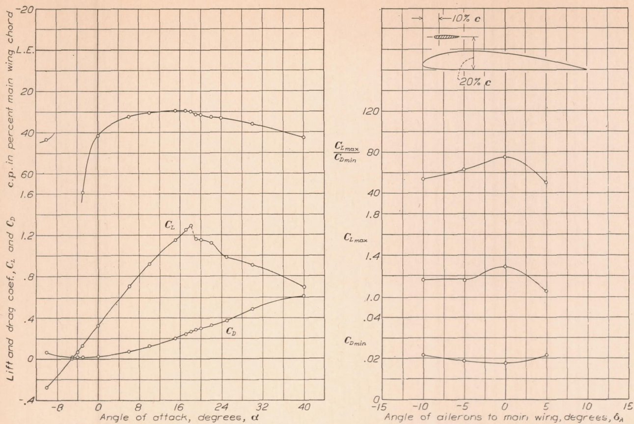
FIGURE 22.—Lift, drag, and center of pressure of Clark Y wing with symmetrical external ailerons in position 6.
