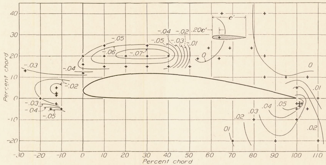
FIGURE 15.—Effect of location of external ailerons on C_l' . Left aileron deflected down-only. \alpha=10^\circ .
