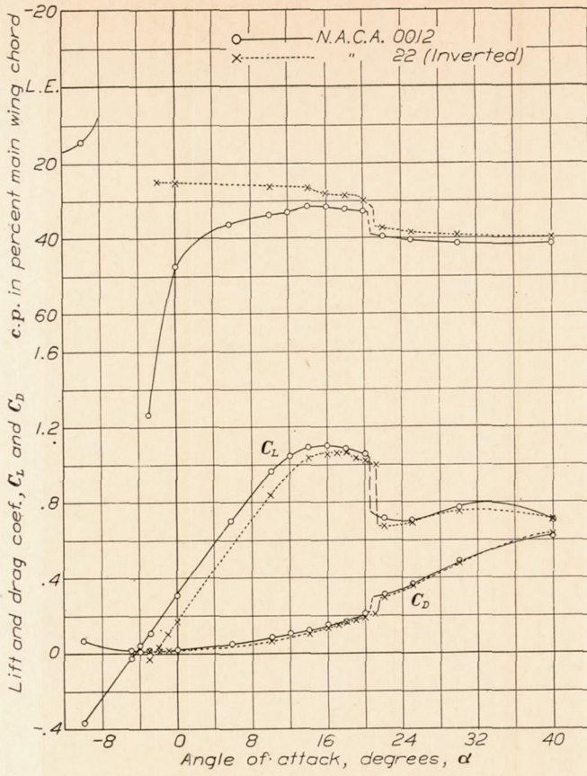
FIGURE 24.—Lift, drag, and center of pressure of Clark Y wing with symmetrical and cambered external ailerons in position 26.
