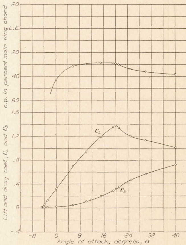
FIGURE 21.—Lift, drag, and center of pressure of Clark Y wing with symmetrical external ailerons in position 3.
