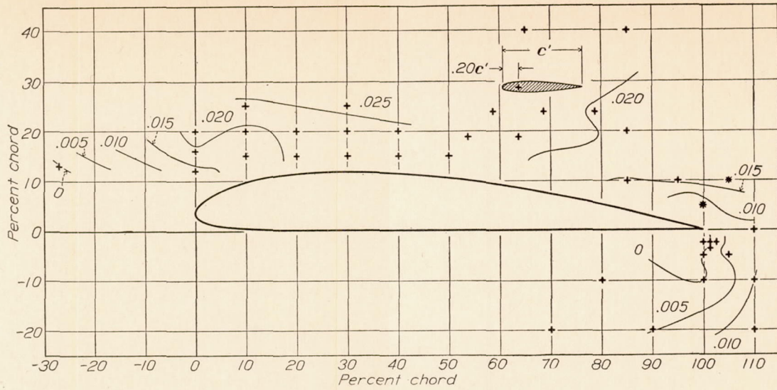
FIGURE 11.—Effect of location of external ailerons on C_L' . Right aileron deflected up-only. \alpha=0^\circ .
