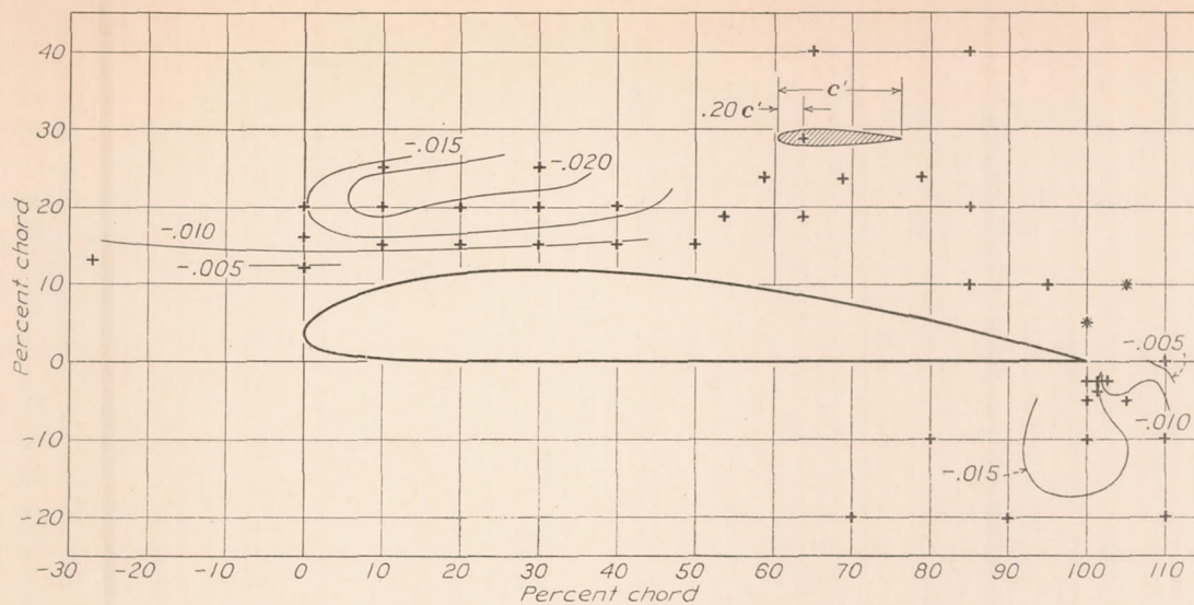
FIGURE 17.—Effect of location of external ailerons on C_n' . Left aileron deflected down-only. \alpha=0^\circ .
