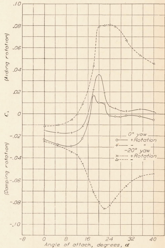
FIGURE 28.—Rolling moment due to rolling. p'b/2V=0.05 . Clark Y wing with symmetrical external ailerons in position 35. \delta_A=-5^\circ .
