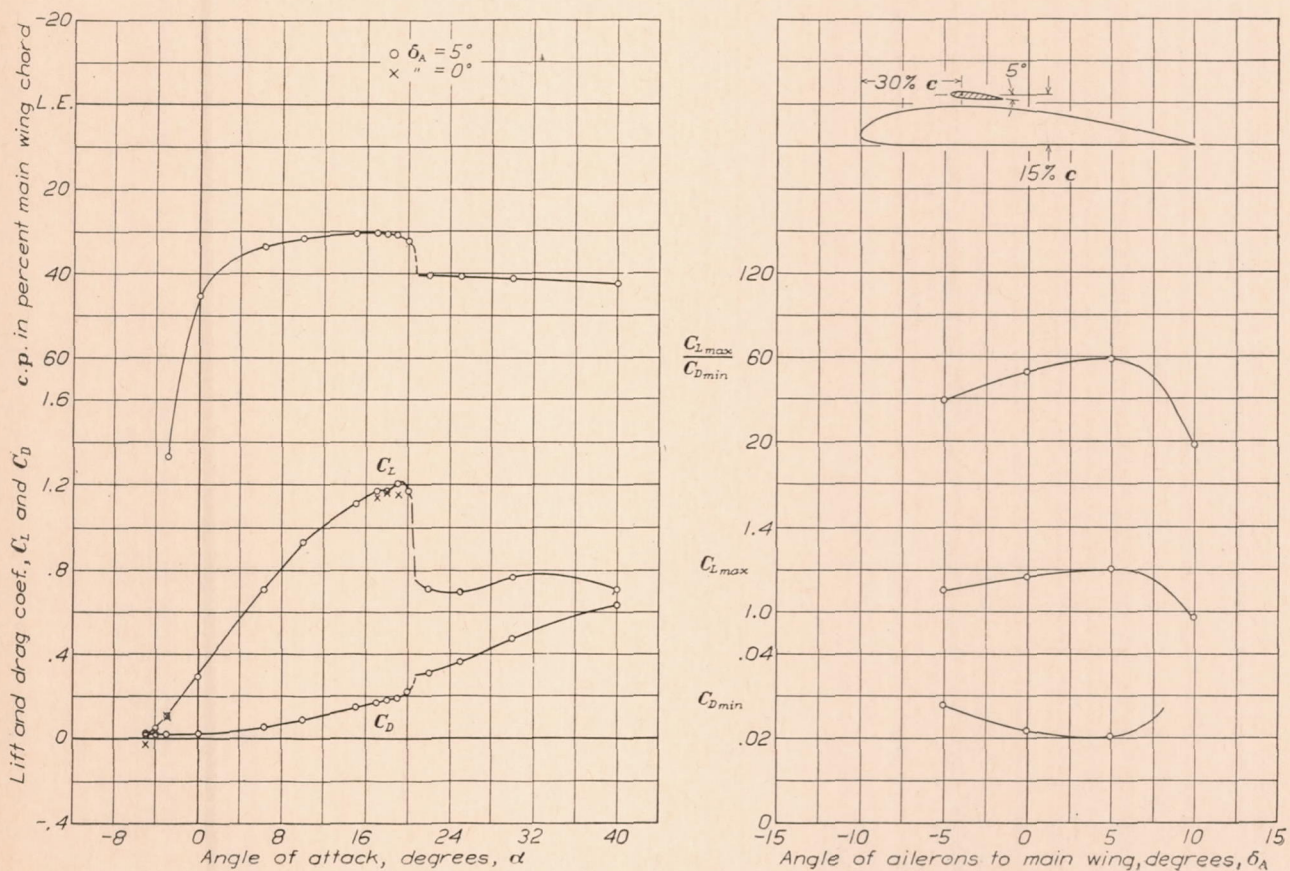
FIGURE 23.—Lift, drag, and center of pressure of Clark Y wing with symmetrical external ailerons in position 12.
