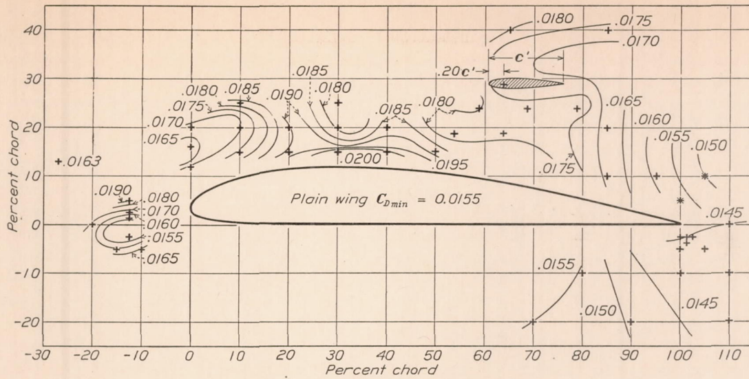
FIGURE 5.—Effect of location of external ailerons on C_{D_{min}} .
