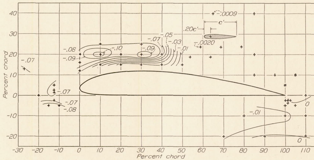
FIGURE 16.—Effect of location of external ailerons on C_l' . Left aileron deflected down-only. \alpha=20^\circ .
