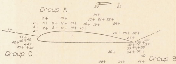
FIGURE 1.—External aileron test positions. Crosses indicate the location of the aileron axis (20 percent of the aileron chord from its leading edge).
