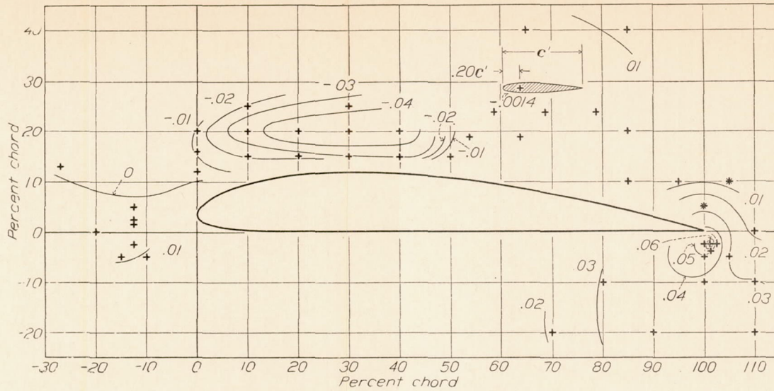
FIGURE 14.—Effect of location of external ailerons on C_l' . Left aileron deflected down-only. \alpha=0^\circ .
