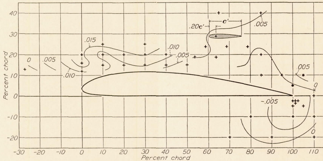
FIGURE 13.—Effect of location of external ailerons on C_L' . Right aileron deflected up-only. \alpha=20^\circ .
