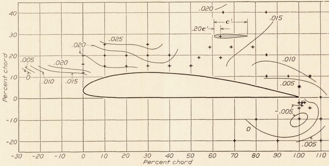
FIGURE 12.—Effect of location of external ailerons on C_m . Right aileron deflected up-only. \alpha=10^\circ .
