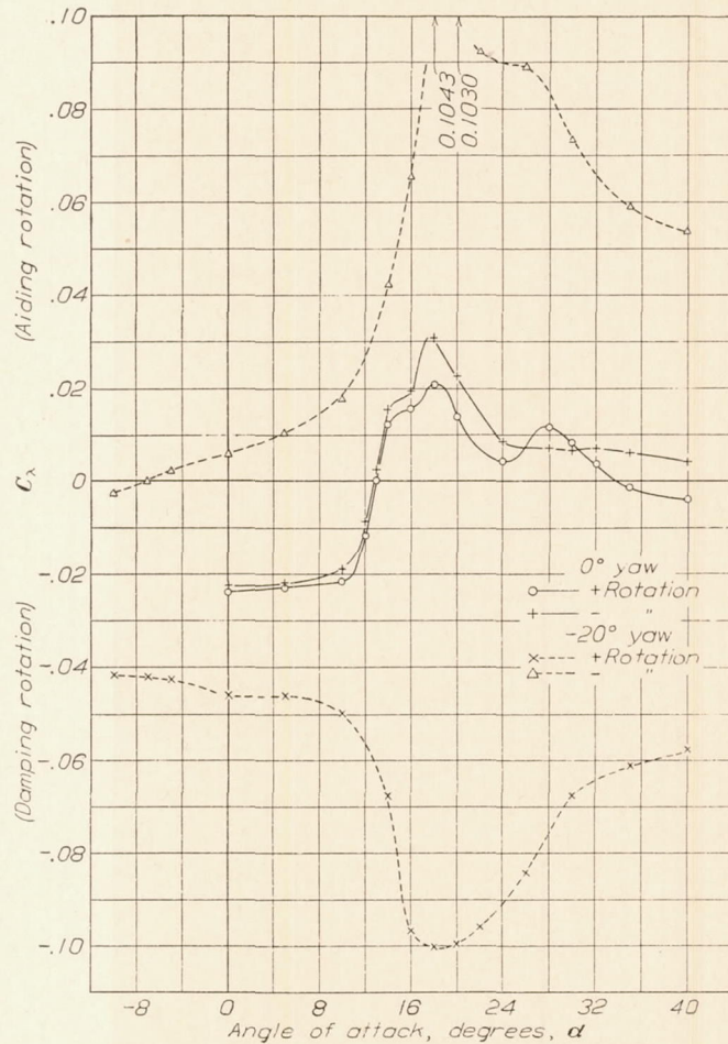
FIGURE 27.—Rolling moment due to rolling. p'b/2V=0.05 . Clark Y wing with no ailerons.
