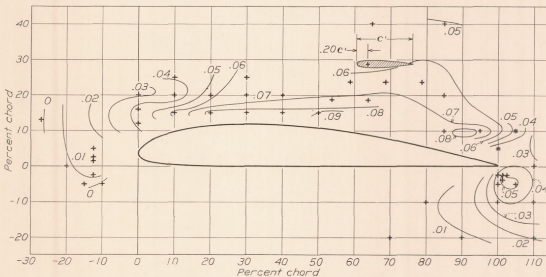
FIGURE 9.—Effect of location of external ailerons on C_l' . Right aileron deflected up-only. \alpha=10^\circ .
