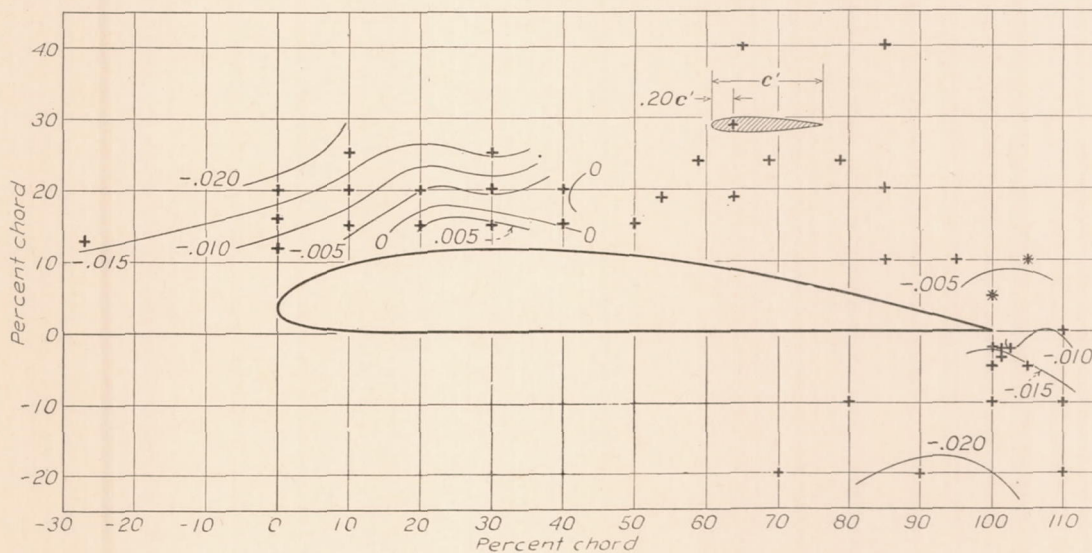
FIGURE 19.—Effect of location of external ailerons on C_n' . Left aileron deflected down-only. \alpha=20^\circ .
