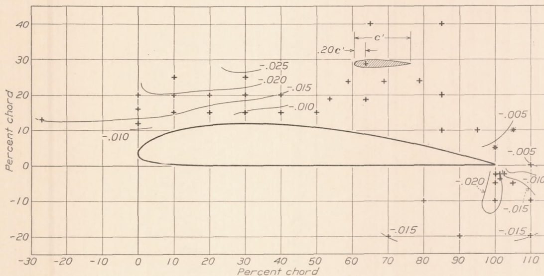
FIGURE 18.—Effect of location of external ailerons on C_n' . Left aileron deflected down-only. \alpha=10^\circ .
