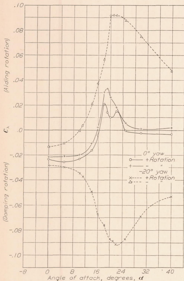
FIGURE 29.—Rolling moment due to rolling. p'b/2V=0.05 . Clark Y wing with symmetrical external ailerons in position 35. \delta_A=45^\circ .
