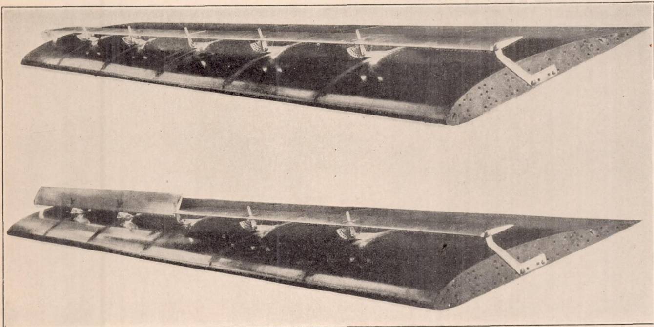
FIGURE 3.—Wing model with external ailerons mounted in position 6.
