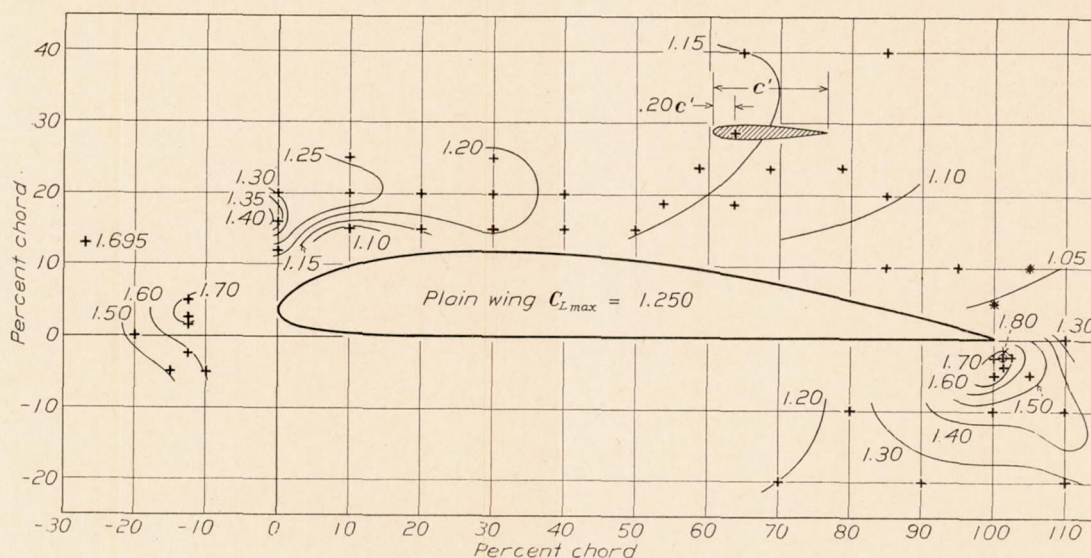
FIGURE 4.—Effect of location of external ailerons on C_{L_{max}} .
