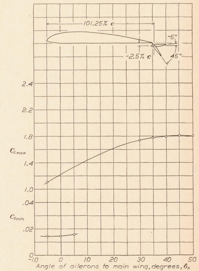
FIGURE 25.—Lift, drag, and center of pressure of Clark Y wing with symmetrical external ailerons in position 35.
