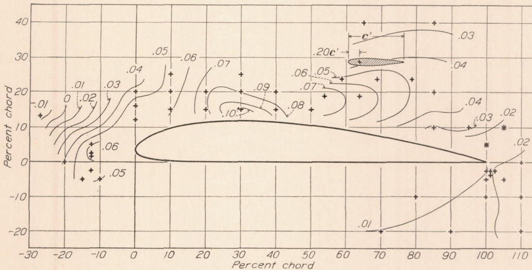
FIGURE 10.—Effect of location of external ailerons on C_l' . Right aileron deflected up-only. \alpha=20^\circ .
