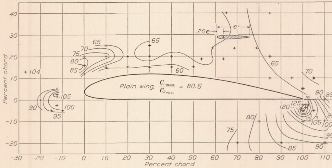
FIGURE 6.—Effect of location of external ailerons on the ratio C_{L_{max}}/C_{D_{min}} .
