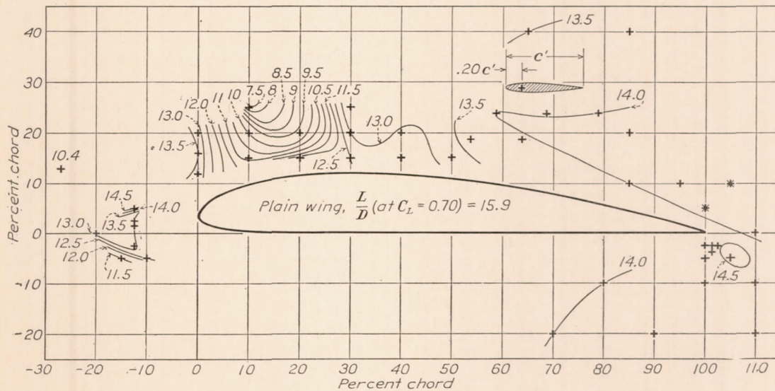
FIGURE 7.—Effect of location of external ailerons on the L/D ratio at C_L=0.70 (rate-of-climb criterion).
