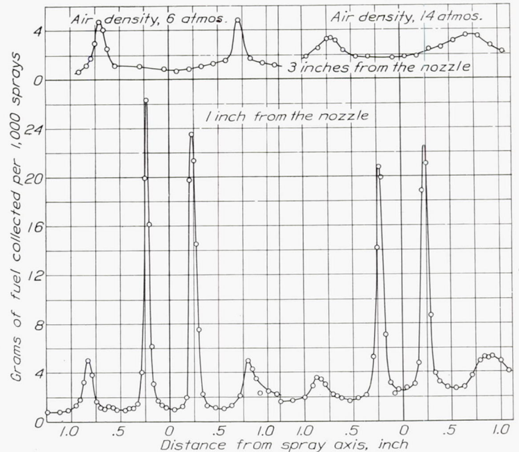
FIGURE 13.—Sampling-tube tests with a multiple-orifice nozzle.
