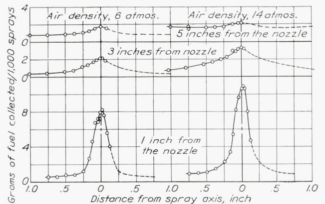
FIGURE 15.—Sampling-tube tests with a centrifugal nozzle.
