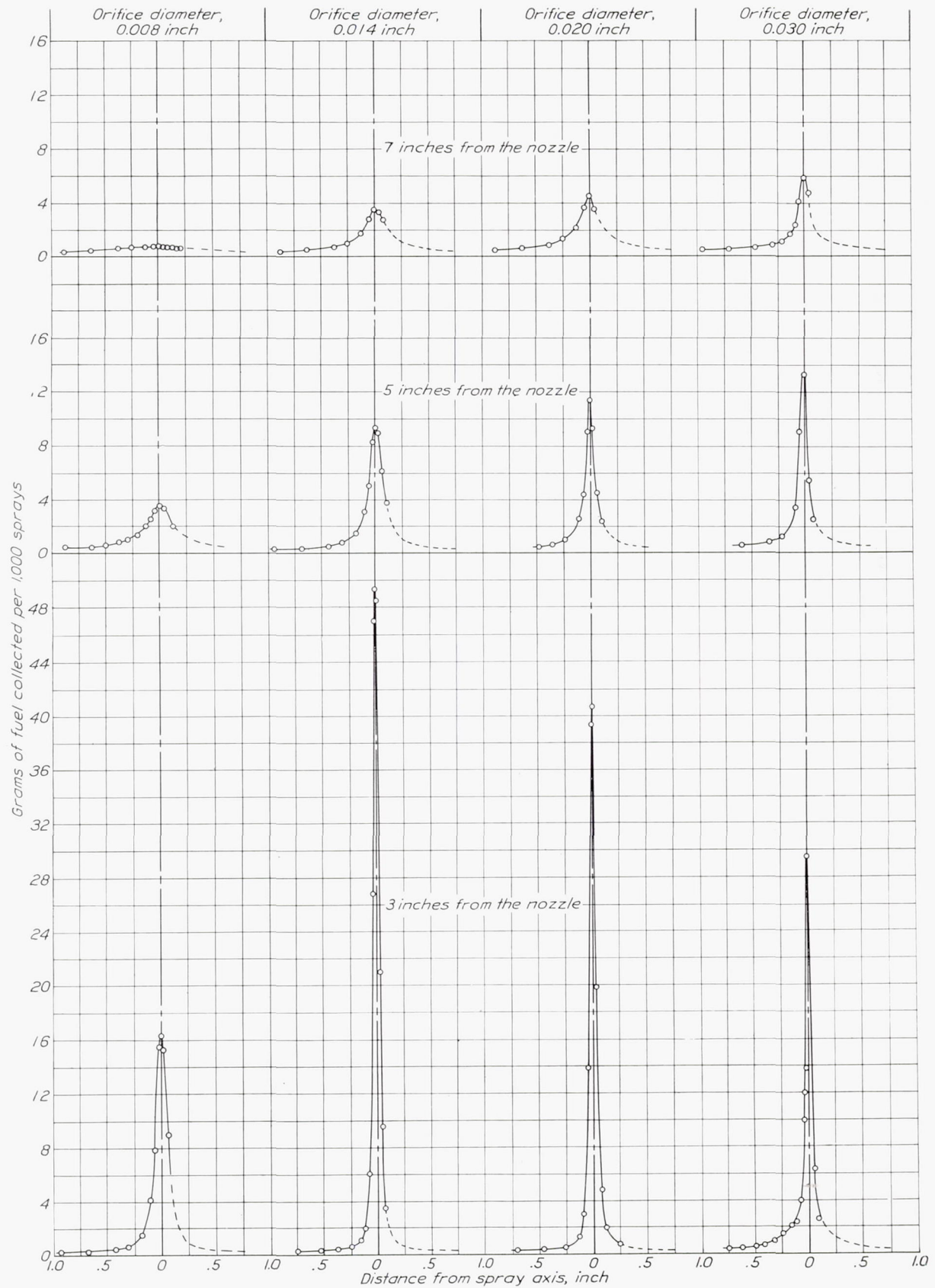
FIGURE 5.—Sampling-tube tests with plain nozzles having different orifice diameters. Orifice length-diameter ratio, 2; air density, 6 atmospheres.
