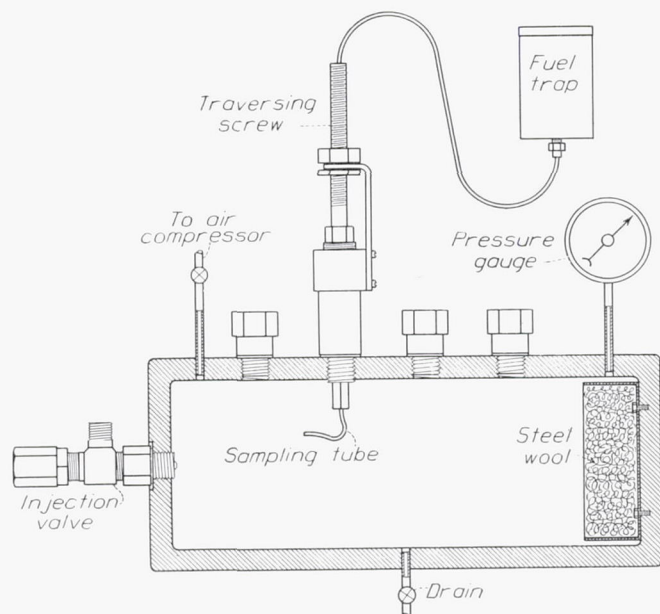
FIGURE 1.—Sampling-tube apparatus.
