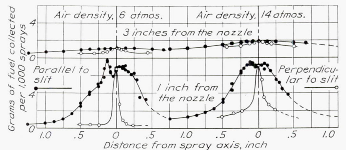
FIGURE 14.—Sampling-tube tests with a slit nozzle.
