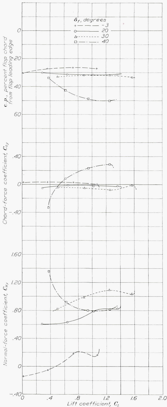
FIGURE 23.—Variation of air loads on flap with wing lift coefficient. N. A. C. A. 23012 airfoil with 0.20c w N. A. C. A. 23012 external-airfoil flap.
