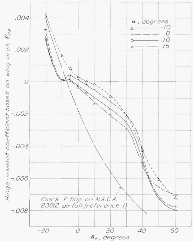
FIGURE 24.—Hinge-moment coefficients of flap. Hinge axis 1. N. A. C. A. 23012 airfoil with 0.20c w N. A. C. A. 23012 external-airfoil flap.
