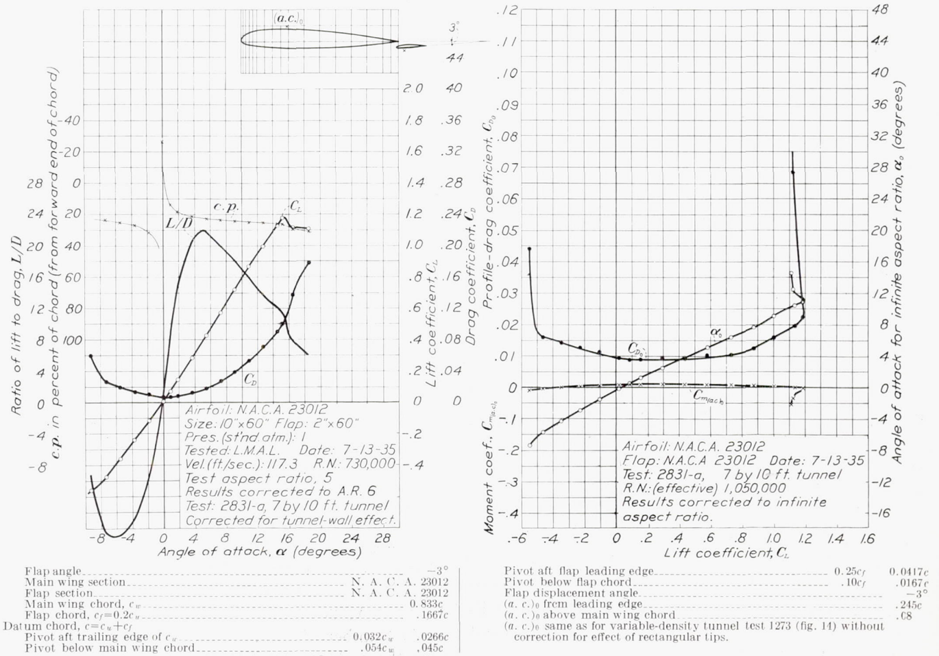
FIGURE 6.—The N. A. C. A. 23012 airfoil with 0.20 w N. A. C. A. 23012 external-airfoil flap.
