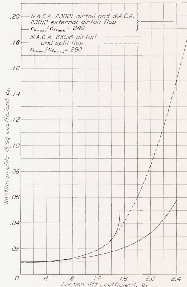
FIGURE 27.—Comparison of N. A. C. A. 23021 airfoil and 0.20c_w N. A. C. A. 23012 external-airfoil flap with N. A. C. A. 23018 airfoil and 0.20c_w split flap. Effective Reynolds Number, 8,200,000.
