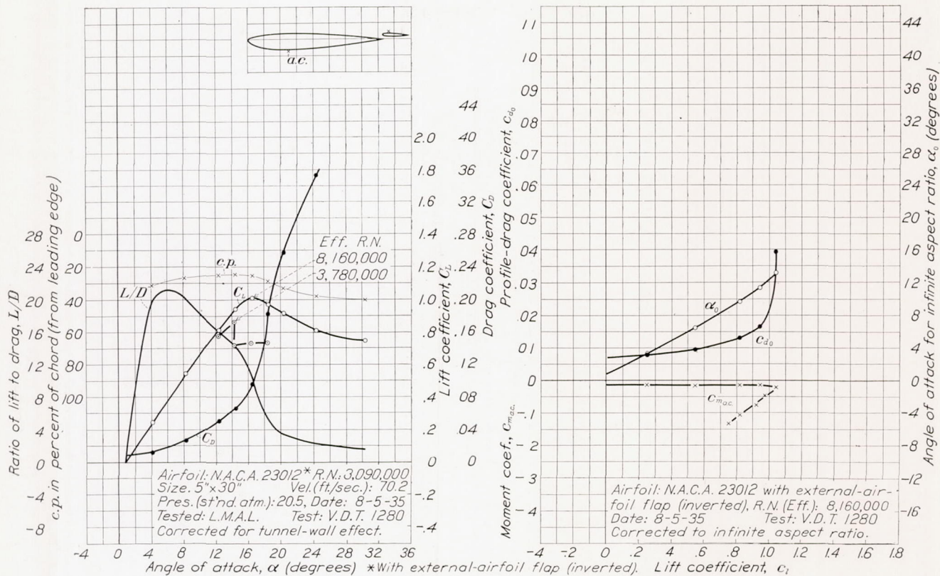
FIGURE 15.—The N. A. C. A. 23012 airfoil with 0.20c N. A. C. A. 23012 external-airfoil flap. Flap angle, -3^\circ (inverted). The airfoil is the same as used for variable-density tunnel test 1273 (fig. 14) except inverted; a. c. from leading edge, 0.252c; a. c. above main wing chord, -0.07c .
