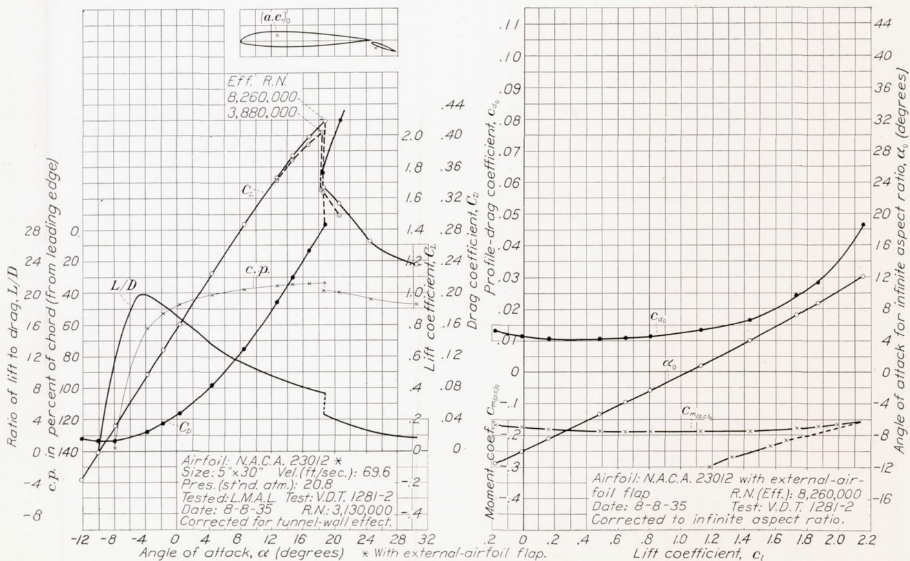
FIGURE 16.—The N. A. C. A. 23012 airfoil with 0.20c N. A. C. A. 23012 external-airfoil flap. Flap angle, 20^\circ . The airfoil is the same as used for variable-density tunnel test 1273 (fig. 14) except the flap setting. The value of c_{m(a.c.)_0} is computed about the aerodynamic center as determined for test 1273.
