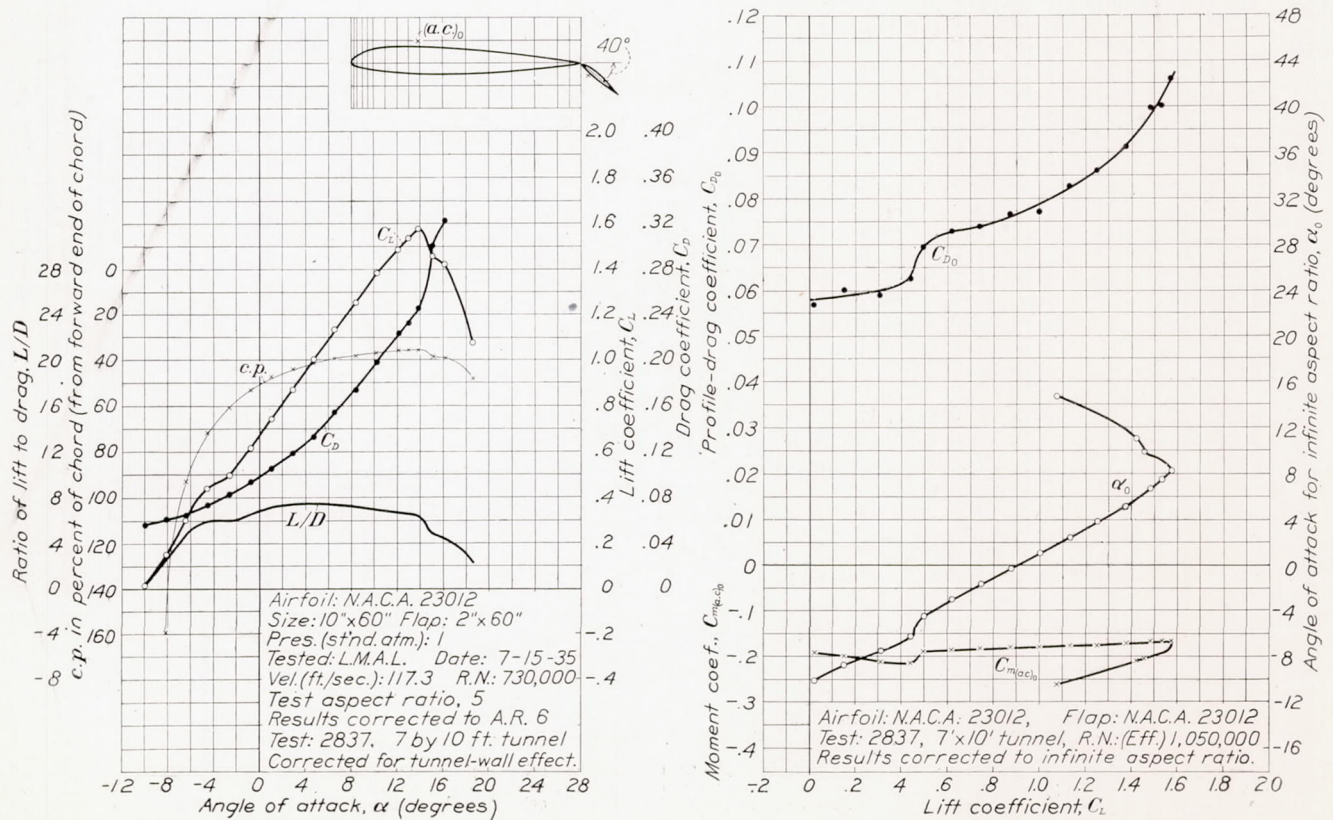
FIGURE 12.—The N. A. C. A. 23012 airfoil with 0.20c w N. A. C. A. 23012 external-airfoil flap. Flap angle, 40°. The airfoil is the same as used for test 2831-a (fig. 6) except the flap setting. The value of C_{m(a.c.)_0} is computed about the aerodynamic center used for test 2831-a.
