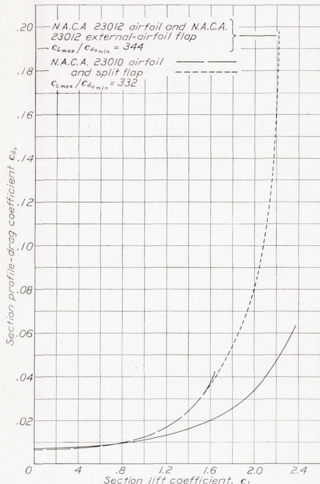
FIGURE 26.—Comparison of N. A. C. A. 23012 airfoil and 0.20c_w N. A. C. A. 23012 external-airfoil flap with N. A. C. A. 23010 airfoil and 0.20c_w split flap. Effective Reynolds Number, 8,200,000.
