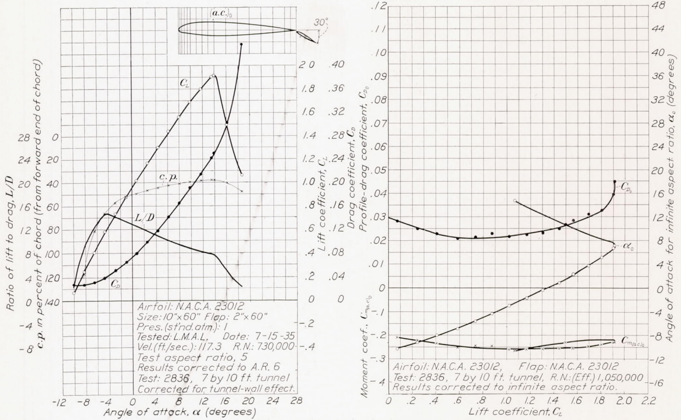
FIGURE 11.—The N. A. C. A. 23012 airfoil with 0.20c w N. A. C. A. 23012 external-airfoil flap. Flap angle, 30°. The airfoil is the same as used for test 2831-a (fig. 6) except the flap setting. The value of C_{m(a.c.)_0} is computed about the aerodynamic center used for test 2831-a.
