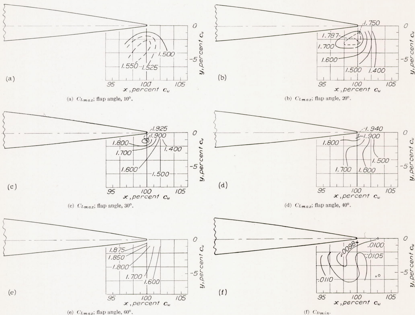
FIGURE 4.—Contours showing variation of C_{Lmax} and C_{Dmin} with flap position and angle. The N. A. C. A. 23012 airfoil with 0.20c_w N. A. C. A. 23012 external-airfoil flap. Plain wing: C_{Lmax} , 1.150; C_{Dmin} , 0.0103.
