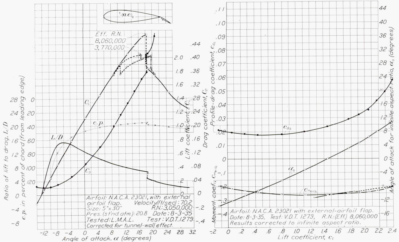
FIGURE 21.—The N. A. C. A. 23021 airfoil with 0.20c N. A. C. A. 23012 external-airfoil flap. Flap angle, 30°. The airfoil is the same as used for variable-density tunnel test 1274 (fig. 19) except the flap setting. The value of c_{m(a,c)_0} is computed about the aerodynamic center as determined for test 1274.
