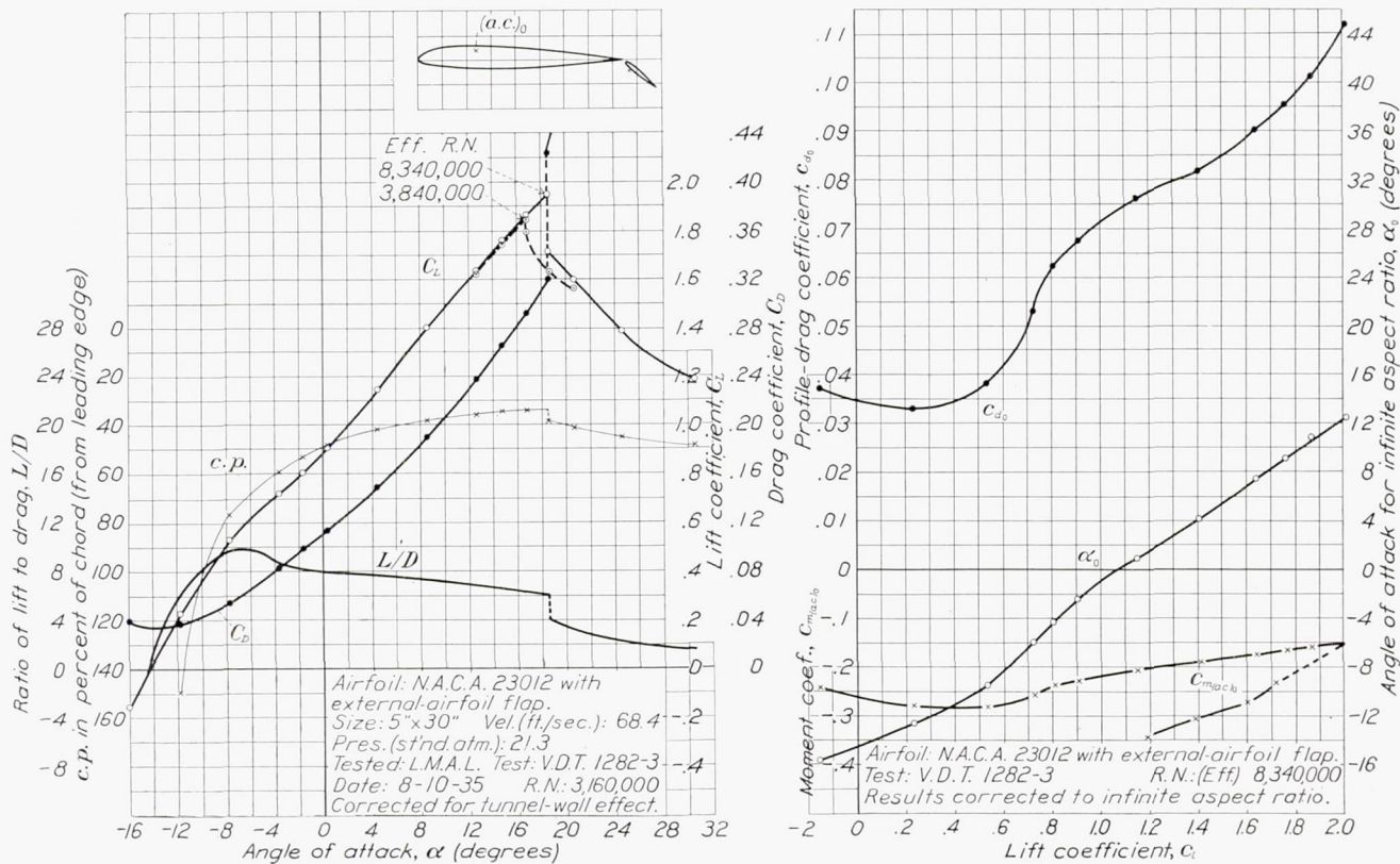
FIGURE 18.—The N. A. C. A. 23012 airfoil with 0.20c_w N. A. C. A. 23012 external-airfoil flap. Flap angle, 40^\circ . The airfoil is the same as used for variable-density tunnel test 1273 (fig. 14) except the flap setting. The value of c_{m(a.c.)_0} is computed about the aerodynamic center as determined for test 1273.
