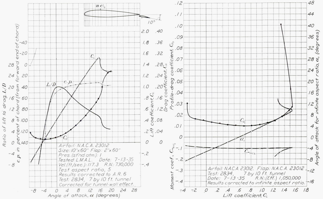
FIGURE 9.—The N. A. C. A. 23012 airfoil with 0.20c w N. A. C. A. 23012 external-airfoil flap. Flap angle, 10°. The airfoil is the same as used for test 2831-a (fig. 6), except the flap setting. The value of C_{m_{(a.c.)_0}} is computed about the aerodynamic center used for test 2831-a.
