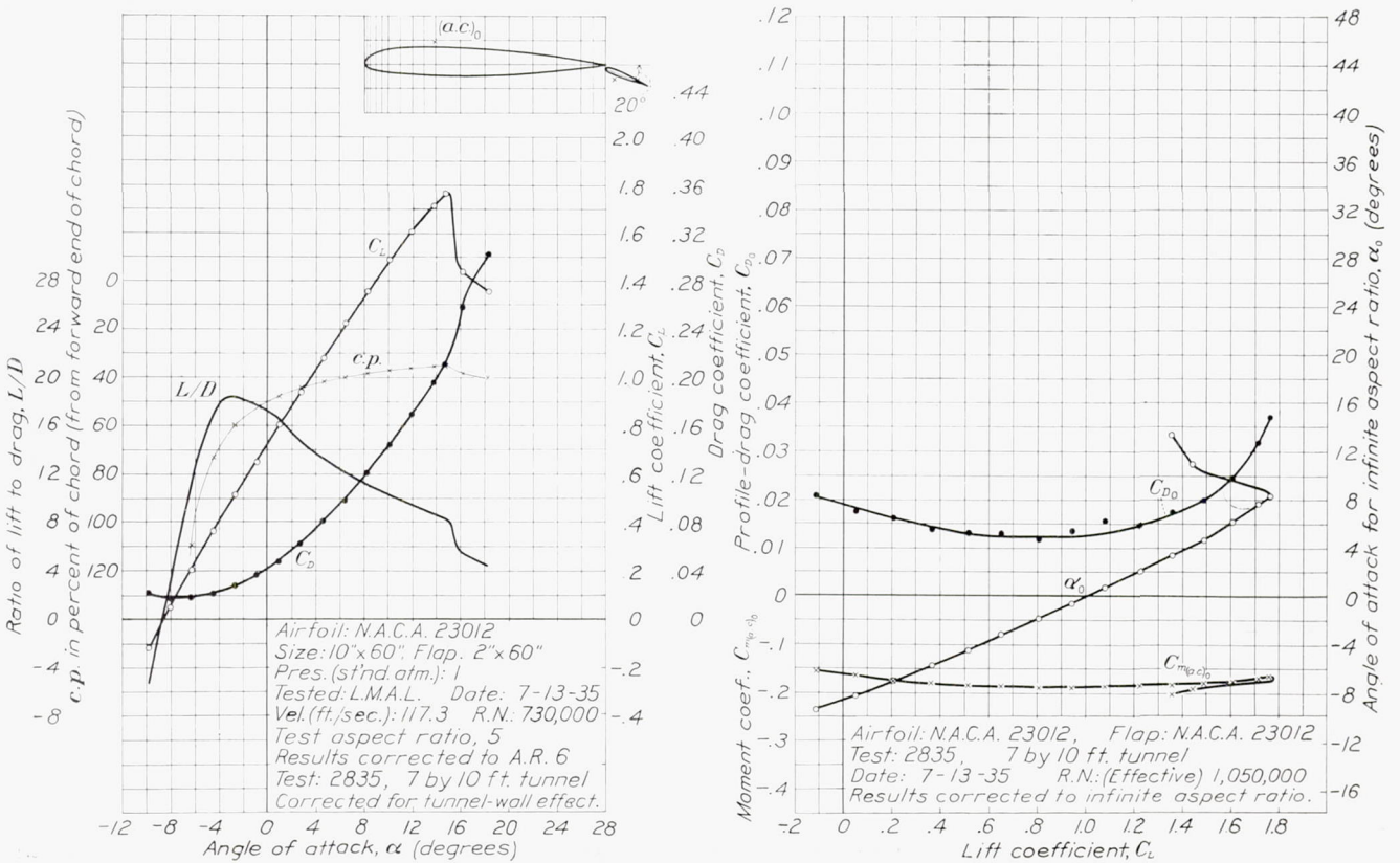
FIGURE 10.—The N. A. C. A. 23012 airfoil with 0.20c w N. A. C. A. 23012 external-airfoil flap. Flap angle, 20°. The airfoil is the same as used for test 2831-a (fig. 6), except the flap setting. The value of C_{m_{(a.c.)_0}} is computed about the aerodynamic center used for test 2831-a.
