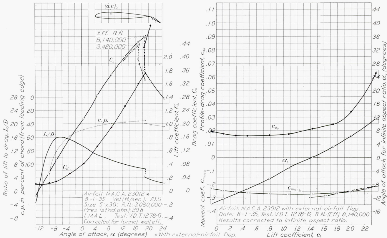
FIGURE 17.—The N. A. C. A. 23012 airfoil with 0.20c_w N. A. C. A. 23012 external-airfoil flap. Flap angle, 30^\circ . The airfoil is the same as used for variable-density tunnel test 1272 (fig. 14) except the flap setting. The value of c_{m(a.c.)_0} is computed about the aerodynamic center as determined for test 1273.
