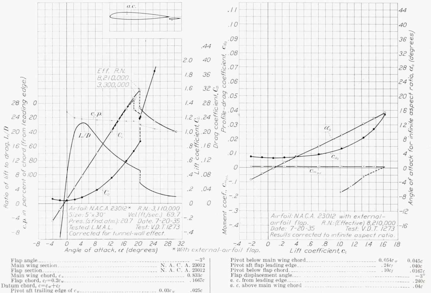
FIGURE 14.—The N. A. C. A. 23012 airfoil with 0.20c w N. A. C. A. 23012 external-airfoil flap.
