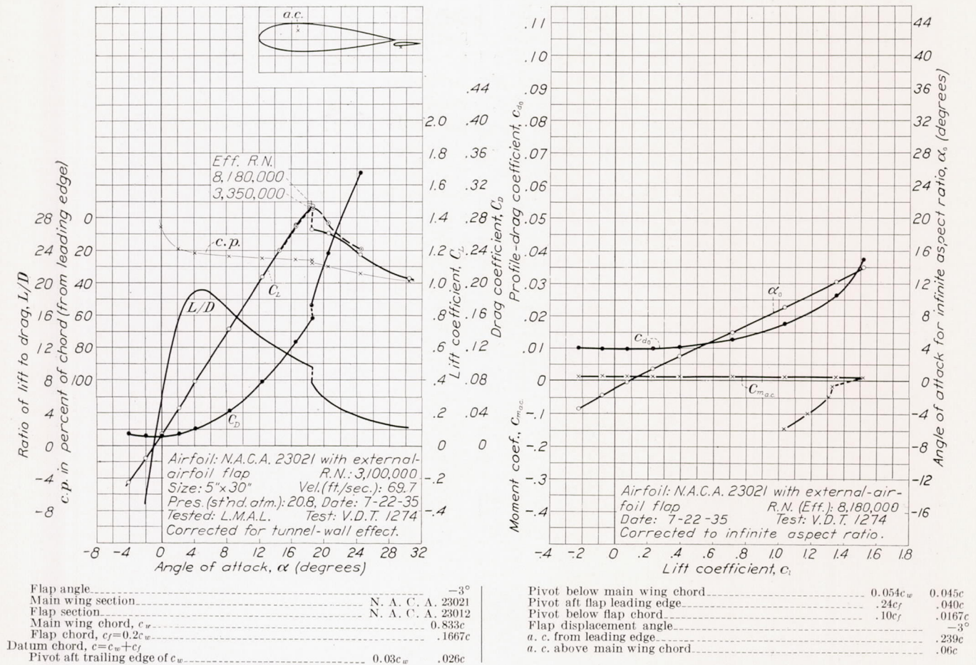
FIGURE 19.—The N. A. C. A. 23021 airfoil until 0.20 c_w N. A. C. A. 23012 external-airfoil flap.
