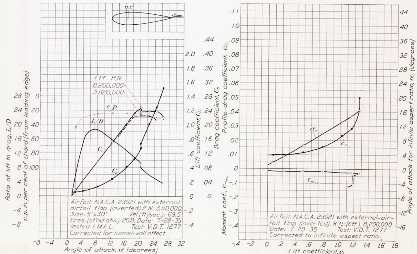
FIGURE 20.—The N. A. C. A. 23021 airfoil with 0.20 c_w N. A. C. A. 23012 external-airfoil flap. Flap angle, -3° (inverted). The airfoil is the same as used for variable-density tunnel test 1274 (fig. 19) except inverted; a. c. from leading edge, 0.217c; a. c. above main wing chord, -0.01c.
