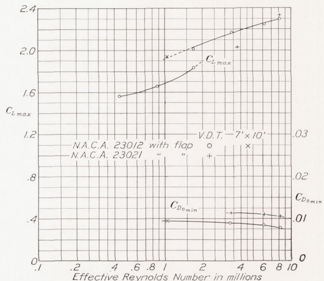
FIGURE 22.—Scale effect on N. A. C. A. 23012 and N. A. C. A. 23021 airfoils with 0.20c external-airfoil flap. All values uncorrected for hinge fares and for effects of rectangular tips.
