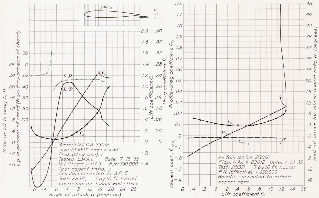
FIGURE 7.—The N. A. C. A. 23012 airfoil with 0.20c w N. A. C. A. 23012 external-airfoil flap. Flap angle, 0°. The airfoil is the same as used for test 2831-a (fig. 6) except the flap setting. The value of C m(a.c.) 0 is computed about the aerodynamic center used for test 2831-a.
