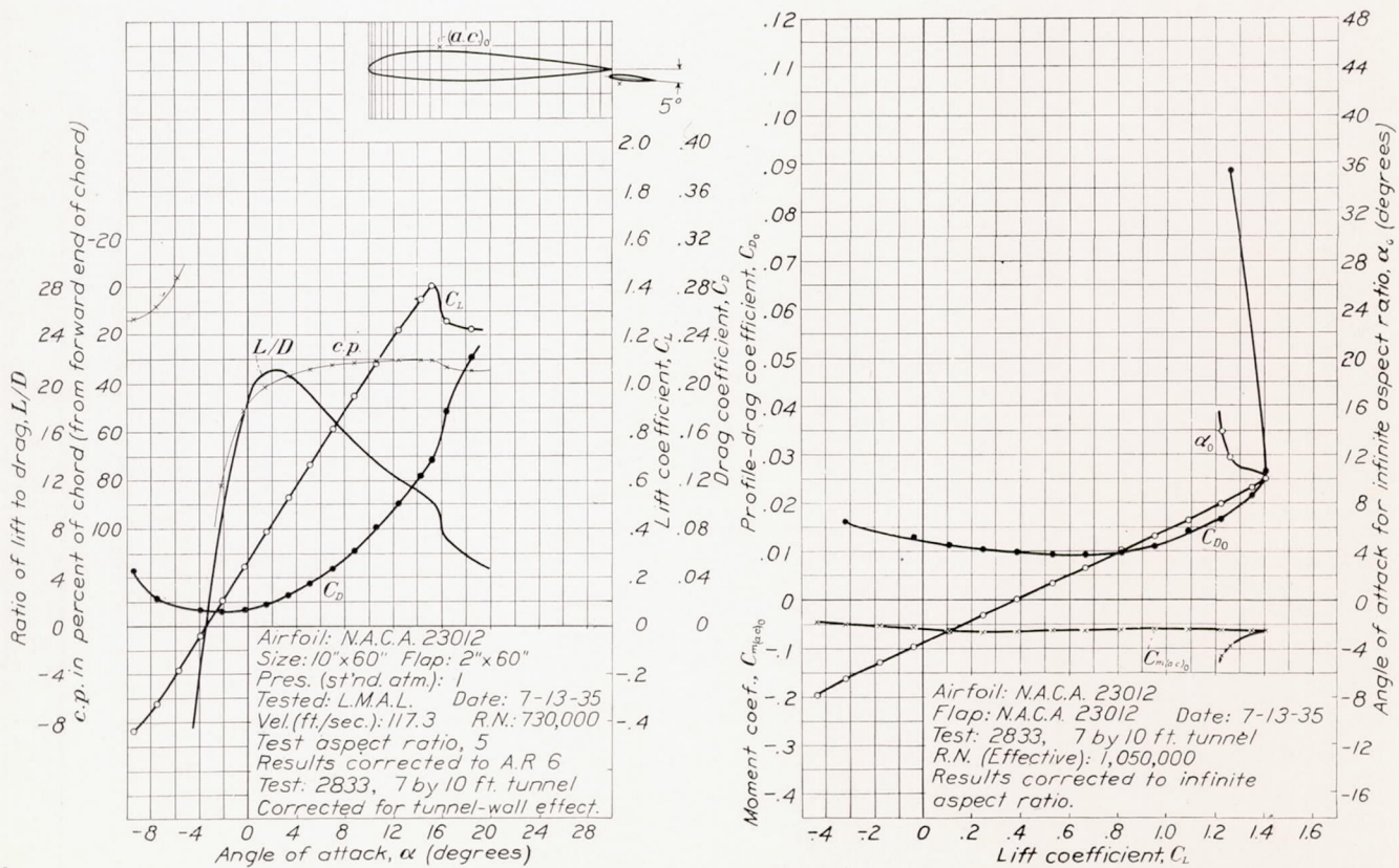
FIGURE 8.—The N. A. C. A. 23012 airfoil with 0.20c w N. A. C. A. 23012 external-airfoil flap. Flap angle, 5°. The airfoil is the same as used for test 2831-a (fig. 6), except the flap setting. The value of C m(a.c.) 0 is computed about the aerodynamic center used for test 2831-a.
