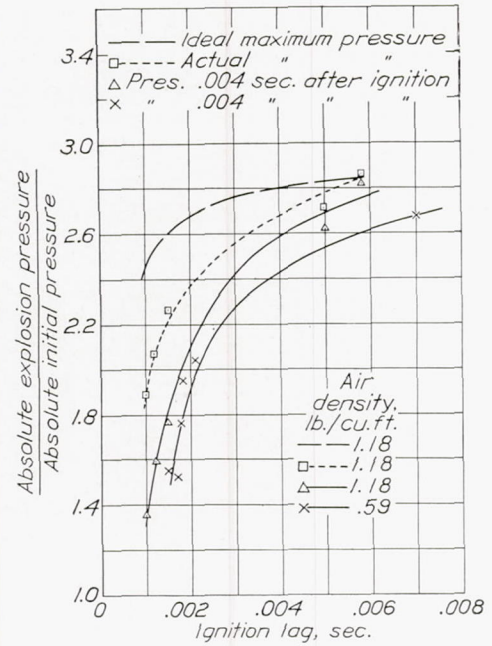
FIGURE 8.—Effect of ignition lag on combustion. Air-fuel ratio, 30.
