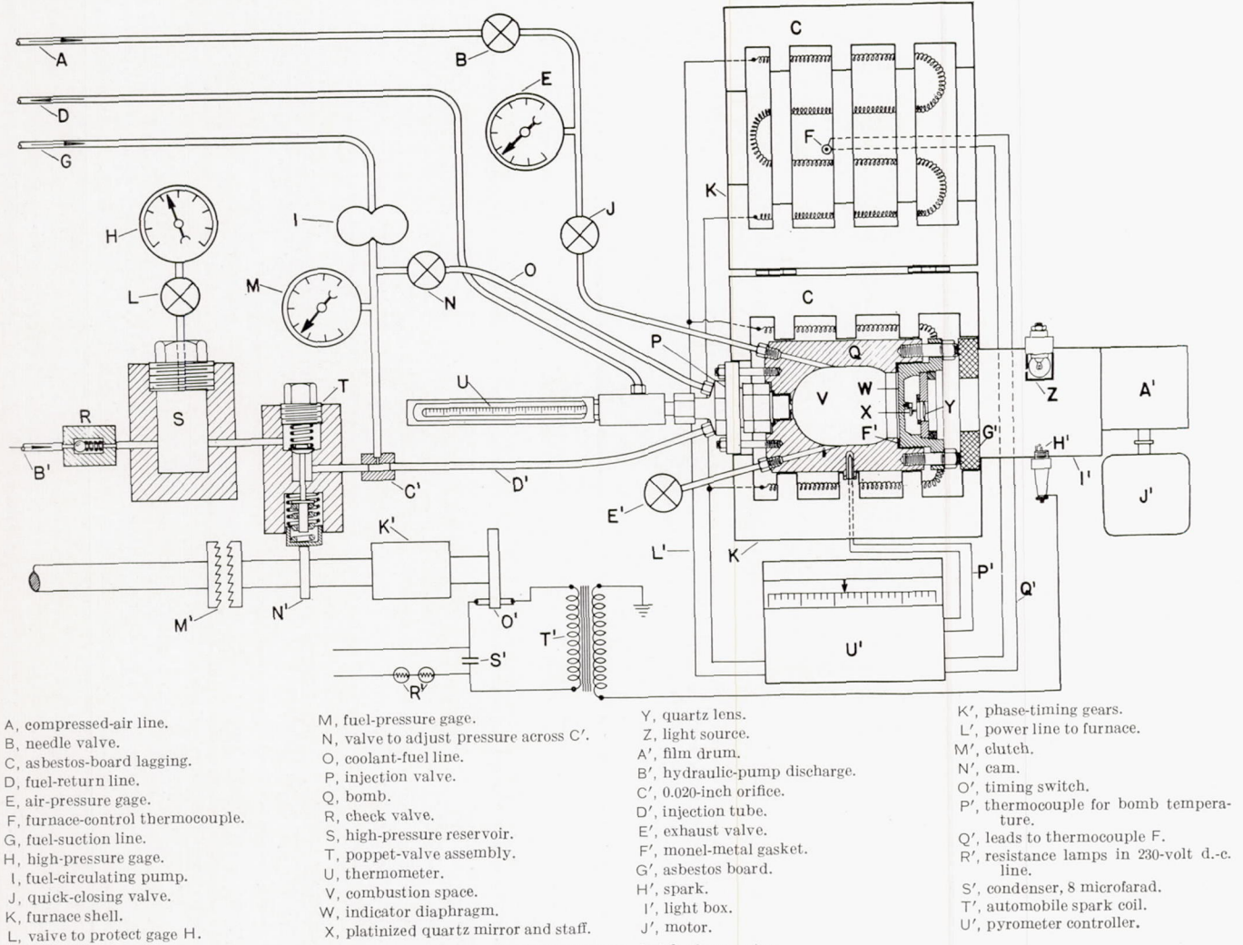
FIGURE 1.—Diagrammatic sketch of apparatus.
