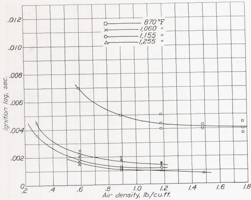
FIGURE 7.—Effect of air density on ignition lag. Variable air-fuel ratio.
