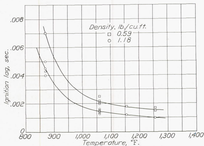
FIGURE 5.—Effect of temperature on ignition lag. Variable air-fuel ratio.
