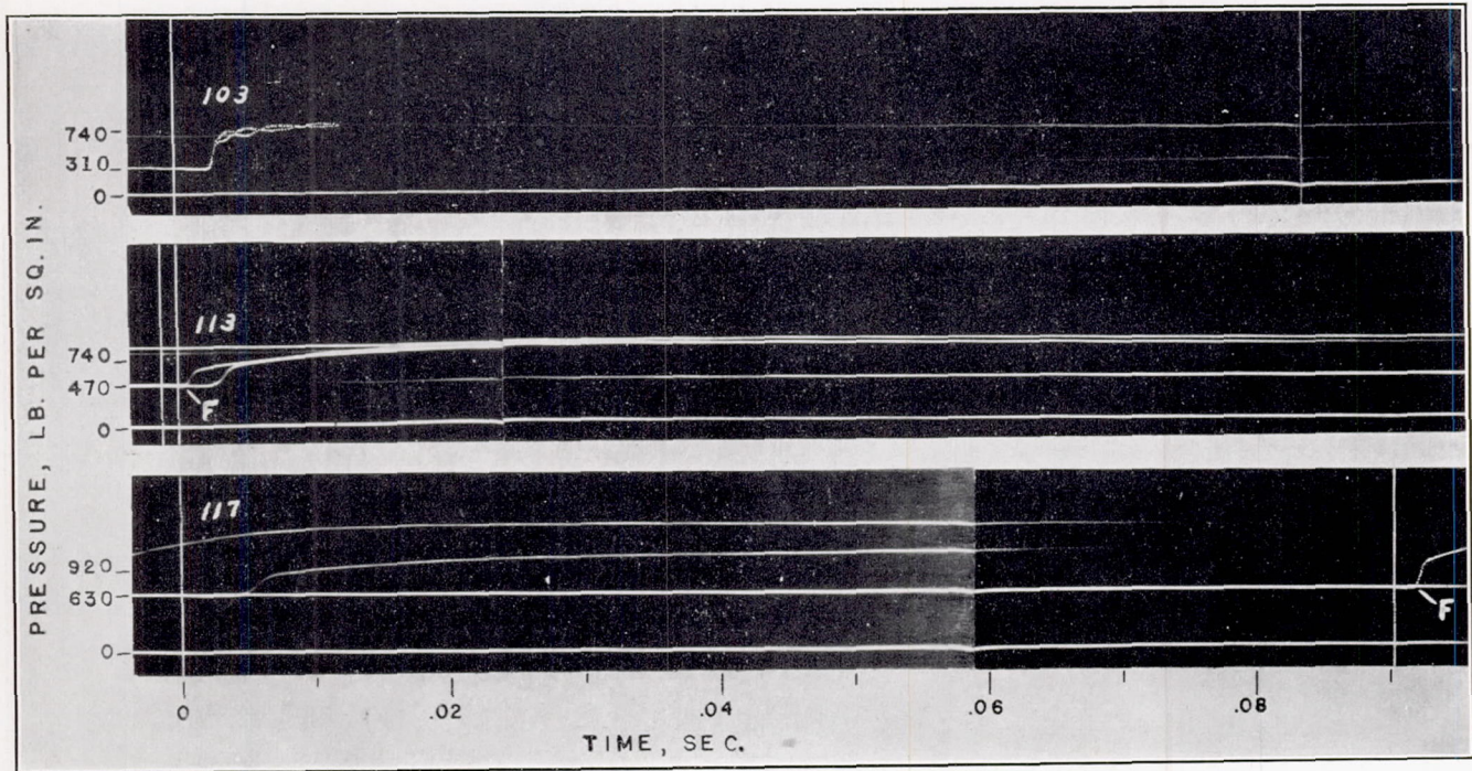
FIGURE 7.—Effect of air density on ignition lag. Variable air-fuel ratio.
