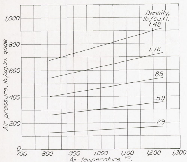
FIGURE 3.—Relations of temperature, pressure, and density.
