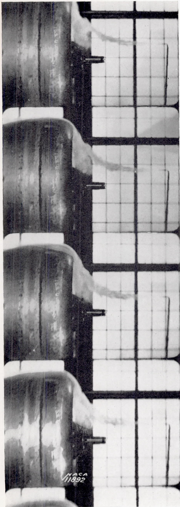
L. □ FIGURE 1.—Smoke flow over the nose of an N. A. C. A. cowling.
