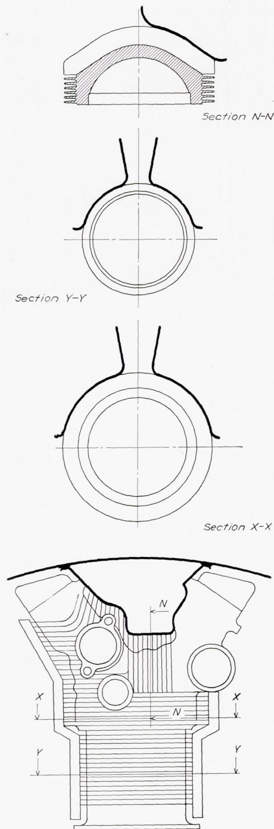
FIGURE 8.—Typical baffle design for a cylinder of a radial engine.
