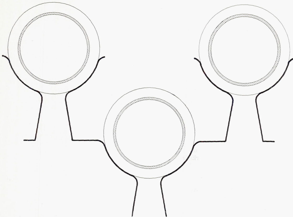
FIGURE 9.—Baffle design for a double-row radial engine.
