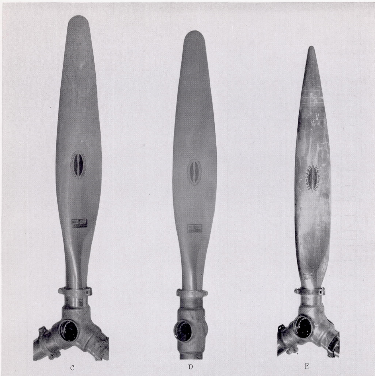
FIGURE 3.—The propellers used in this investigation.
