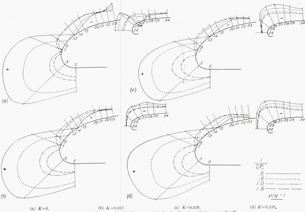
FIGURE 10.—Pressure distribution on nose 1, slot 2. Opening, 4\frac{1}{2} in.; propeller E.
