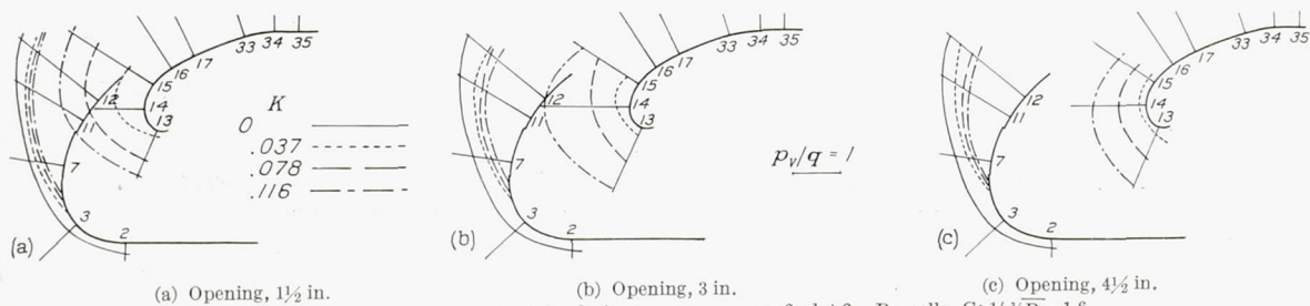
FIGURE 13.—Distribution of indicated velocity pressure on nose 2, slot 2. Propeller C; 1/\sqrt{P_c}=1.6 .
