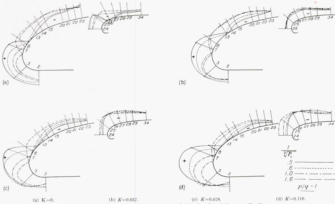
FIGURE 9.—Pressure distribution on nose 1, slot 2. Opening, 4\frac{1}{2} in.; propeller C.
