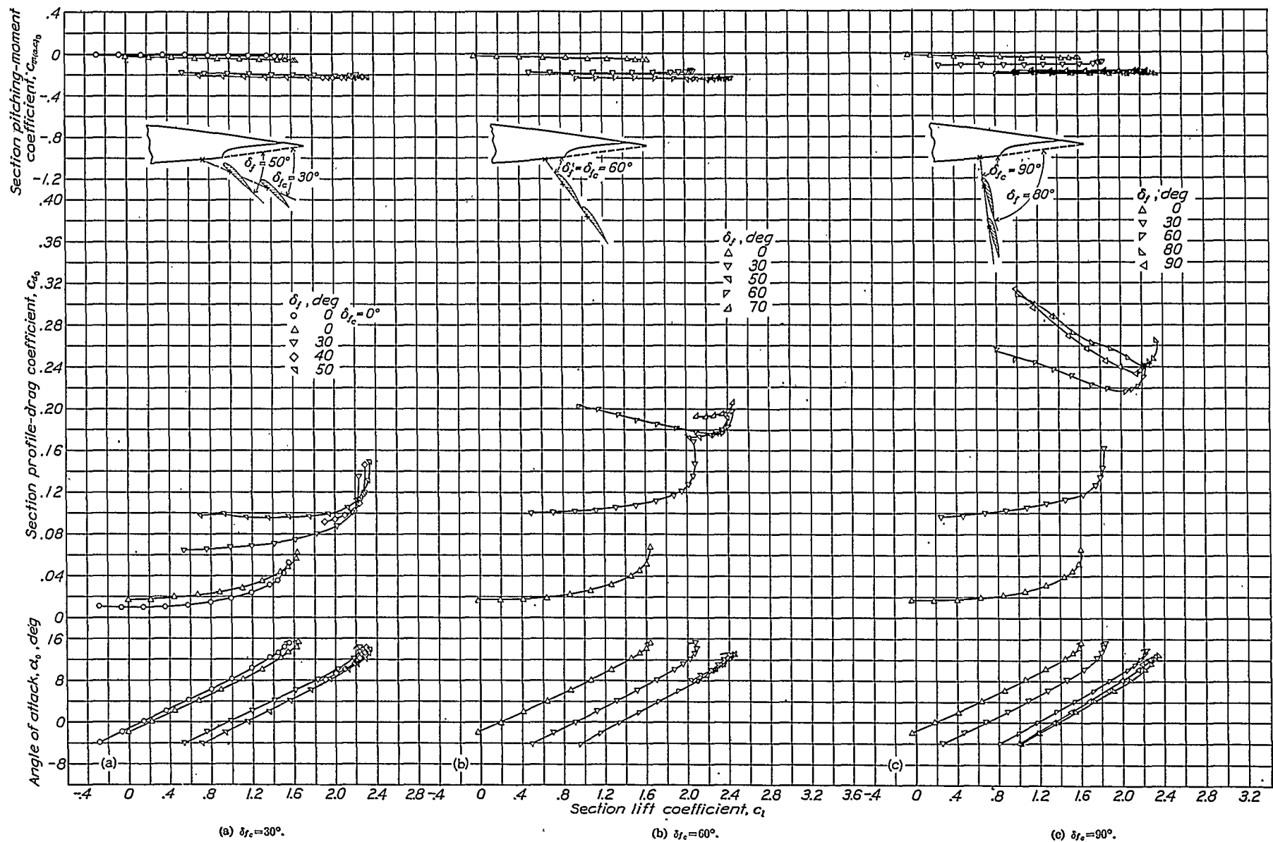
FIGURE 15.—Aerodynamic section characteristics of N. A. C. A. 23012 airfoil with a venetian-blind flap hinged at 0.75c axis; two 0.10c slats.
