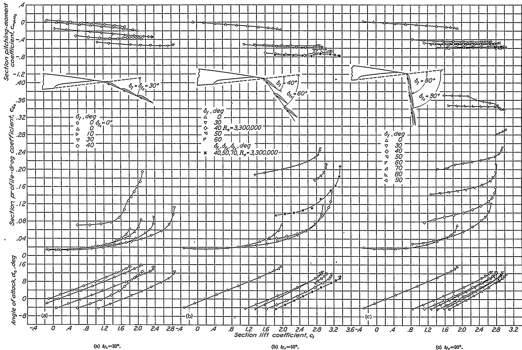
FIGURE 17.—Aerodynamic section characteristics of N. A. C. A. 23012 airfoil with a venetian-blind flap hinged at 0.995c axis; three 0.10c slats.
