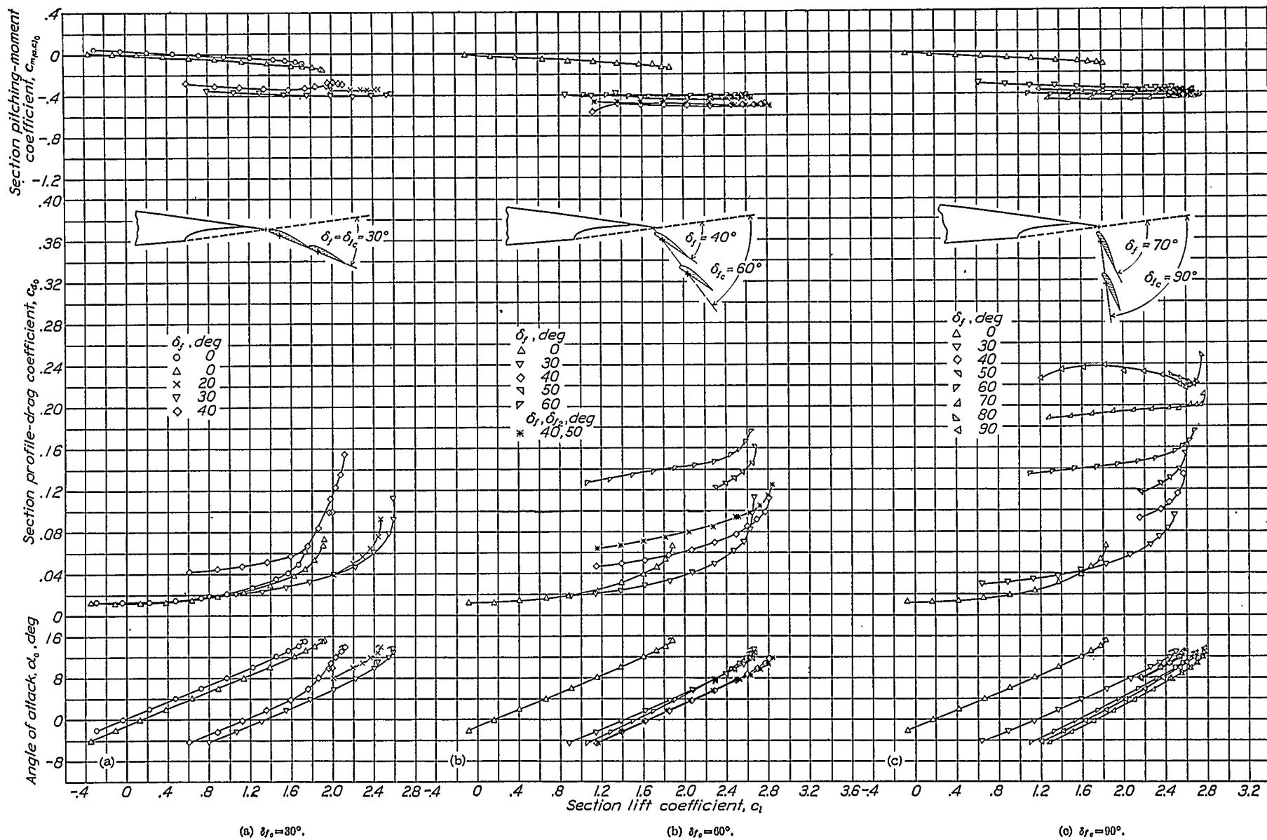
FIGURE 18.—Aerodynamic section characteristics of N. A. C. A. 23012 airfoil with a venetian-blind flap hinged at 0.095c axis; two 0.10c slats.
