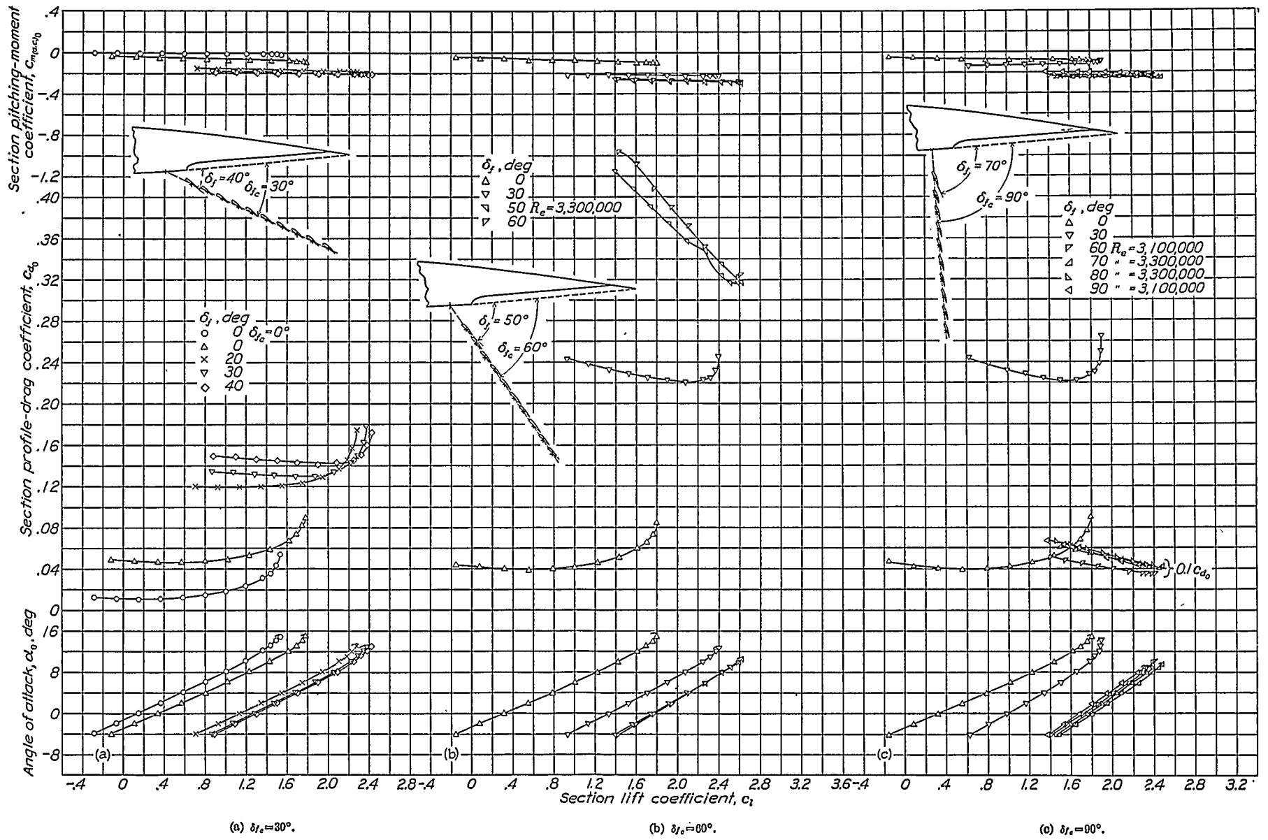
FIGURE 10.—Aerodynamic section characteristics of N. A. C. A. 23012 airfoil with a venetian-blind flap hinged at 0.55c axis; ton 0.04c slats.
