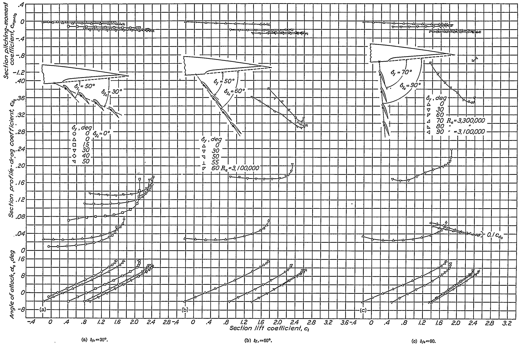
FIGURE 12.—Aerodynamic section characteristics of N. A. C. A. 23012 airfoil with a venetian-blind flap hinged at 0.55c axis; four 0.10c slats.
