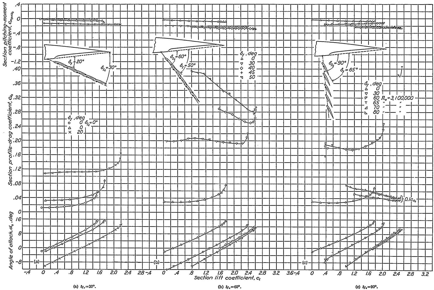
FIGURE 11.—Aerodynamic section characteristics of N. A. C. A. 23012 airfoil with a venetian-blind flap hinged at 0.55c axis; five 0.10c slats.
