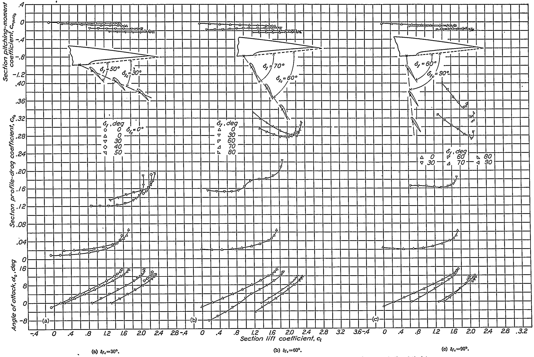
FIGURE 13.—Aerodynamic section characteristics of N. A. C. A. 23012 airfoil with a venetian-blind flap hinged at 0.55c axis; three 0.10c slats.
