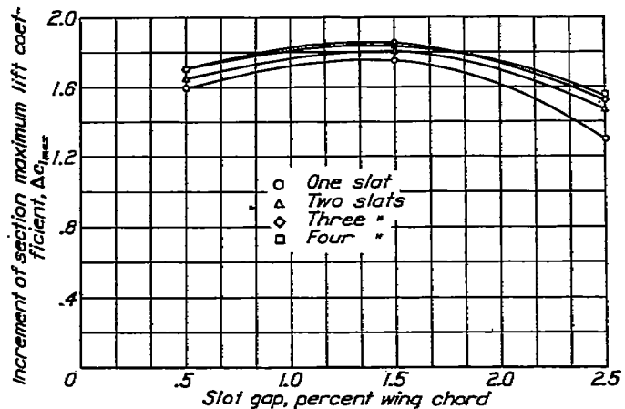
FIGURE 3.—Effect of slot gap on maximum lift of 0.20c venetian-blind flaps at optimum deflections
