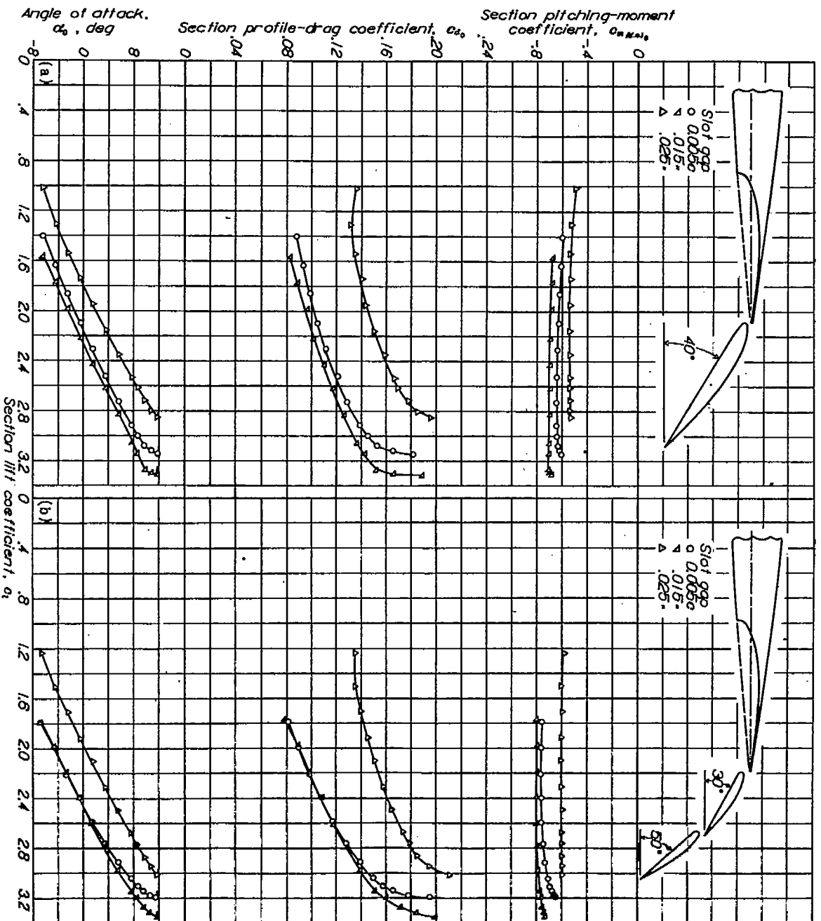
FIGURE 4.—Effect of slot gap on aerodynamic section characteristics of 0.3c venetian-blind flaps at optimum deflections.
