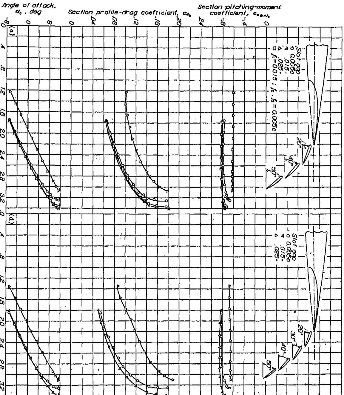
(c) Three slats; \delta_1 = 20^\circ ; \delta_2 = 40^\circ ; \delta_3 = 50^\circ .
