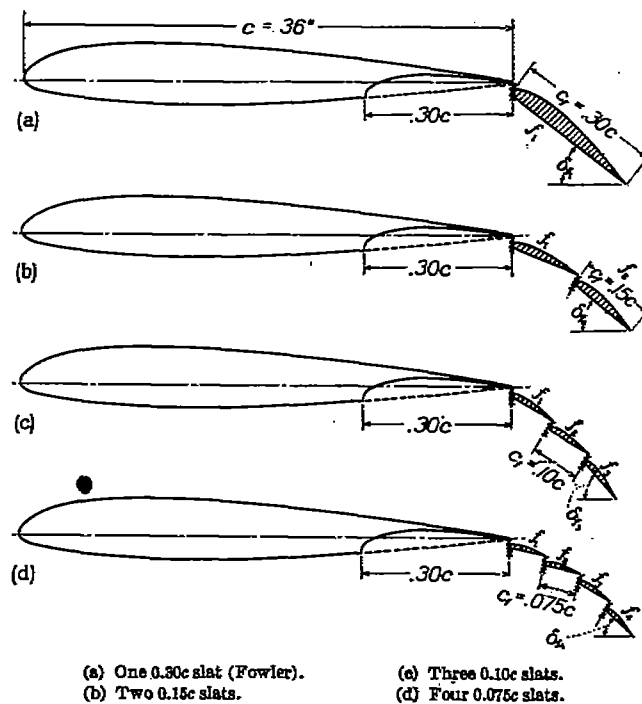
FIGURE 1.—Sections of NACA 23012 airfoil with several arrangements of 30c venetian-blind flaps. Test hinge axes of slats (x) at 0.005c, 0.015c, and 0.025c below trailing edge and perpendicular to chord line of preceding slat or airfoil.
