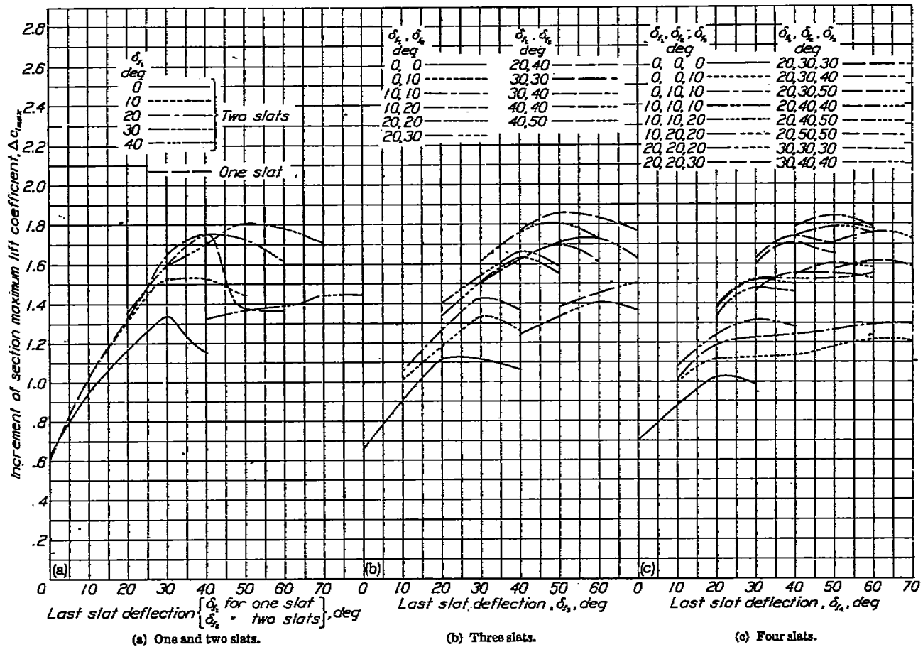
FIGURE 2.—Increments of maximum lift coefficients for various arrangements of 0.20c venetian-blind flaps with 0.015c gaps.
