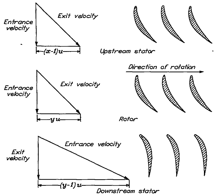
FIGURE 4.—Fan design for over-all pressure coefficient C_{p,r}=2 with rotor pressure coefficient C_{p,r}=-1 . Velocity vectors shown are relative to corresponding blading. Design values: x=0 ; y=-1 .
