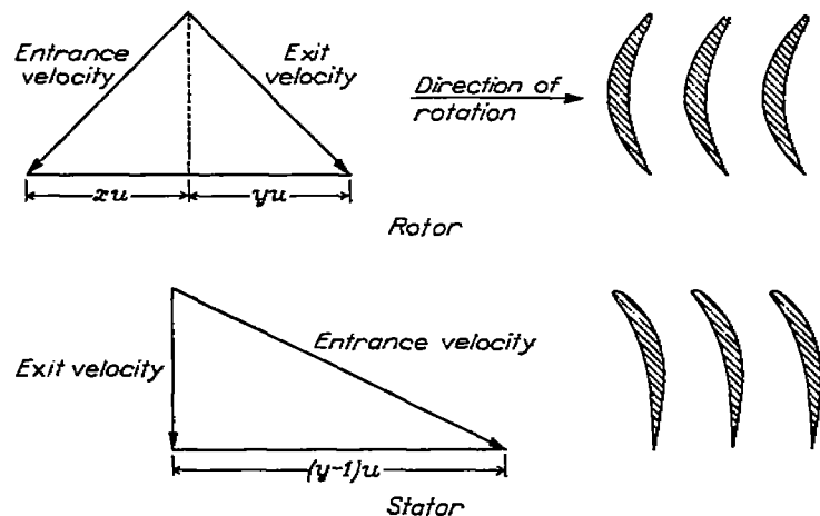
FIGURE 3.—Fan design for over-all pressure coefficient C_{p,r}=4 with rotor pressure coefficient C_{p,r}=0 . Velocity vectors shown are relative to corresponding blading. Design values: x=1 ; y=-1 .
