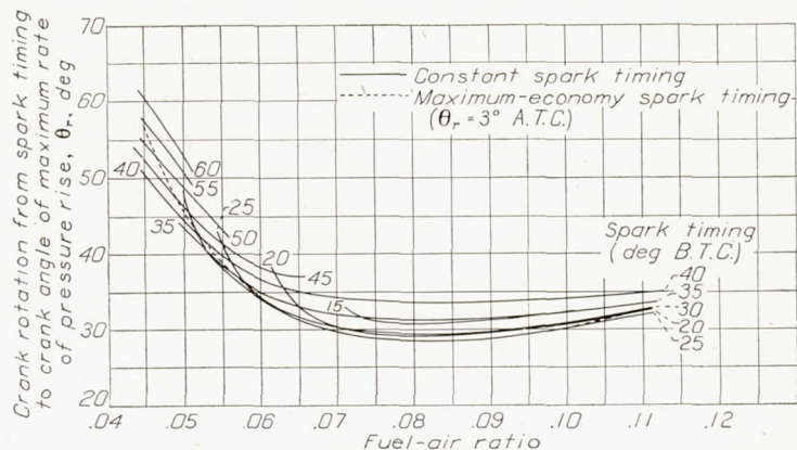
FIGURE 4.—Variation in crank rotation between spark timing and time of maximum rate of pressure rise with fuel-air ratio for constant spark timing and for maximum-economy spark timing. (Cross plot from fig. 2.)
