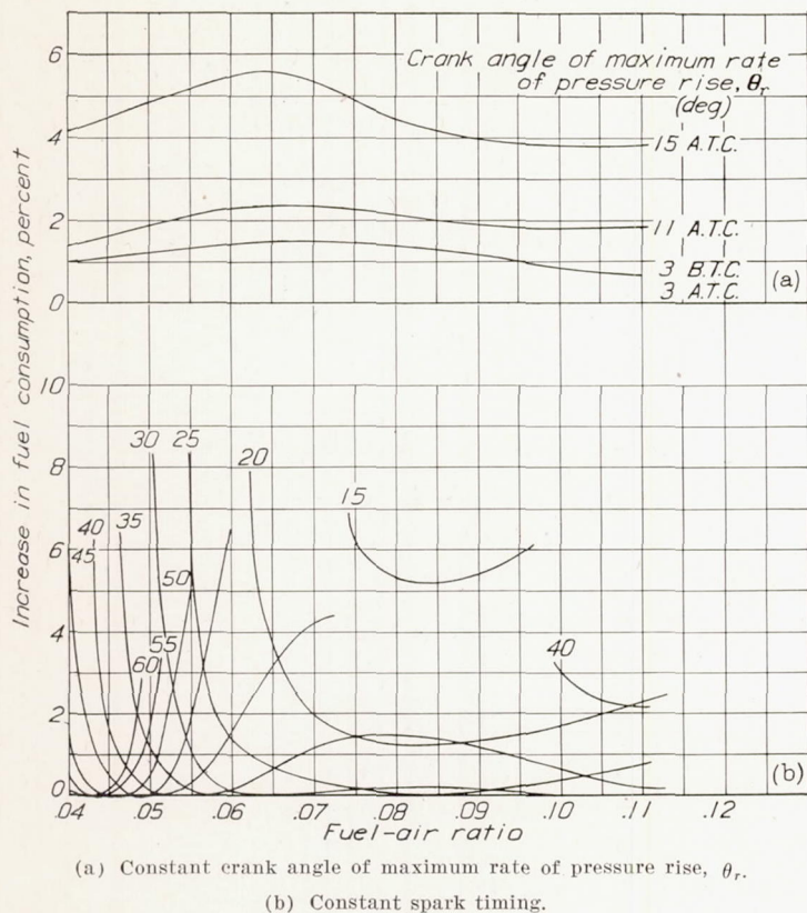
FIGURE 3.—Percentage increase in fuel consumption over that obtained with maximum-economy spark timing when fuel-air ratio is varied with various spark timings and crank angles of maximum rate of pressure rise \theta_r . Numerical values indicate spark timing, degrees B.T.C. (Cross plot from fig. 2.)
