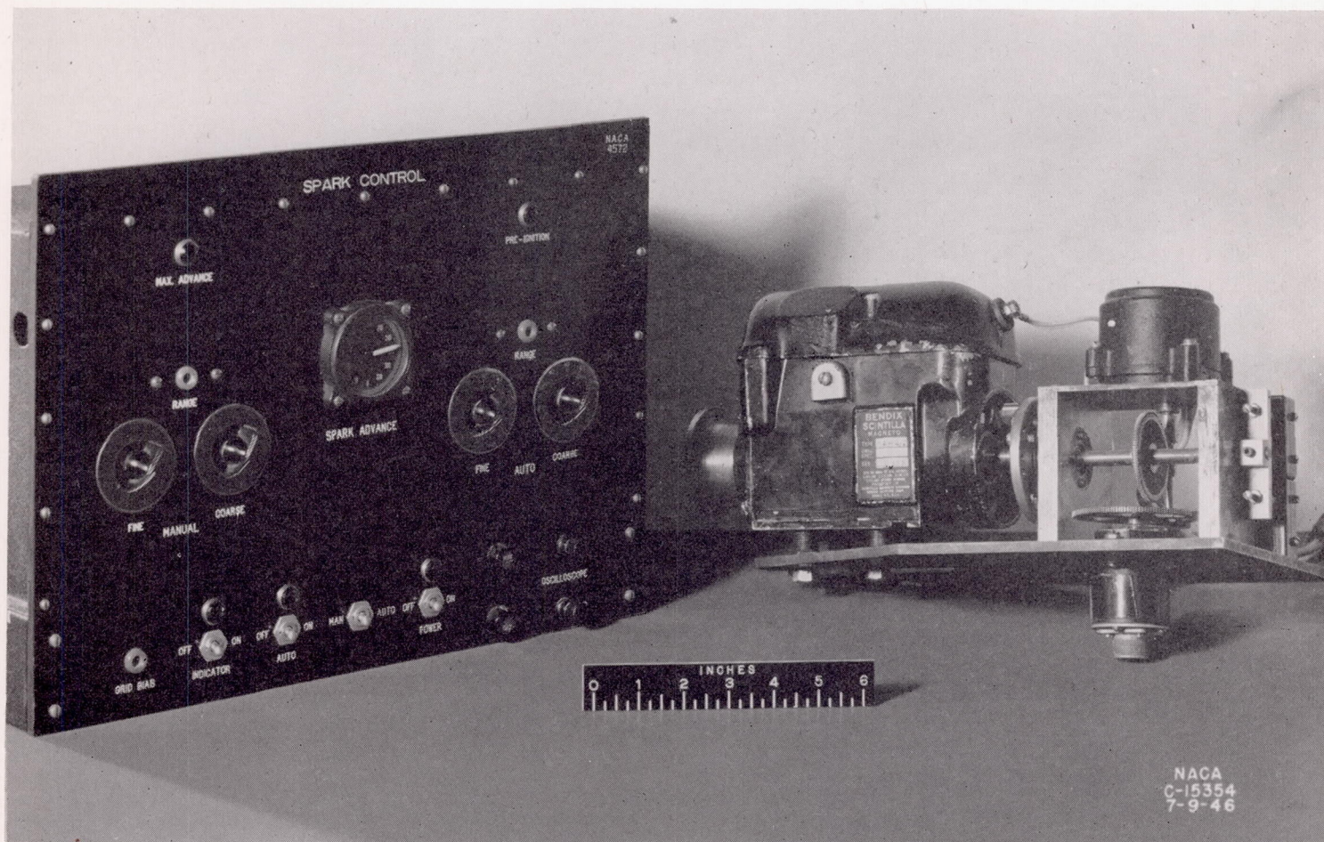
FIGURE 5.—Spark-timing-control instrument.
