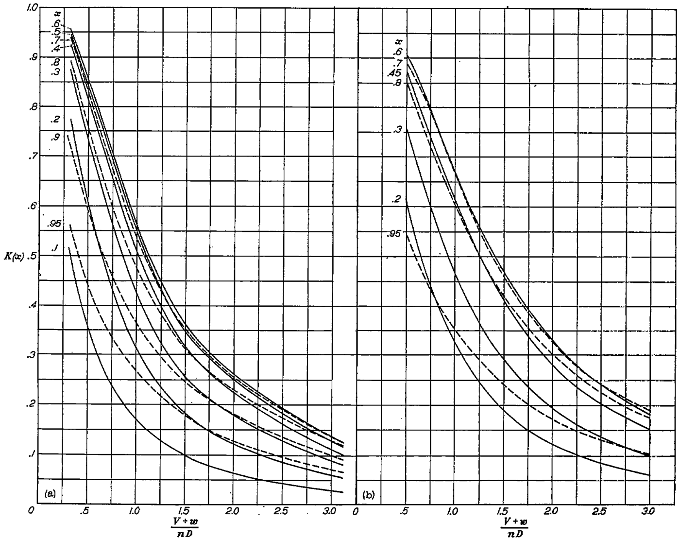
(a) Two-blade single-rotating propeller (reference 6).
