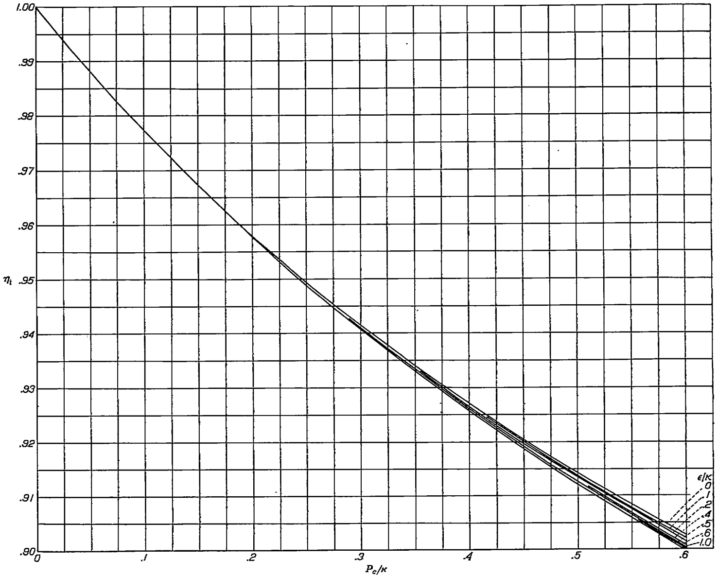
FIGURE 9.—Propeller efficiency against P_c/\kappa .
