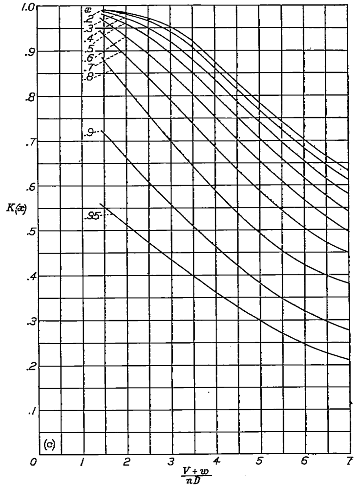
(c) Twelve-blade dual-rotating propeller.
