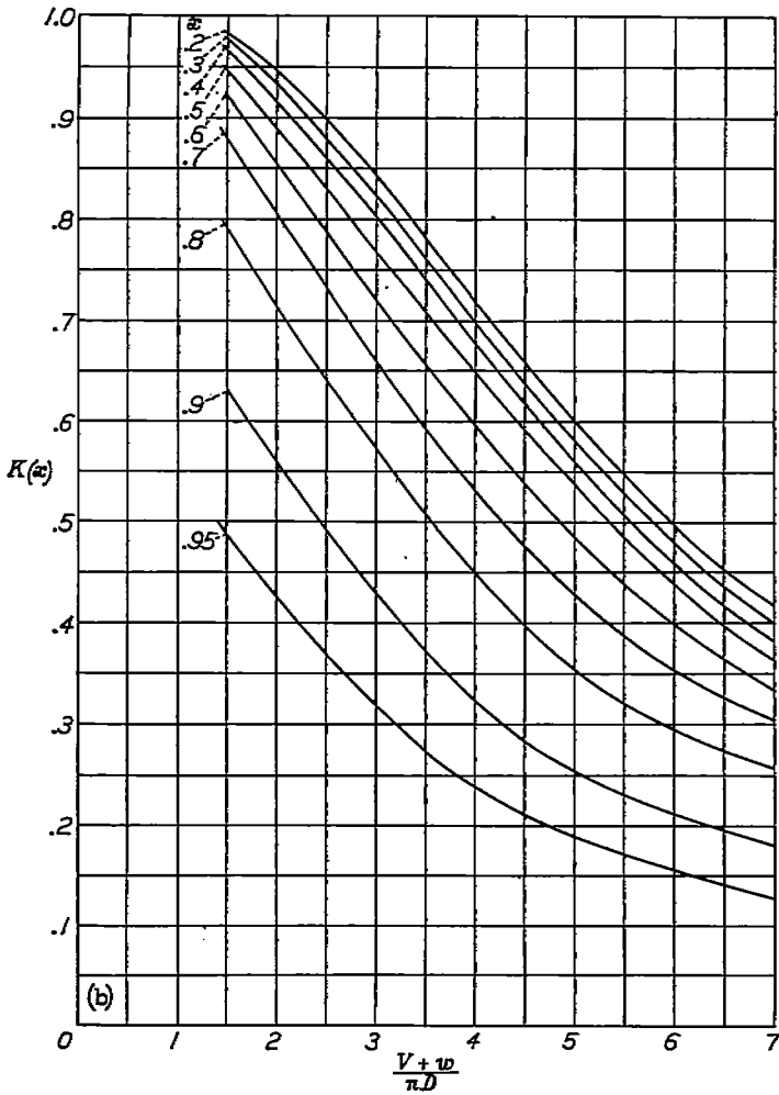
(b) Eight-blade dual-rotating propeller.
