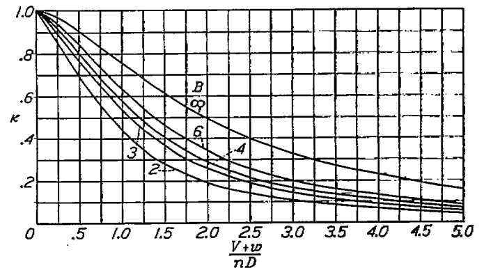
FIGURE 5.—Mass coefficient \kappa against \frac{V+w}{nD} for various numbers of blades for single-rotating propellers.
