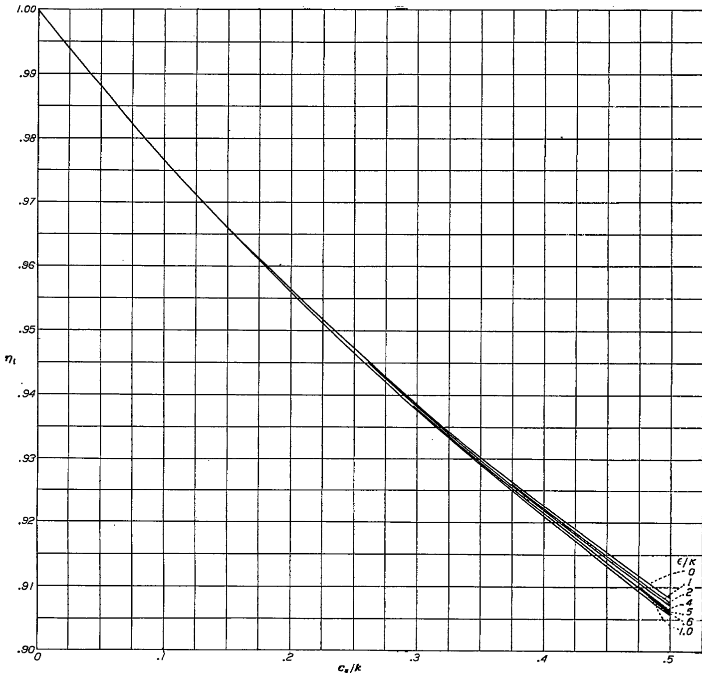
FIGURE 8.—Propeller efficiency against c_d/k (reference 4).
