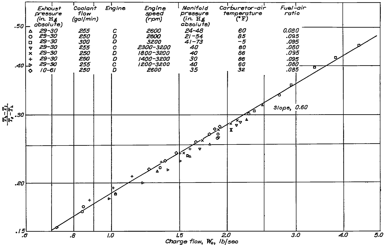
FIGURE 8.—Determination of exponent n on charge flow W_c for cylinder-head-temperature correlation from variation of \frac{T_h - T_i}{T_e - T_h} with W_c . Coolant, 30-70 ethylene glycol-water; average coolant temperature, 245° F.
