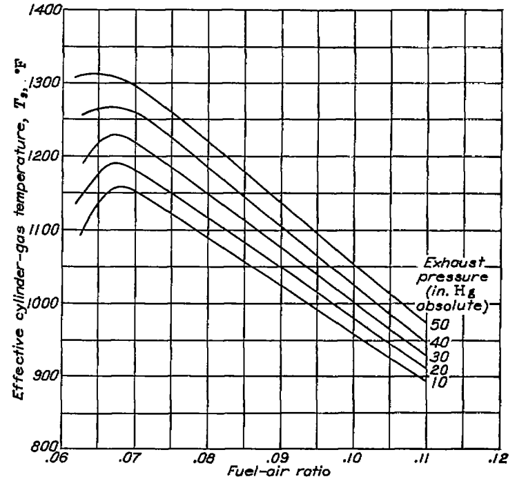
FIGURE 6.—Variation of effective cylinder-gas temperature with fuel-air ratio at various exhaust pressures for cylinder-head-temperature correlation (obtained from cross plot of fig. 5). Data corrected to dry inlet-manifold temperature of 80^\circ\text{F} ; standard ignition timing; engine D.
