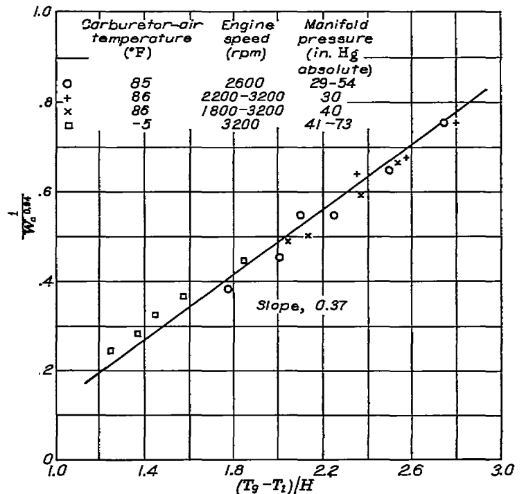
FIGURE 26.—Variation of 1/\dot{W}_c^{0.94} with (T_g - T_i)/H . Fuel-air ratio, 0.095; exhaust pressure, 29-30 inches mercury absolute; standard ignition timing.
