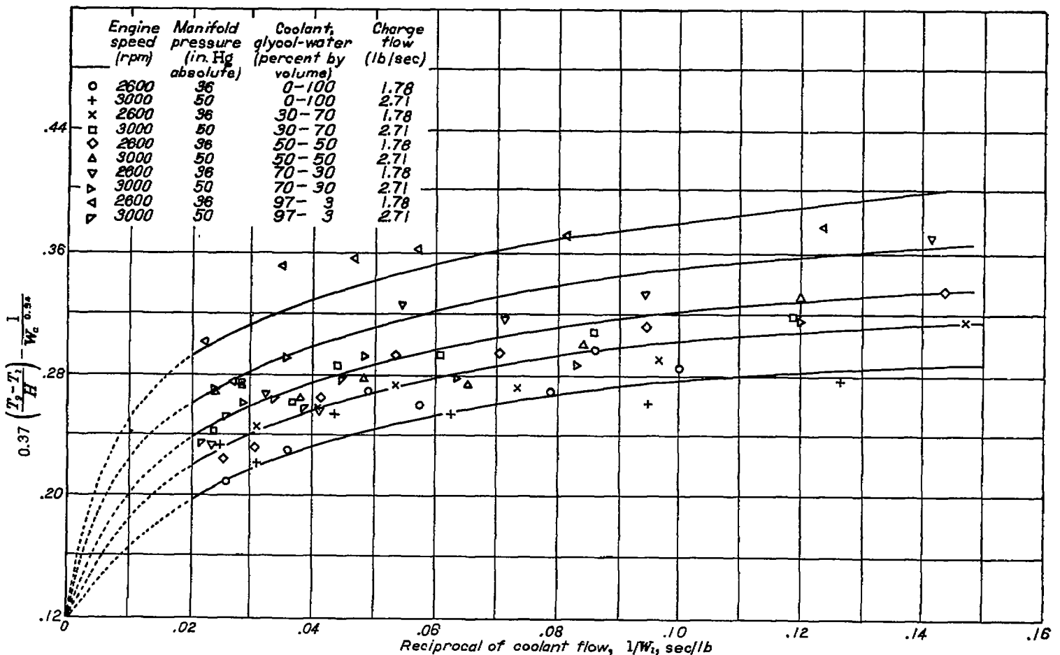
FIGURE 27.—Determination of factor Z for coolant-heat-rejection correlation from variation of 0.37 \left( \frac{T_s - T_i}{H} \right) - \frac{1}{W_c^{0.34}} with \frac{1}{W_i} . Average coolant temperature, 245° F.
