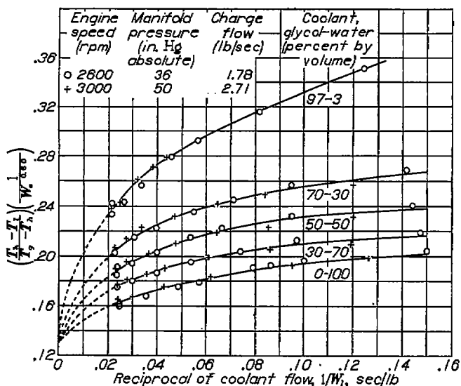
FIGURE 9.—Determination of factor Z from variation of \left(\frac{T_h - T_i}{T_g - T_h}\right) \left(\frac{1}{W_c^{0.60}}\right) with 1/W_i for cylinder-head-temperature correlation. Average coolant temperature, 245° F; engine D.
