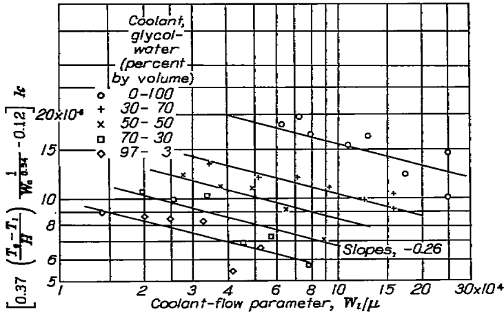
FIGURE 28.—Determination of exponent m on coolant-flow parameter W_i/\mu for coolant-heat-rejection correlation from variation of \left[ 0.37 \left( \frac{T_g - T_i}{H} \right) - \frac{1}{W_c^{0.94}} - 0.12 \right] k with \frac{W_i}{\mu} for various coolants. Average coolant temperature, 245° F.
