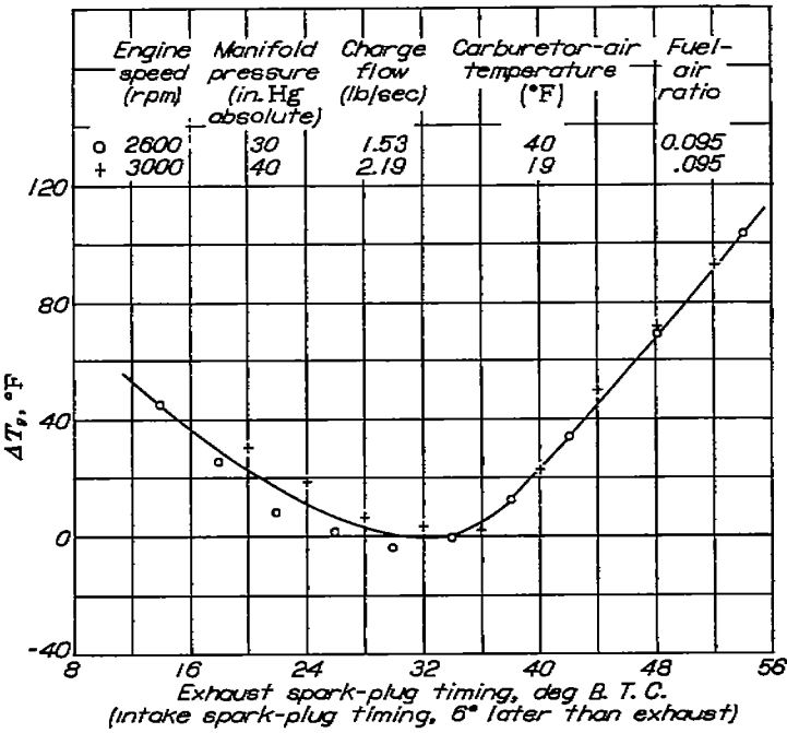
FIGURE 7.—Variation of change in effective cylinder-gas temperature with ignition timing for cylinder-head-temperature correlation. Engine D.
