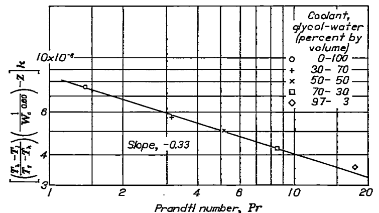
FIGURE 13.—Determination of exponent s on Prandtl number Pr for cylinder-head-temperature correlation from variation of \left[ \left( \frac{T_h - T_i}{T_s - T_h} \right) \left( \frac{1}{W_c^{0.60}} \right) - Z \right] k with Pr as obtained from cross plot of figure 12 at value for W_i/\mu of 55,000. Average coolant temperature, 245° F; engine D.
