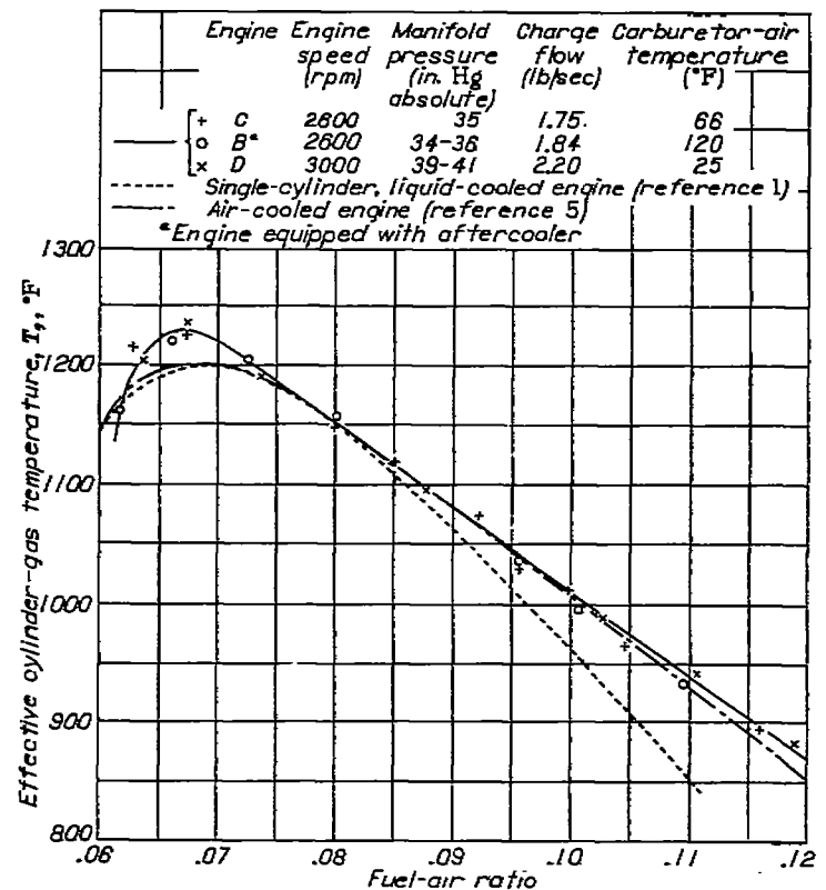
FIGURE 3.—Variation of effective cylinder-gas temperature with fuel-air ratio for cylinder-head-temperature correlation. Data corrected to dry inlet-manifold temperature of 80° F; exhaust pressure, 29-30 inches mercury absolute; standard ignition timing.
