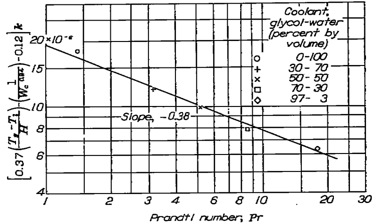
FIGURE 29.—Determination of exponent s on Prandtl number Pr for coolant-heat-rejection correlation from variation of \left[ 0.37 \left( \frac{T_g - T_i}{H} \right) - \frac{1}{W_c^{0.94}} - 0.12 \right] k with Pr as obtained from cross plot of figure 28 at value of \frac{W_i}{\mu} of 55,000. Average coolant temperature, 245° F.
