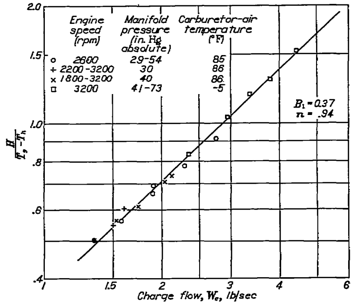
FIGURE 25.—Determination of exponent n and constant B_1 or coolant-heat-rejection correlation from variation of H/(T_g - T_i) with \dot{W}_c . Fuel-air ratio, 0.095; exhaust pressure, 29-30 inches mercury absolute; standard ignition timing.
