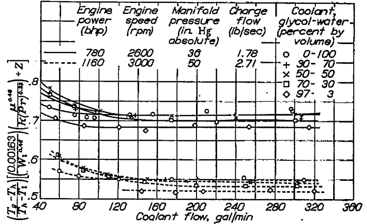
FIGURE 17.—Variation of \left(\frac{T_c - T_h}{T_h - T_i}\right) \left[ \left(\frac{0.00163}{W_i^{0.48}}\right) \left(\frac{\mu^{0.48}}{k(P_r)^{0.33}}\right) + Z \right] with coolant flow as indication of boiling. Average coolant temperature, 243^\circ F; engine D.
