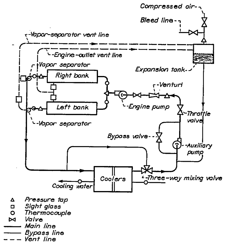
FIGURE 2.—Schematic diagram of engine coolant system.
