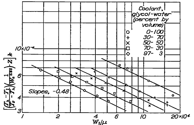
FIGURE 12.—Determination of exponent m on coolant-flow parameter W_i/\mu for cylinder-head-temperature correlation from variation of \left[ \left( \frac{T_h - T_i}{T_s - T_h} \right) \left( \frac{1}{W_c^{0.60}} \right) - Z \right] k with W_i/\mu for various coolants. Average coolant temperature, 245° F; engine D.
