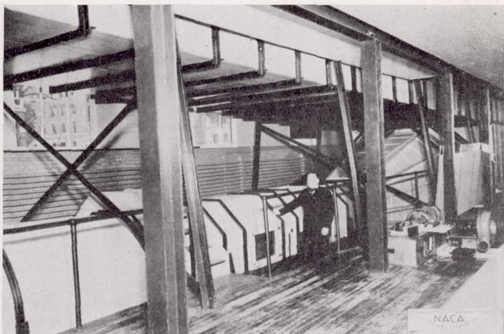
FIGURE 4.—The 4 1/2-foot wind tunnel of the National Bureau of Standards.
