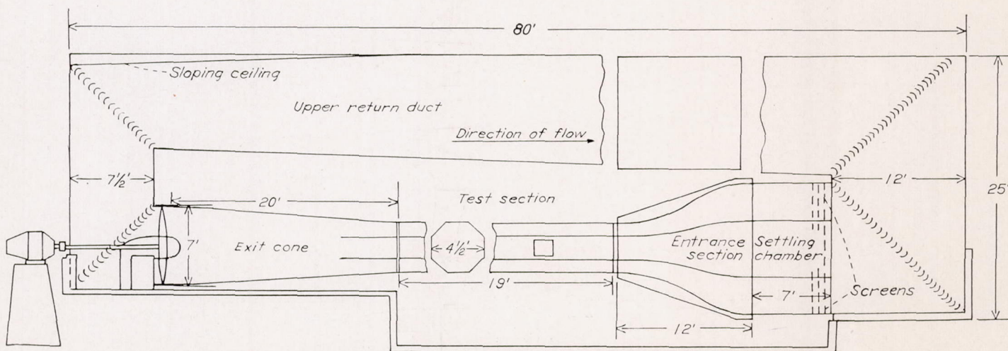
FIGURE 5.—Longitudinal cross section of the 4 1/2-foot wind tunnel of the National Bureau of Standards.
