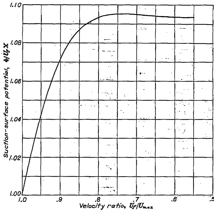
FIGURE 3.—Relation between suction-surface potential and velocity ratio for laminar diffusion with D_T = -0.0038 .
