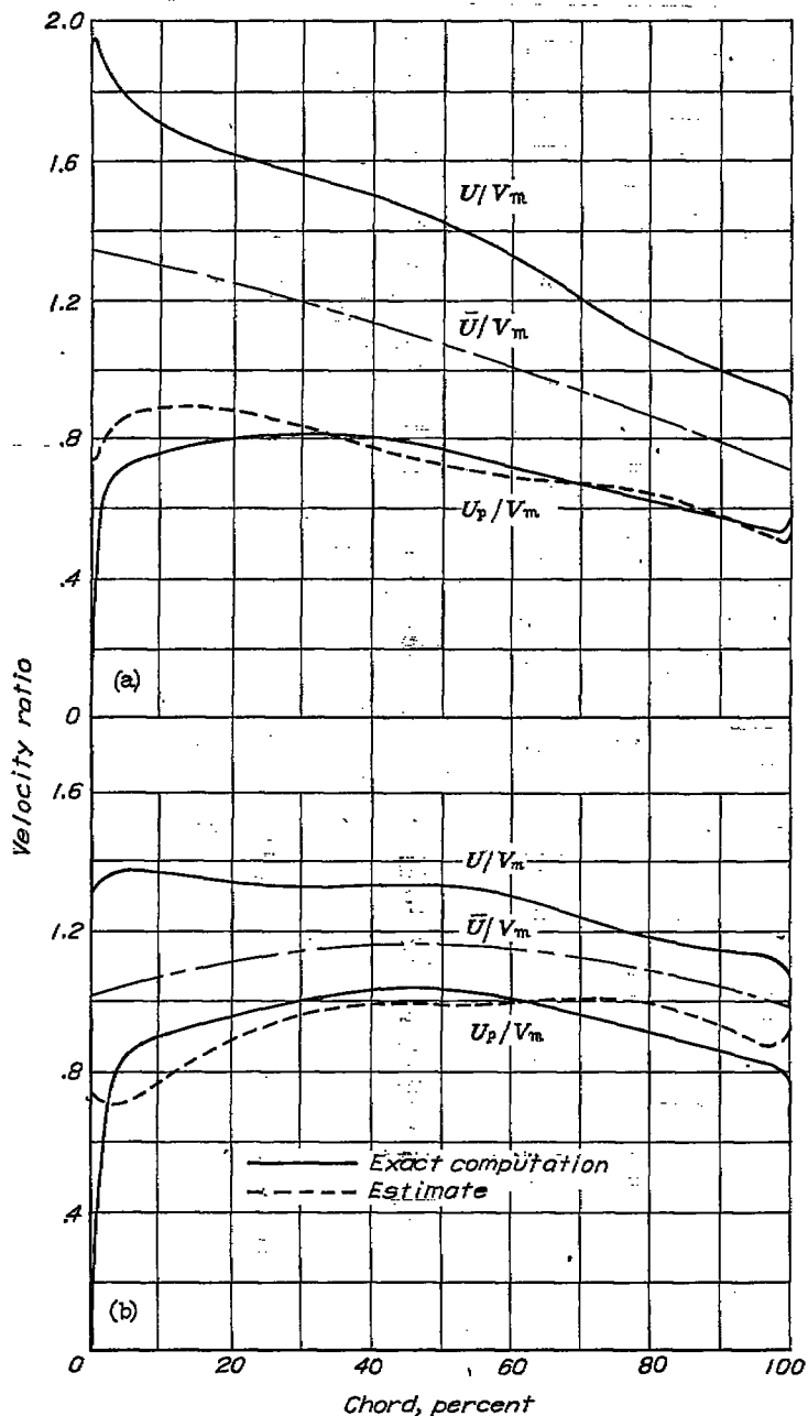
(a) NACA 65-(12)10; c/s=1.00 ; \alpha_1=63.0^\circ ; \Gamma/V_m c=0.735 ; \alpha_m=63.4^\circ ; estimated c/s=1.06 . (b) NACA 65-(8)10; c/s=1.00 ; \alpha_1=3.7^\circ ; \Gamma/V_m c=0.365 ; \alpha_m=-6.8^\circ ; estimated c/s=0.96 .
