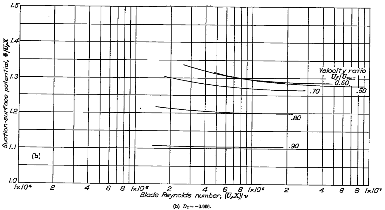
FIGURE 6.—Variation of suction-surface potential with blade Reynolds number. R_D=250 .
