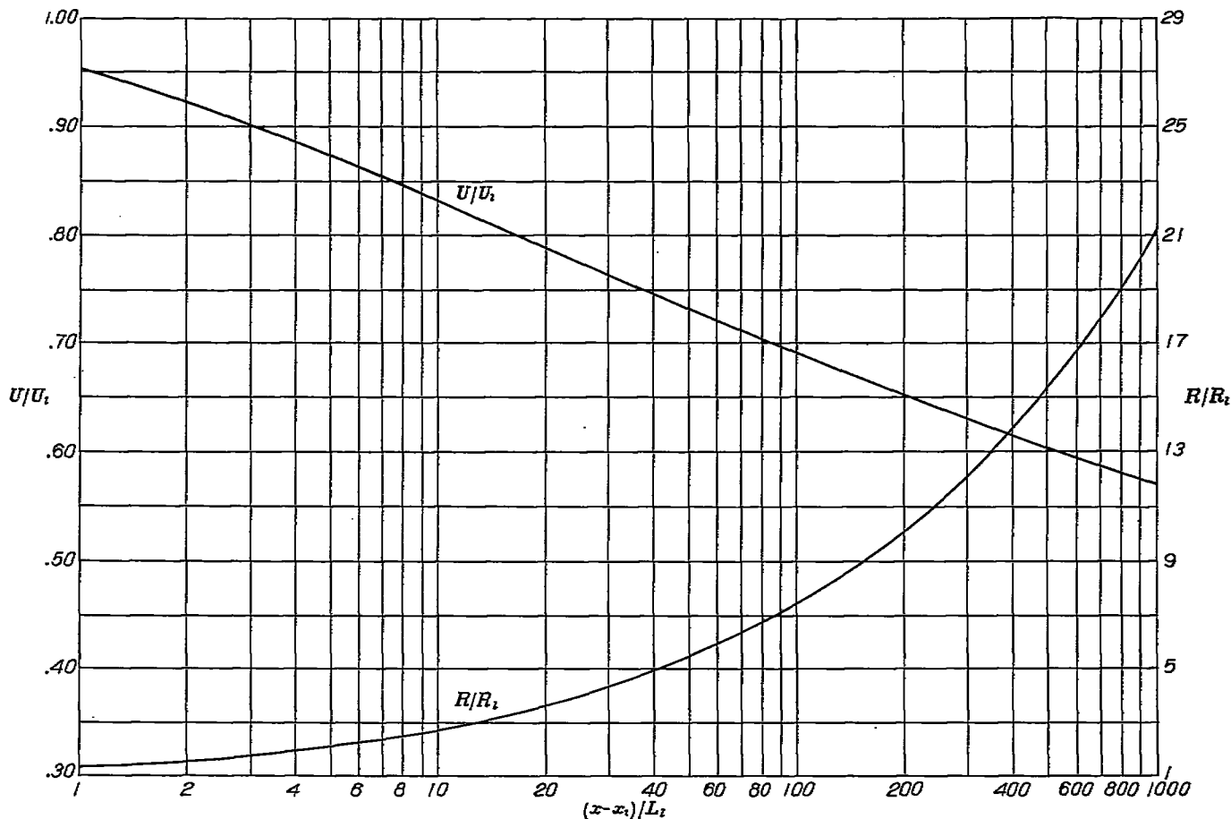
FIGURE 2.—Development of velocity and laminar boundary layer with constant diffusion coefficient. D_L = -0.06618 ; H = 3.214 .
