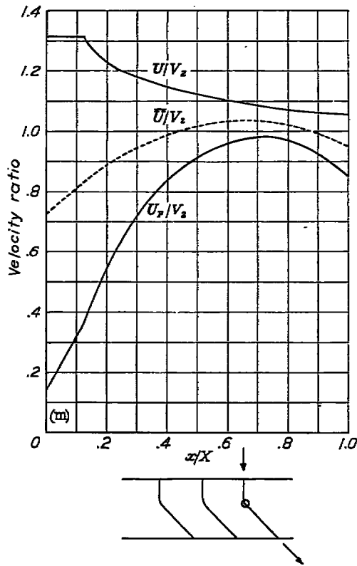
(m) Case (m) D_L = -0.06618 ; RN < 70,000 ; \alpha_1 = 0^\circ ; \alpha_2 = -45^\circ ; t_m/X = 0.09 ; X/s = 1.7 .
