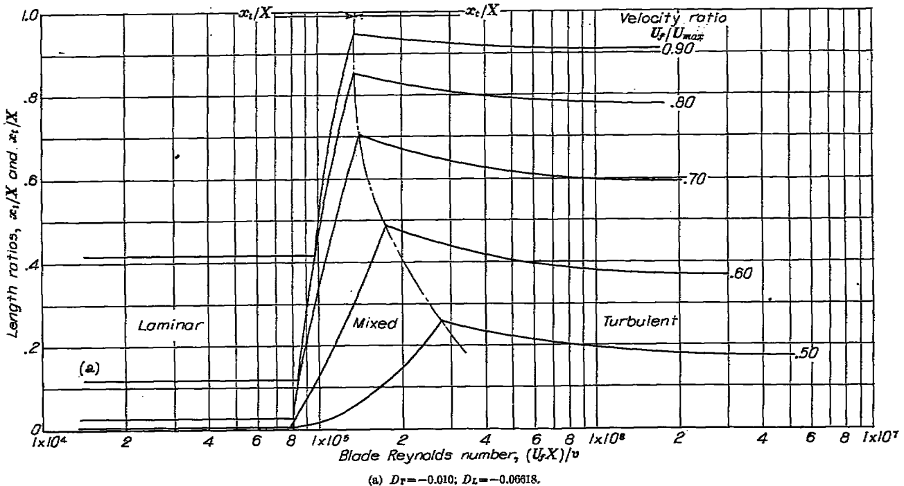
(a) D_T = -0.010 ; D_L = -0.06618 . FIGURE 5.—Variation of length ratios x_i/X and x_t/X with blade Reynolds number. R_{tr} = 250 .
