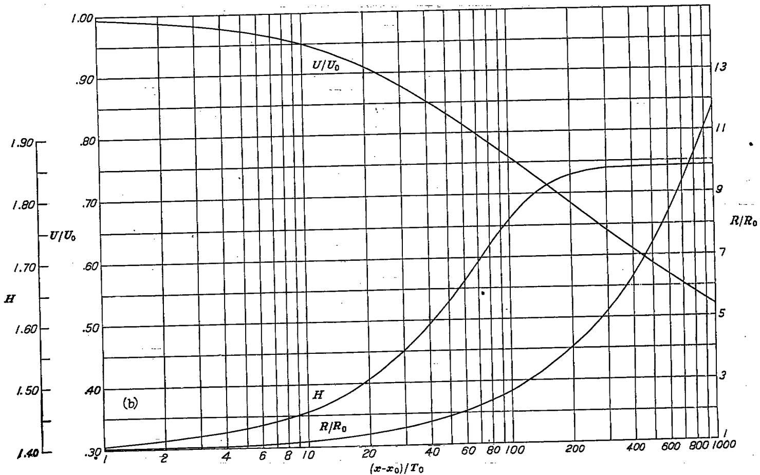
FIGURE 4.—Turbulent boundary-layer growth.
