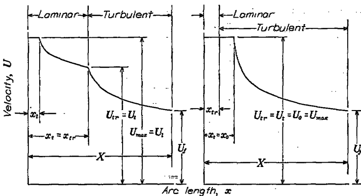
FIGURE 1.—Suction-surface velocities and lengths.
