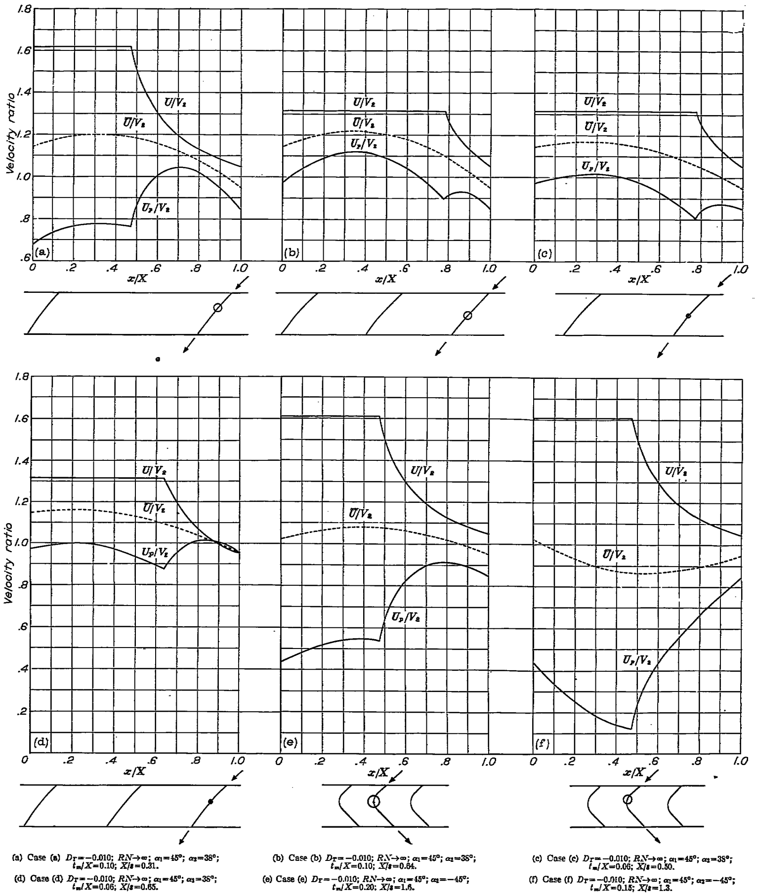
FIGURE 10.—Examples of velocity distributions.
