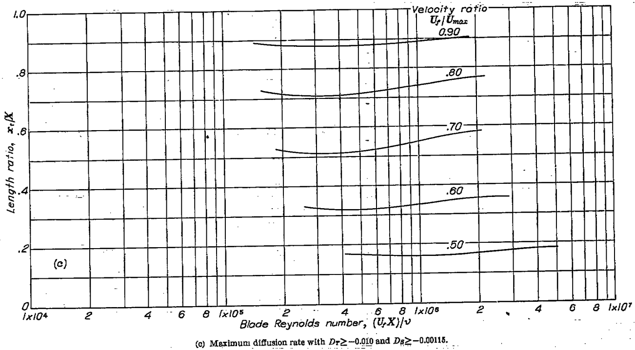
FIGURE 5.—Concluded. Variation of length ratios x_i/X and x_t/X with blade Reynolds number. R_n=250 .
