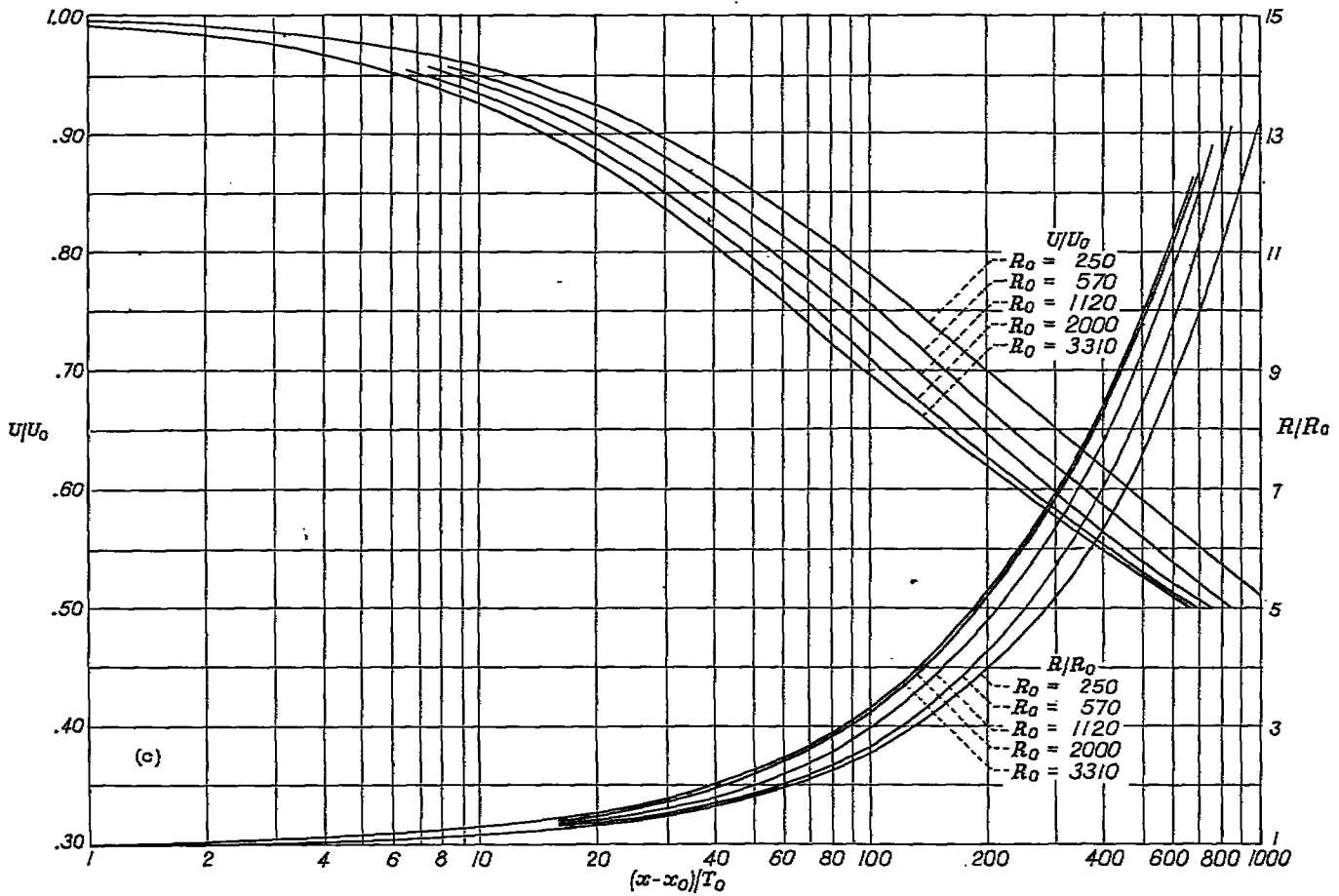
(c) Maximum diffusion rate D_T \geq -0.01 and D_S \geq -0.00115 . FIGURE 4.—Concluded. Turbulent boundary-layer growth.
