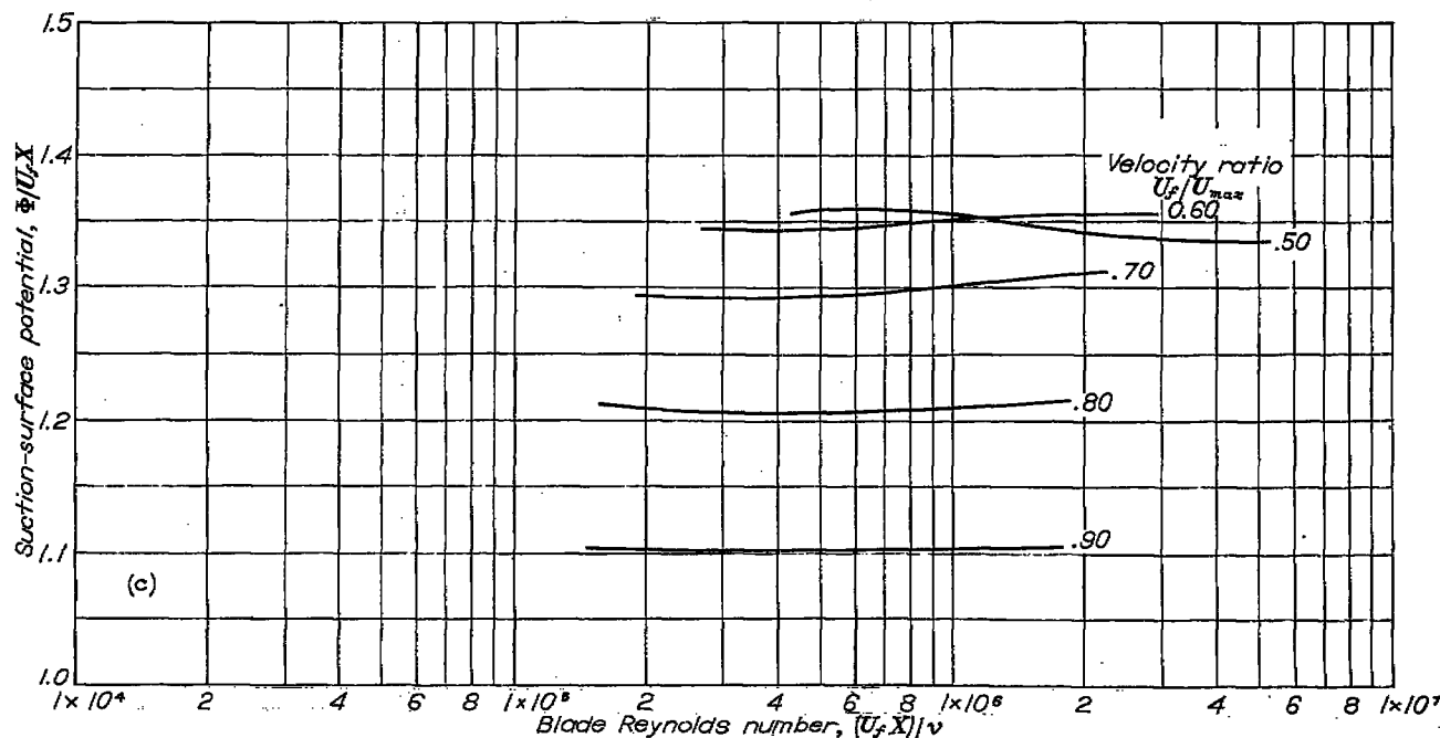
(c) Maximum diffusion rate with D_T \geq -0.010 and D_S \geq -0.00115 .
