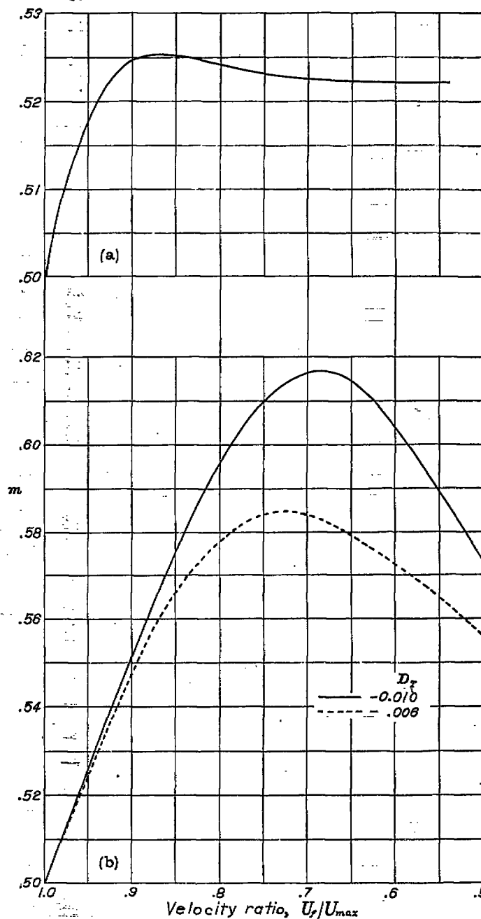
(a) Laminar diffusion. (b) Blade Reynolds number approaching infinity.
