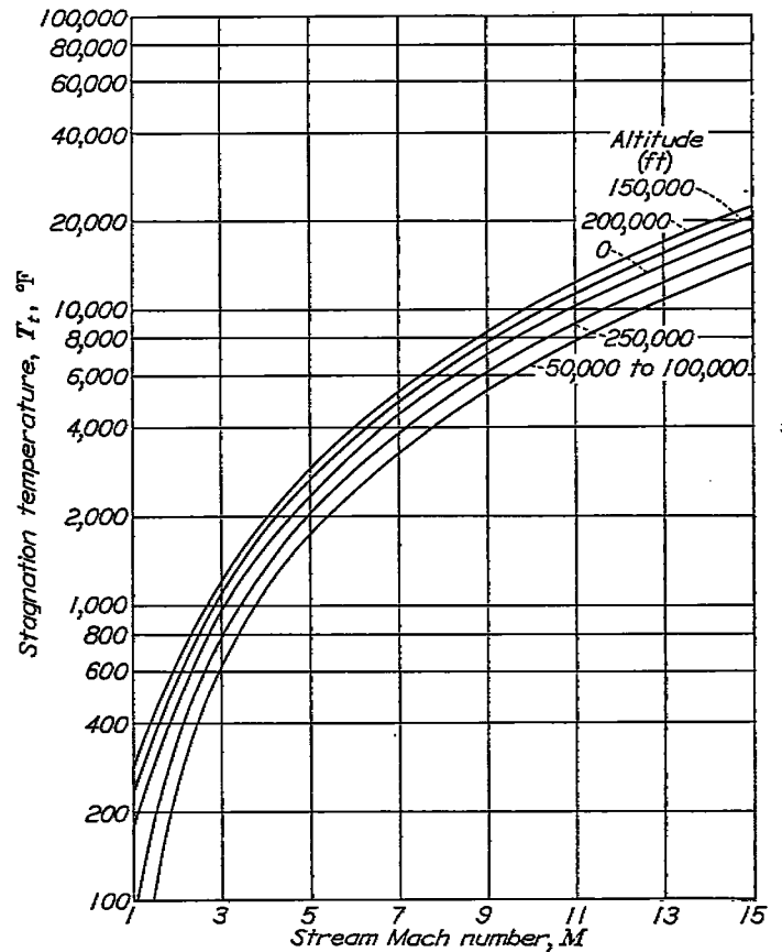
FIGURE 2.—Effect of Mach number on stagnation temperature.
