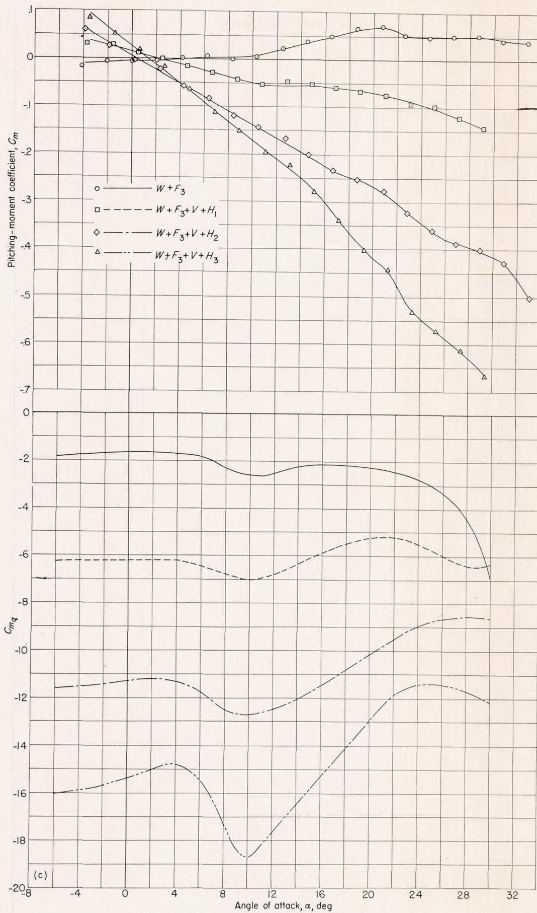
(c) Long fuselage F_3 .
