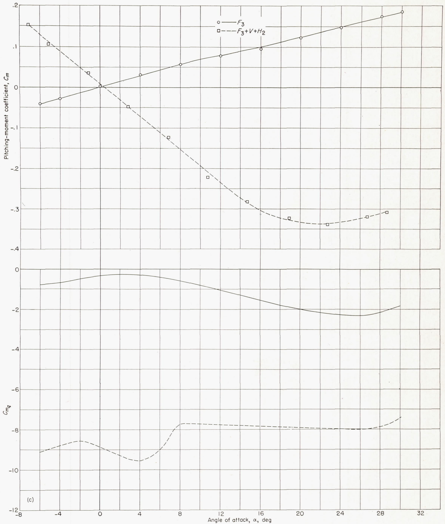
(c) Long fuselage F_3 .
