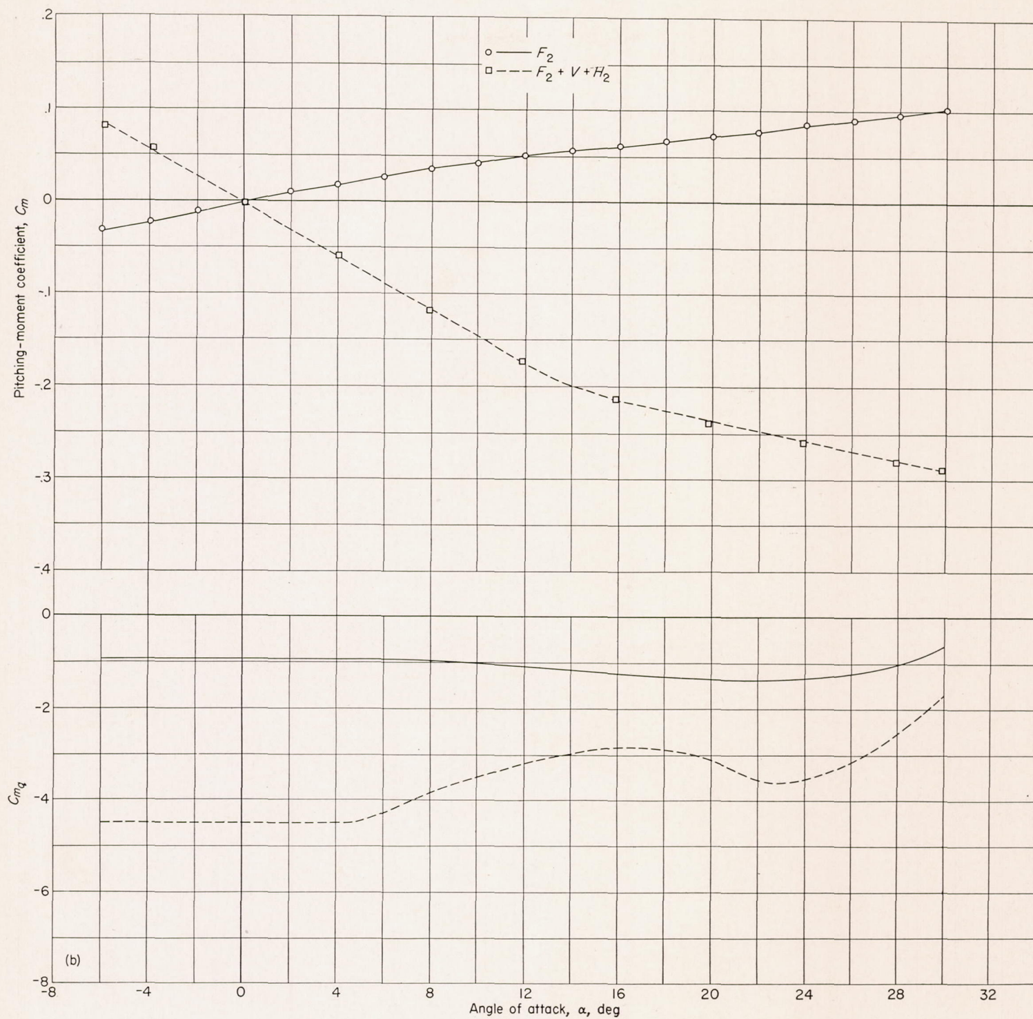
(b) Medium fuselage F_2 .
