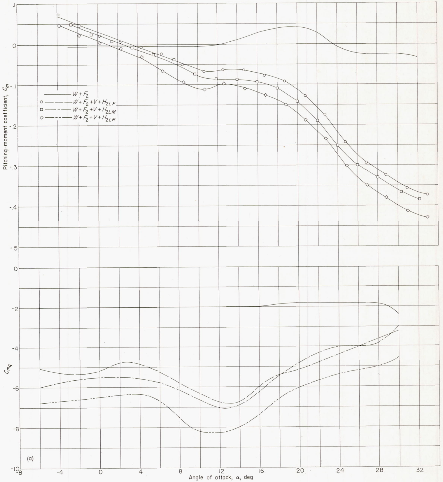
(a) Horizontal tail in the low position.
