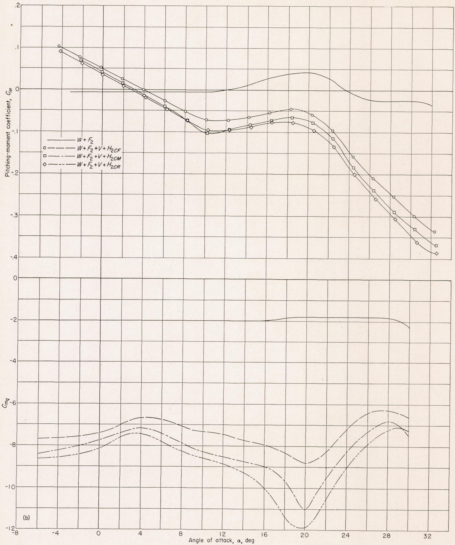
(b) Horizontal tail in the center position.
