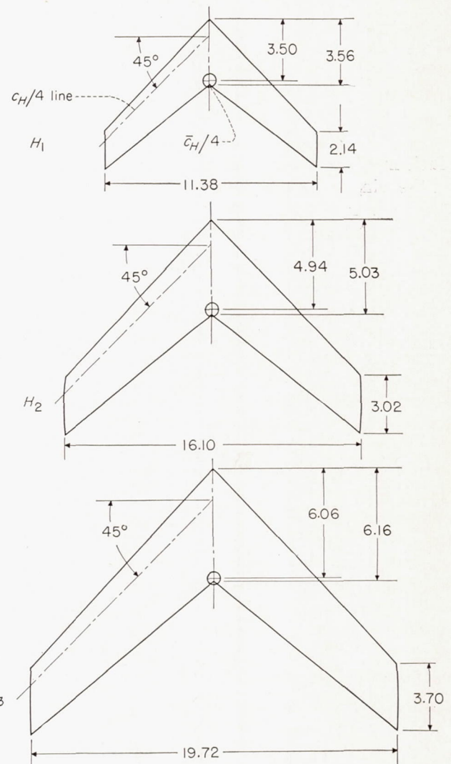
FIGURE 4.—Dimensions of the horizontal tails tested. All dimensions are in inches.
