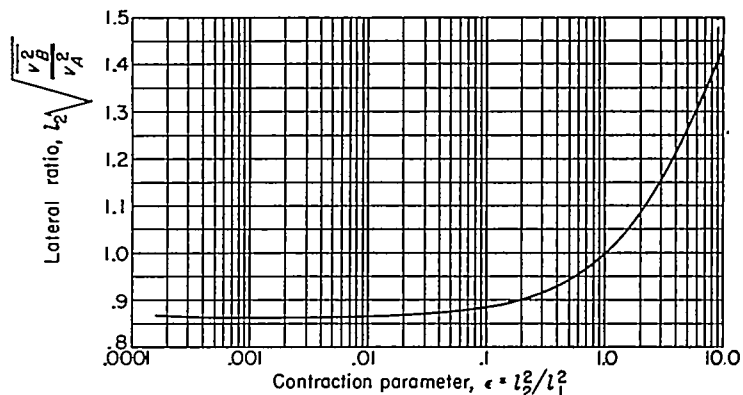
FIGURE 6.—Variation of relative root-mean-square lateral velocity fluctuation with both speed ratio l_1 and area ratio l_2^2 for axisymmetric contraction and isotropic turbulence at l_1=1 .
