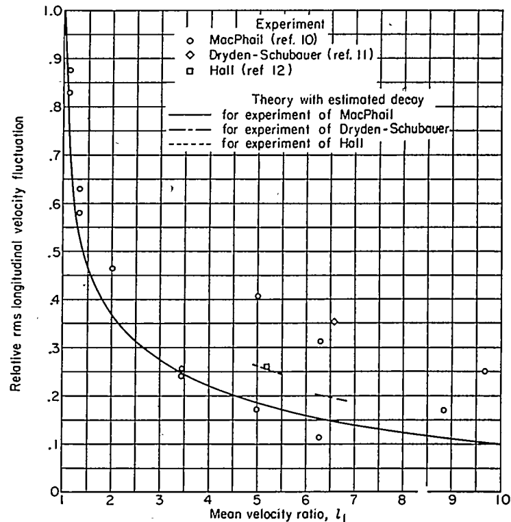
FIGURE 7.—Comparison of predicted axisymmetric contraction effect with experiment for longitudinal component of turbulence, with decay allowed for in first approximation. Initial isotropic turbulence assumed.
