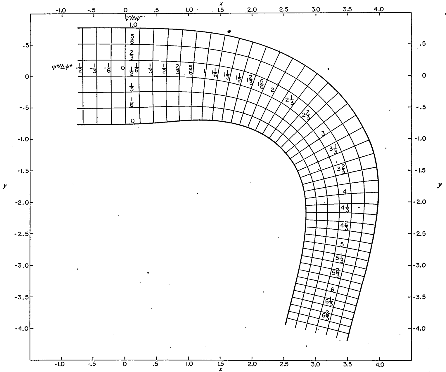
FIGURE 18.—Streamlines and velocity-potential lines in physical xy -plane for example IV. Linearized compressible flow; prescribed velocity as function of arc length along channel walls same as for example III (fig. 2) and with q_2 equal to 0.80176.
