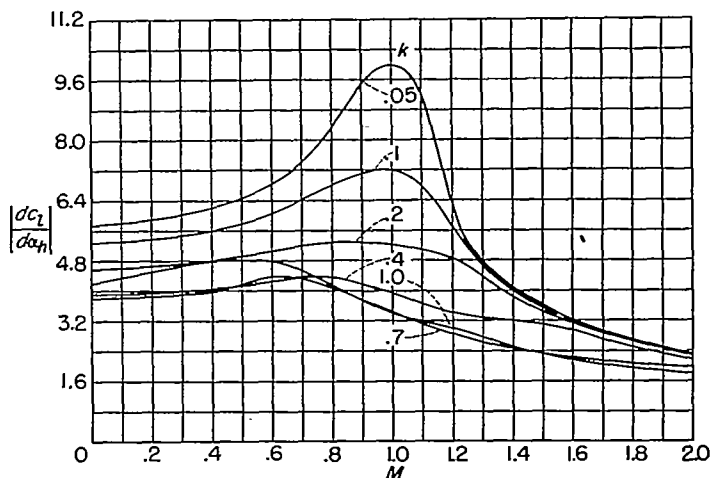
FIGURE 4.—Magnitude of lift-curve slope associated with vertical translation of wing against Mach number for several values of reduced frequency. \left| \frac{dc_1}{d\alpha} \right| = 4k\sqrt{L_1'^2 + L_2'^2} .
