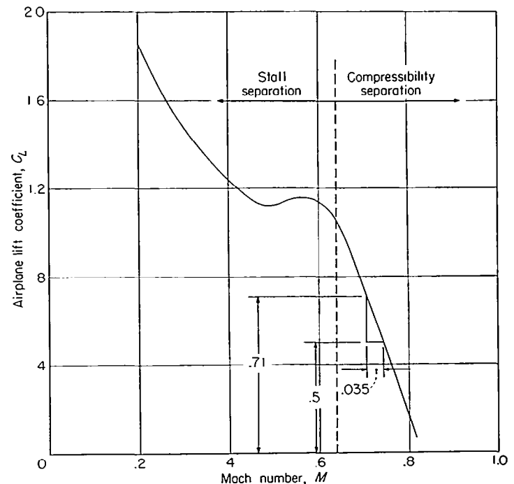
FIGURE 1.—Typical buffeting boundary for high-speed fighter airplane 1.
