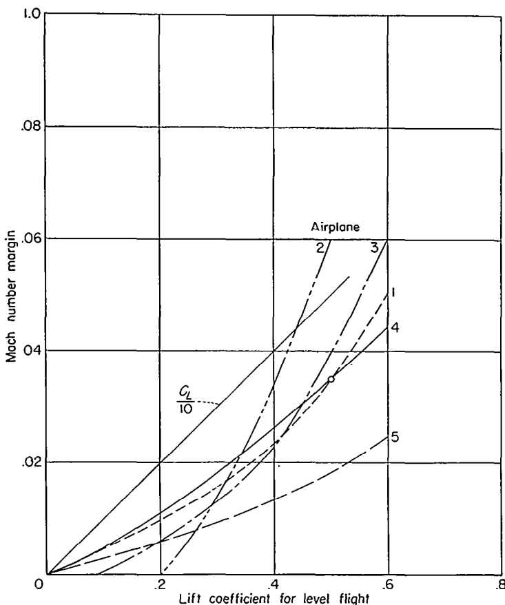
FIGURE 2.—Mach number margin required to execute 45° bank without crossing the buffet boundary.
