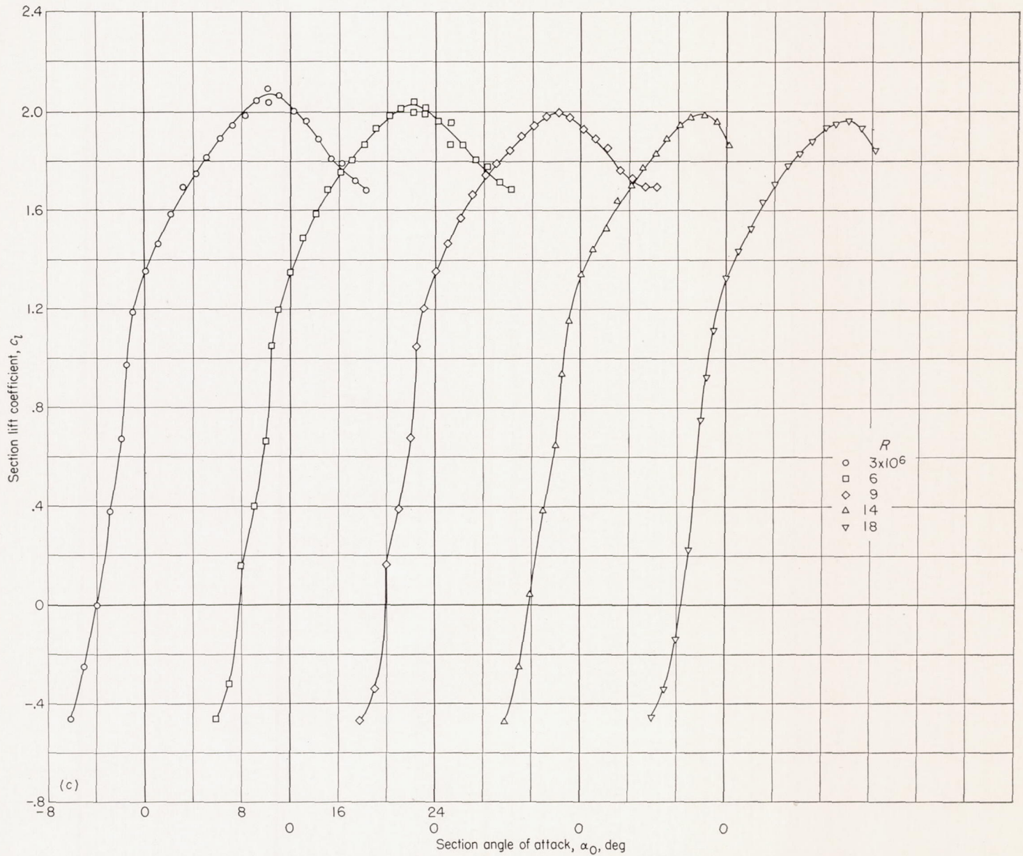
(c) 10-percent-thick airfoil. \delta_N=36^\circ , \delta_F=60^\circ .
