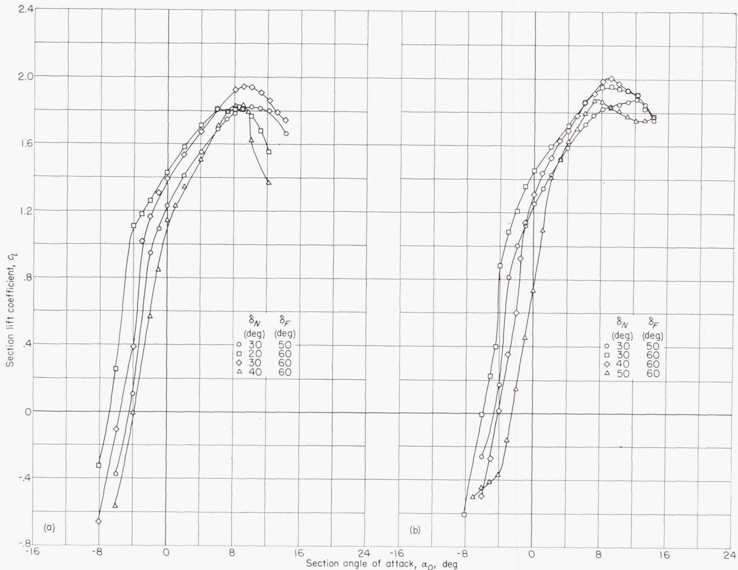
(a) 6-percent-thick airfoil. R=6 \times 10^6 .
