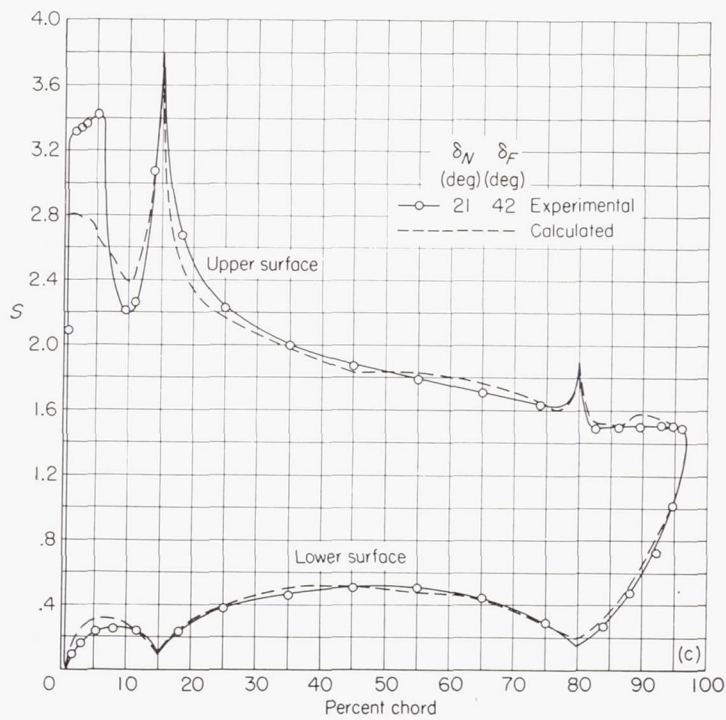
(c) \alpha_0 = 6.1^\circ . FIGURE 30.—Concluded.
