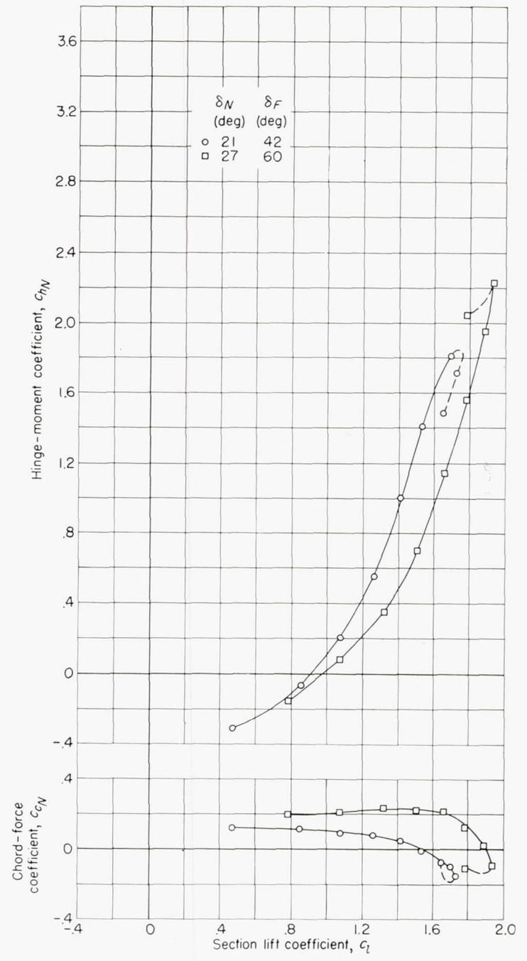
(a) Plain leading-edge flap.
