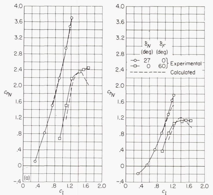
(a) 0.15-chord plain leading-edge flap.
