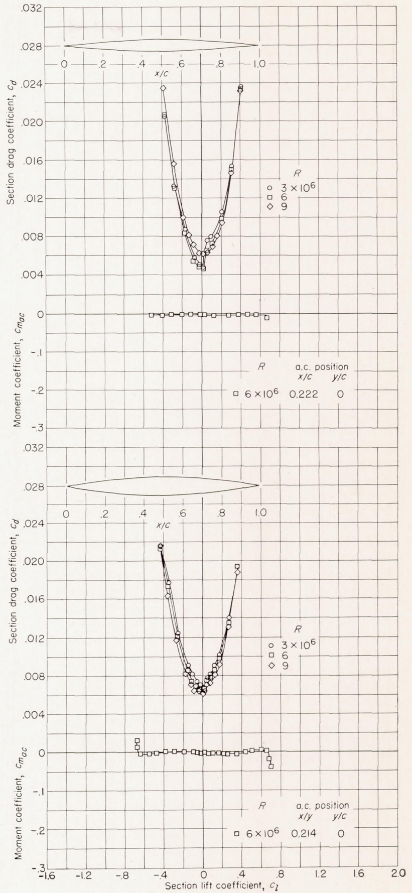
(a) 6-percent-thick airfoil. (b) 10-percent-thick airfoil.
