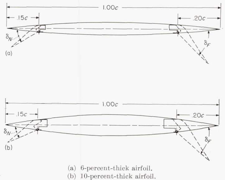
(a) 6-percent-thick airfoil. (b) 10-percent-thick airfoil. FIGURE 1.—Symmetrical circular-arc airfoils with plain leading-edge flaps and plain trailing-edge flaps.
