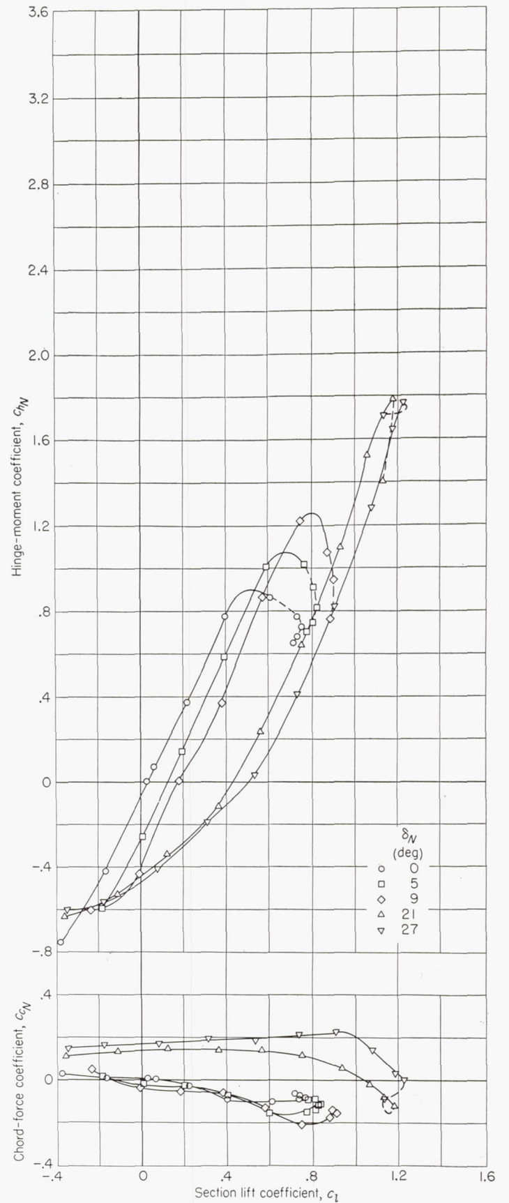
(a) Plain leading-edge flap.
