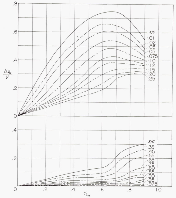
FIGURE 26.—Variation of incremental-additional-velocity ratio with additional lift coefficient.
