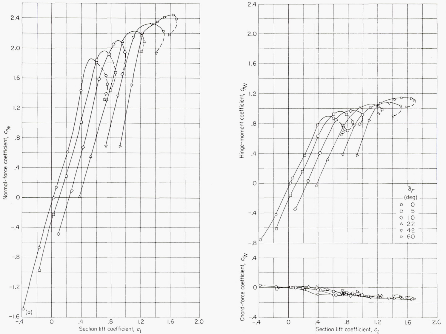
(a) Plain leading-edge flap.
