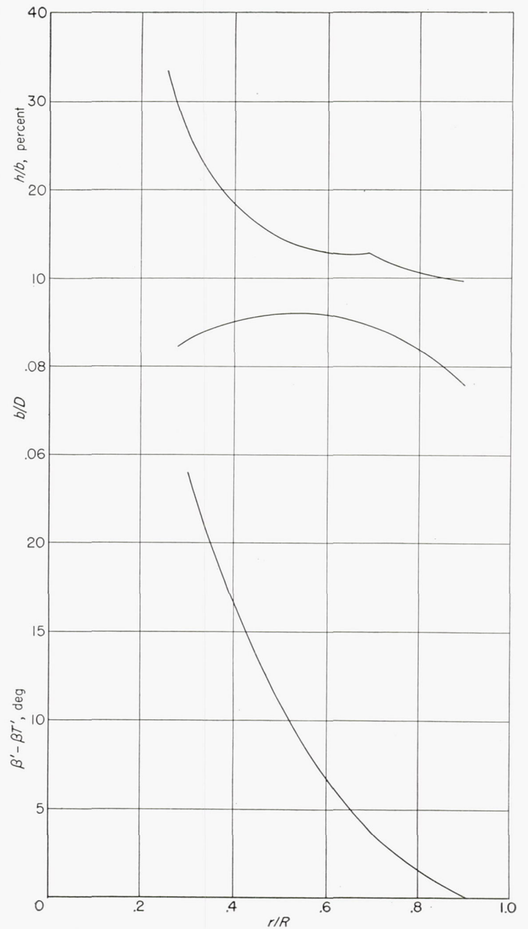
FIGURE 10.—Blade-form curves for four-bladed, one-piece propeller used on ARF Stinson (configuration 3). D , diameter of propeller; R , tip radius; r , radius of element; b , width (chord) of element; h , maximum thickness of element; \beta' , pitch angle of element; \beta T' , pitch angle of tip element.
