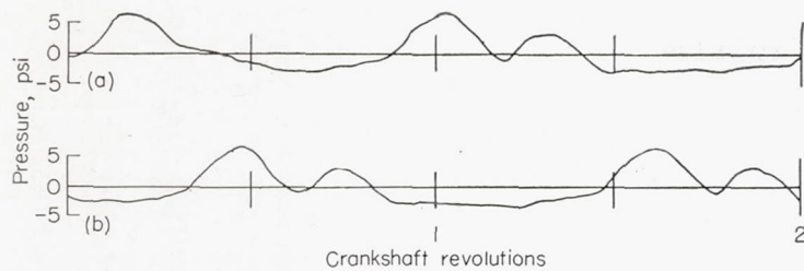
(a) Variation of sound pressure measured in the 3-cylinder exhaust of the test helicopter.
