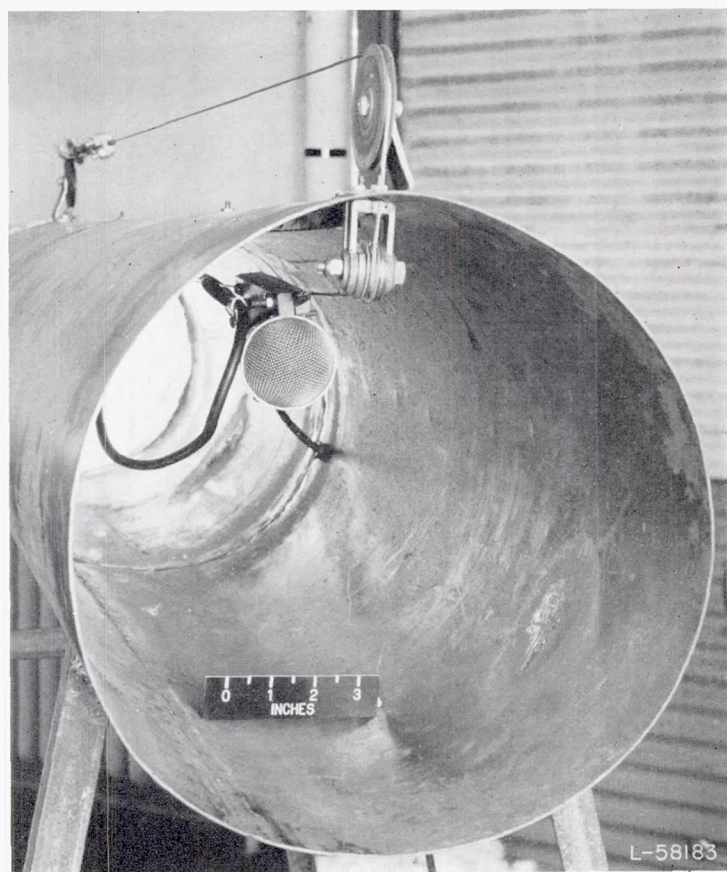
FIGURE 6.—Movable-microphone arrangement in the 12-inch tailpipe.
