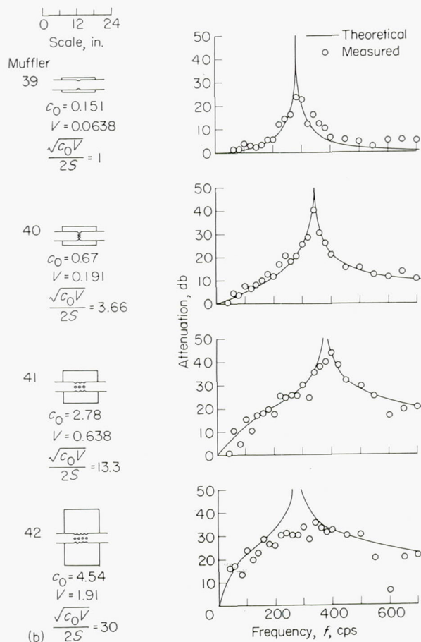
(b) Effect of varying \frac{\sqrt{c_0 V}}{2S} . Equation (B10).
