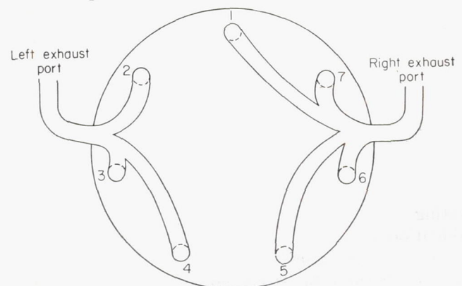
FIGURE 30.—Schematic drawing of helicopter-engine-exhaust system. Firing order: 1, 3, 5, 7, 2, 4, 6.
