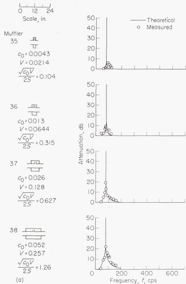
(a) Effect of varying the attenuation parameter \frac{\sqrt{c_0 V}}{2S} with the resonance parameter \sqrt{\frac{c_0}{V}} constant. Equation (B10).
