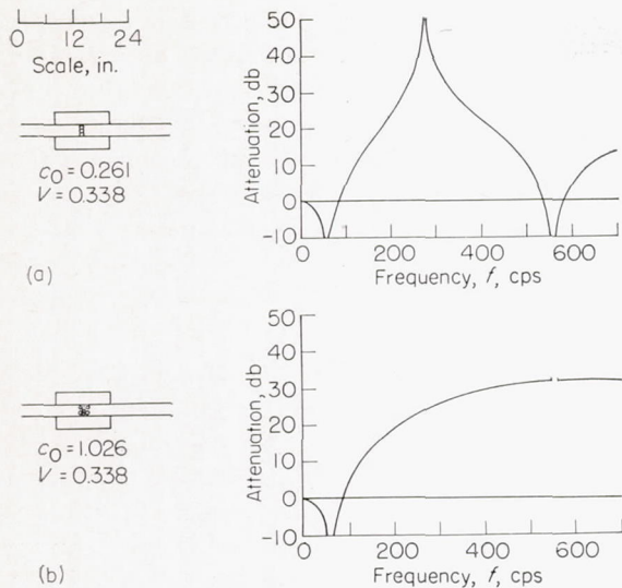
(a) Single-resonator muffler with tailpipe. k_r l_t = 0.48\pi . (See also table IV.)
