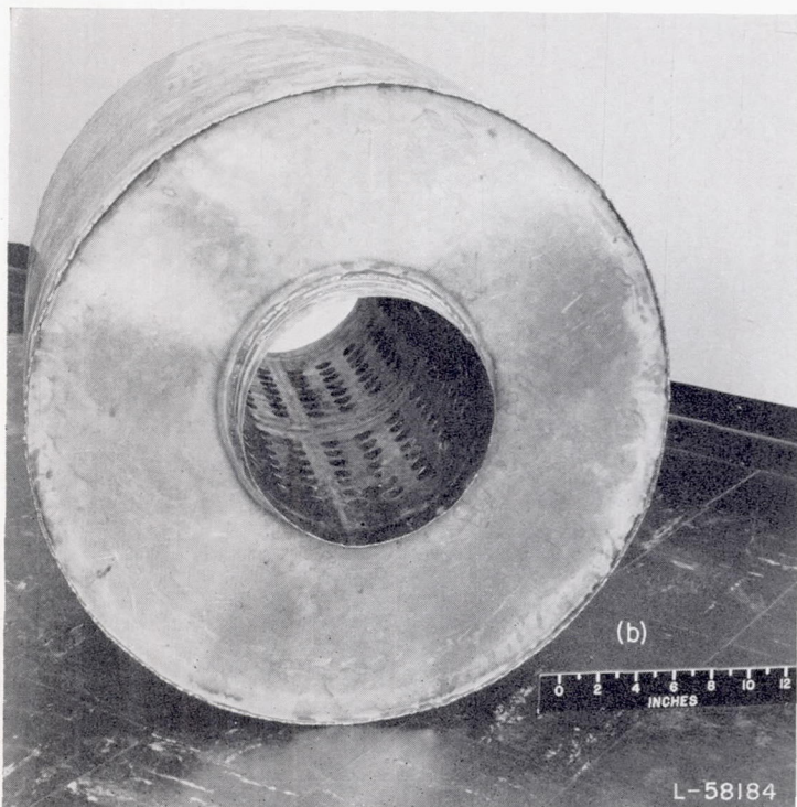
(b) Central-tube diameter, 12 inches; muffler 74.
