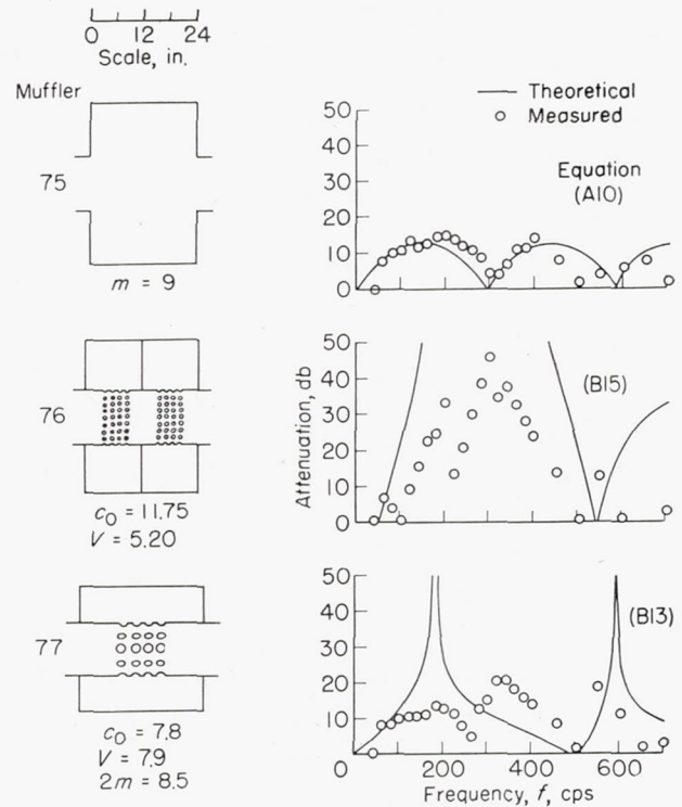
FIGURE 17.—Mufflers for large-diameter (12 in.) exhaust pipes.
