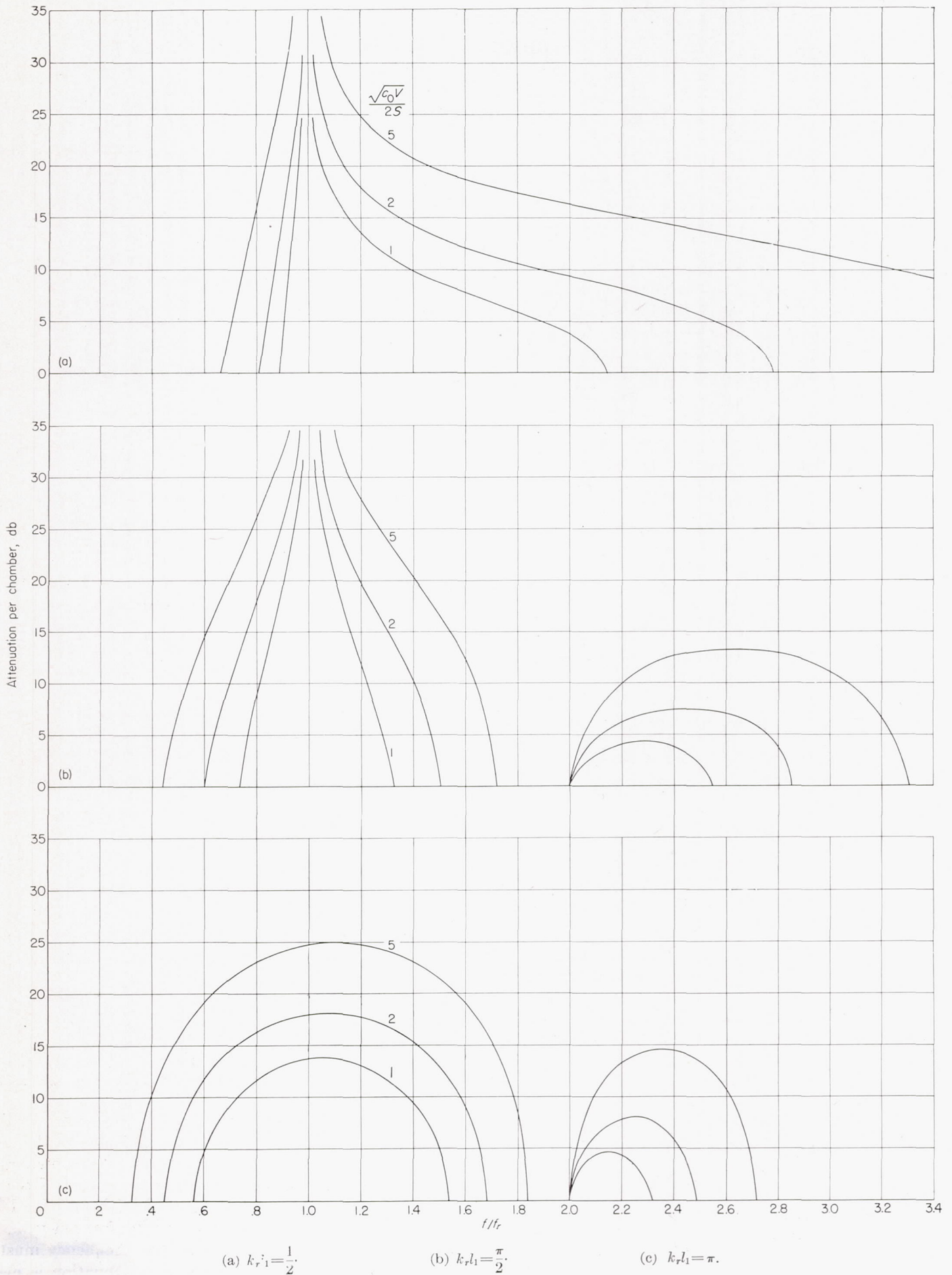
FIGURE 24.—Multiple-chamber-resonator design curves.
