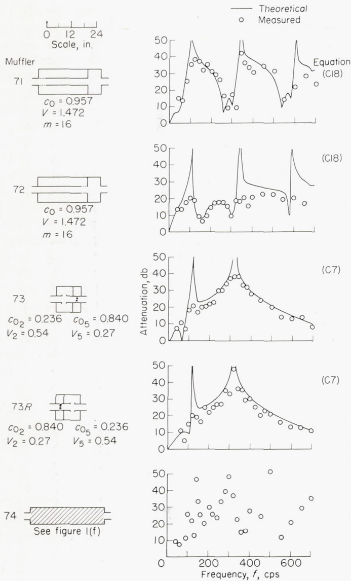
FIGURE 16.—Combination mufflers.
