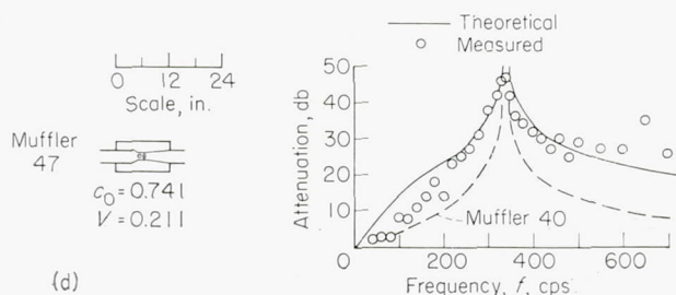
(d) Effect of venturi-shape contraction in central tube. Equation (B10).
