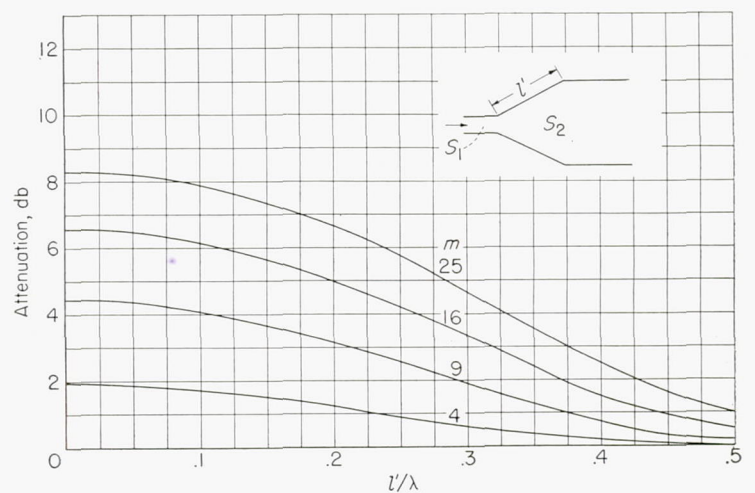
FIGURE 10.—Acoustical characteristics of truncated cone. (See ref. 1, p. 86.)
