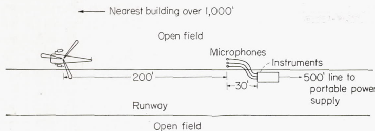
FIGURE 28.—Engine-test arrangement.
