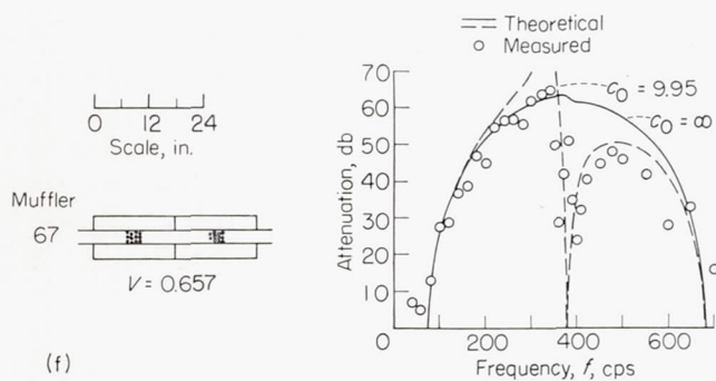
(f) Effect of setting resonant frequency equal to first pass frequency ( k_r l_1 = \pi ). Equation (B12) in (B14).
