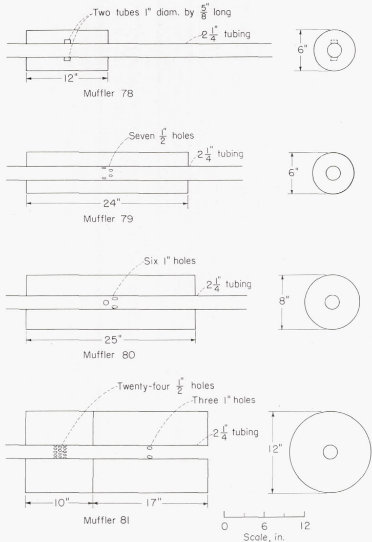
FIGURE 19.—Sketches of muffler-tailpipe combinations tested.
