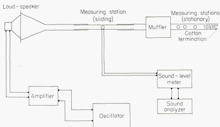
FIGURE 3.—Schematic diagram of experimental apparatus for infinite tailpipe investigation.
