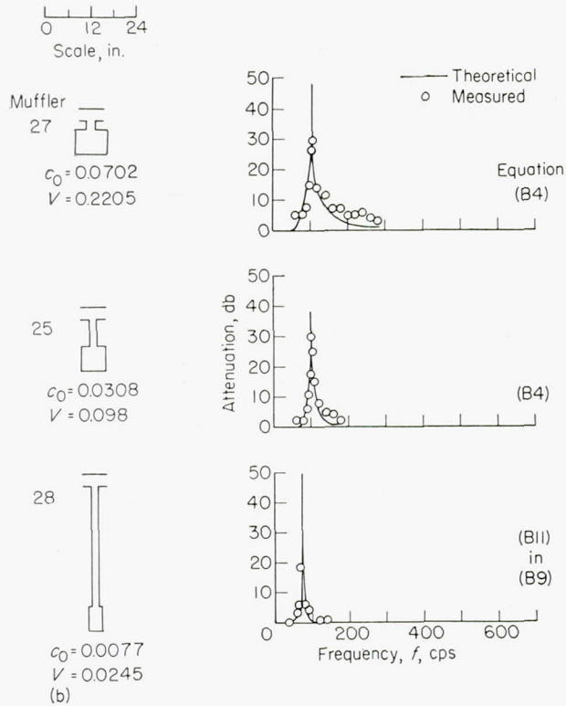
(b) Effect of varying volume V and conductivity c_0 together, with \sqrt{c_0/V} constant.
