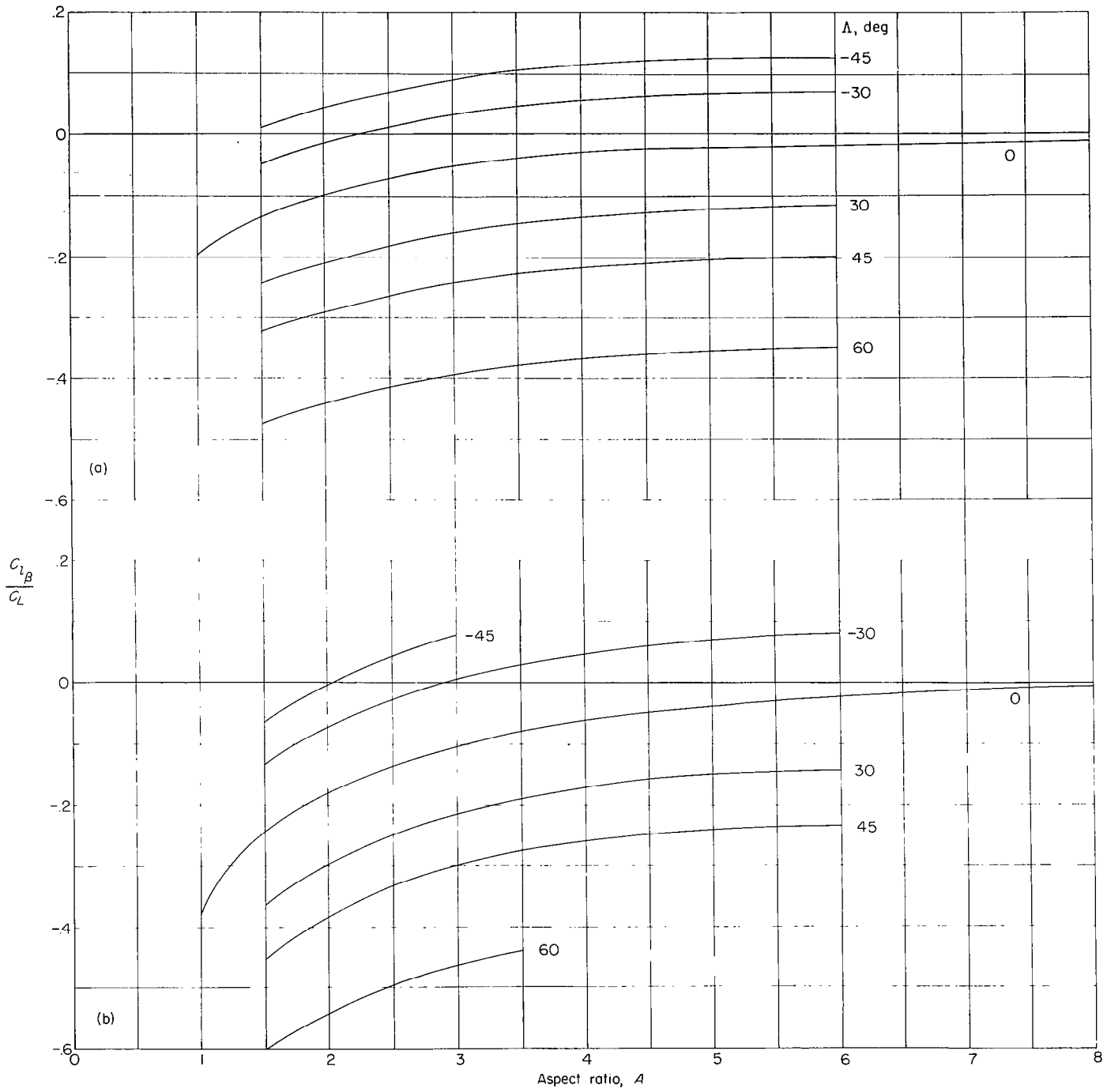
FIGURE 7.—Variation of \frac{C_{l_B}}{C_L} with aspect ratio, taper ratio, and sweep.
