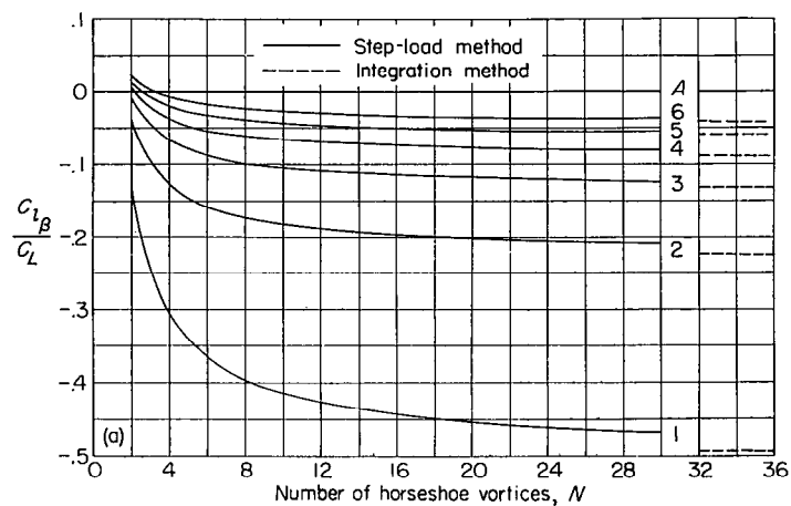
FIGURE 13.—Effect of N on estimated value of \frac{C_{i\beta}}{C_L} .
