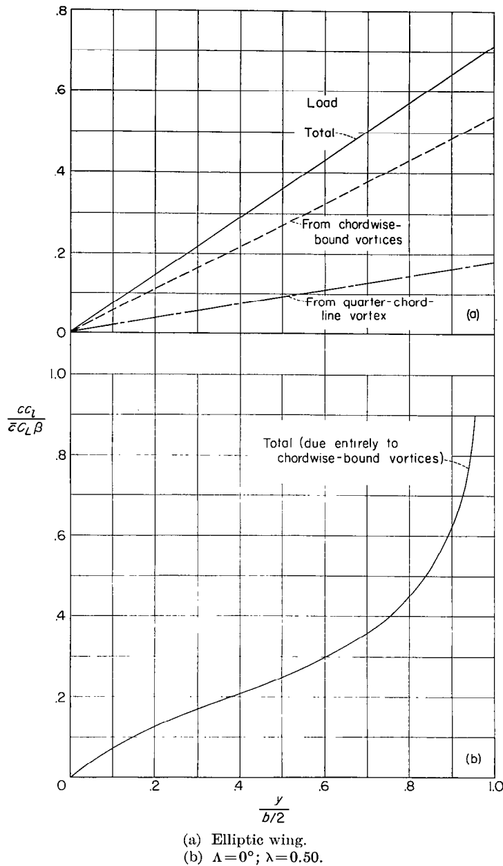
FIGURE 5.—Estimated span load due to sideslip for several plane wings. A = 4.5 .
