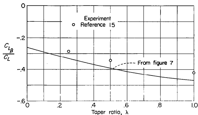
FIGURE 12.—Comparison of experimental and calculated effect of \lambda on \frac{C_{i\beta}}{C_L} . A=2.61 ; \Lambda=45^\circ .
