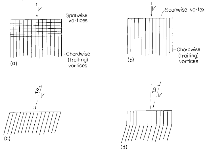
(a) General arrangement for zero sideslip. (b) Lifting-line-theory arrangement for zero sideslip. (c) Blenk's arrangement (ref. 8) for sideslip. (d) Weissinger's arrangement (ref. 1) for sideslip.
