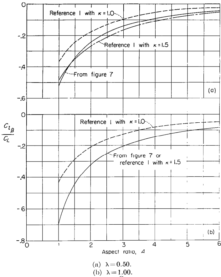
FIGURE 9.—Comparison of values of \frac{C_{iB}}{C_L} from figure 7 with theoretical values from reference 1. \Lambda = 0^\circ .
