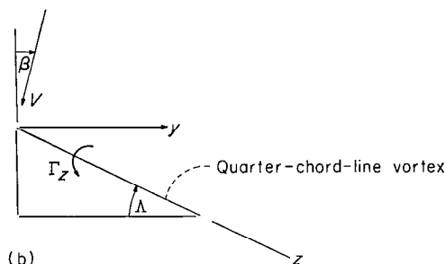
FIGURE 2.—Representation of a wing by the vortex system used in analysis.
