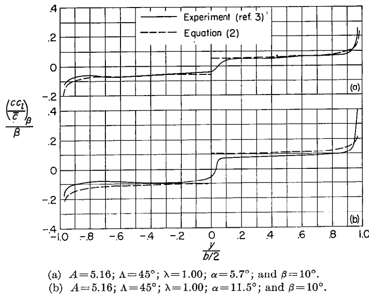
FIGURE 6.—Comparison of experimental and calculated span loads due to sideslip.
