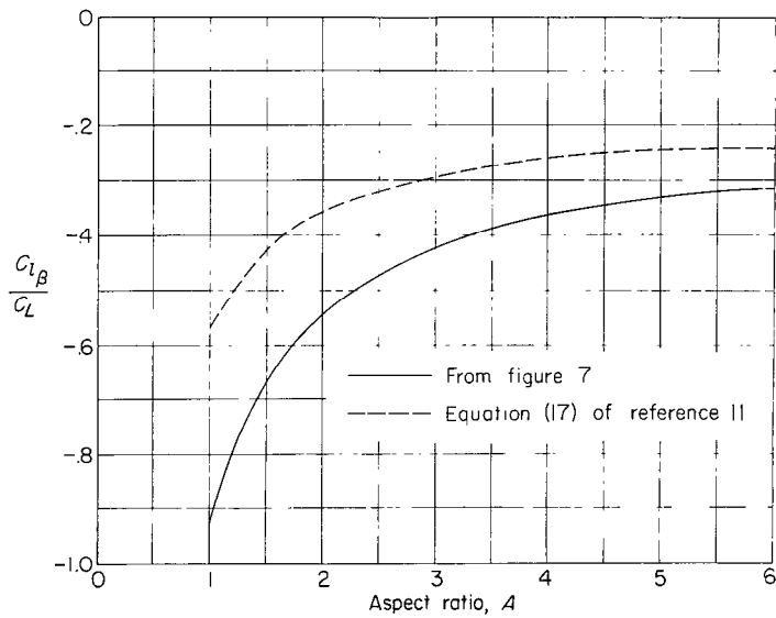
FIGURE 10.—Comparison of values of \frac{C_{iB}}{C_L} from figure 7 with theoretical values from reference 11. \Lambda = 45^\circ ; \lambda = 1.00 .
